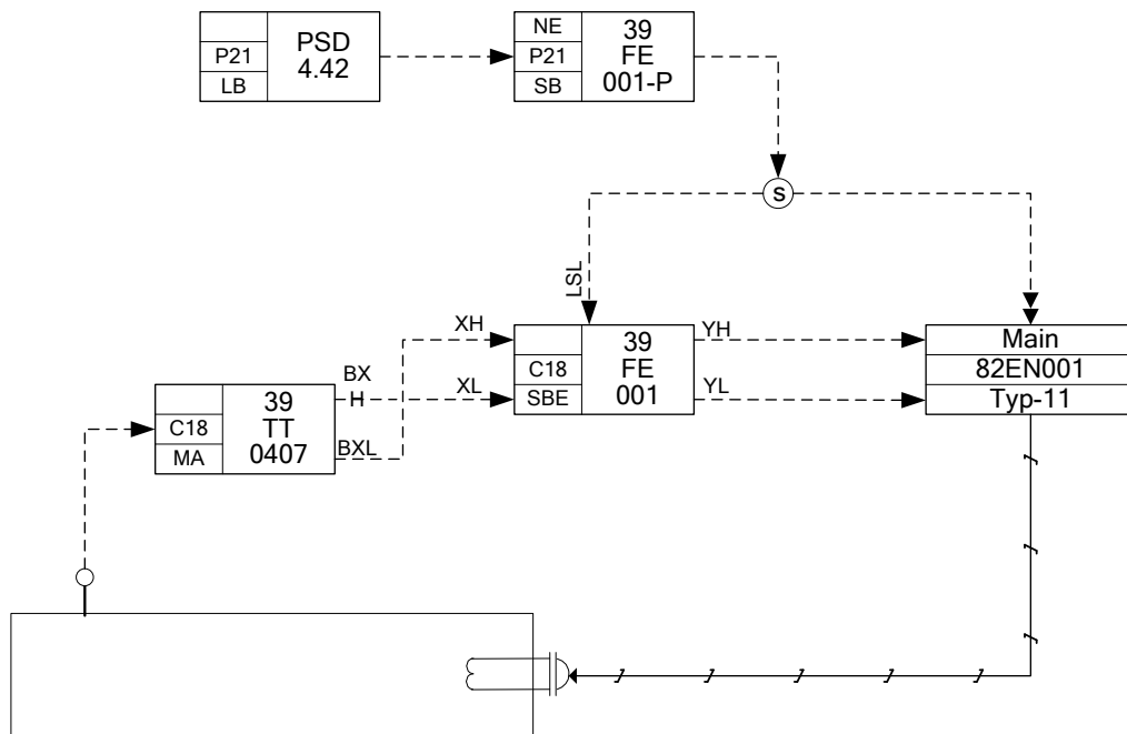
Figure G.2 - Temperature control
