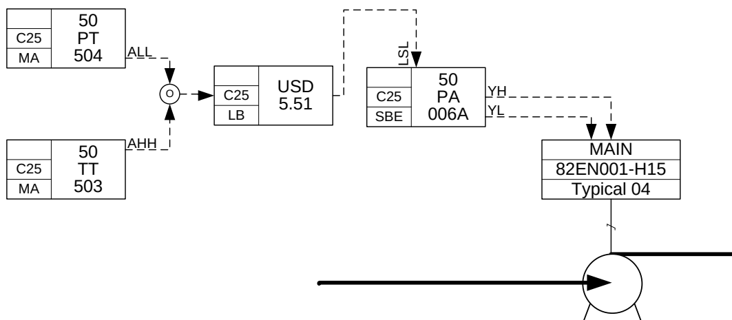
Figure E.36 - Unit shutdown level stop of pump
