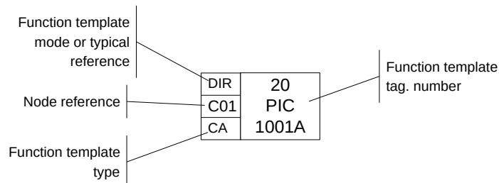
Figure B.1 - The function template symbol
