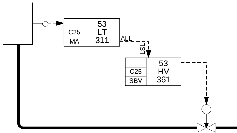
Figure E.24 - Safeguarding of On/Off valve
