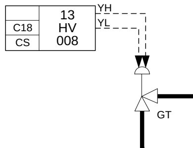
Figure E.18 - Choke valve control
