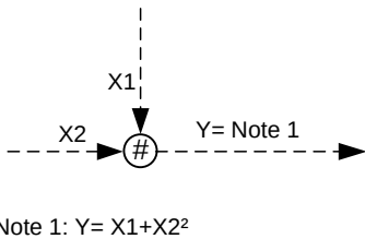
Figure B.8 - Use of the “optional” notation “#”
