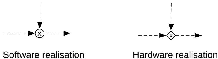
Figure B.6 - Elementary functions symbol
