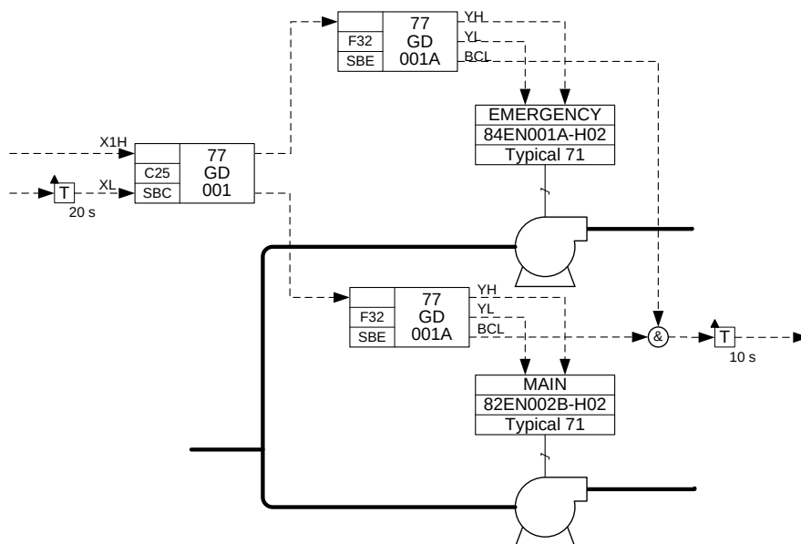
Figure E.46 - Control of multiple fans
