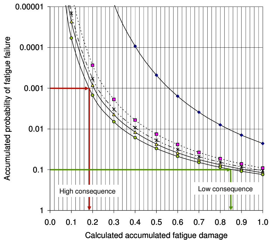
Figure A.21 - Example of accumulated damage at planned first inspections depending on consequence of fatigue failure
