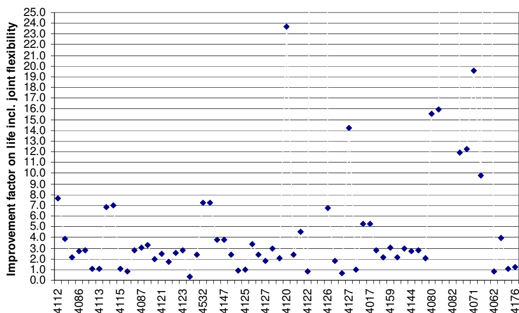
Figure A.5 - Factor on calculated fatigue life when including joint flexibility at horizontal elevation approximately 20 m below water level in a jacket
