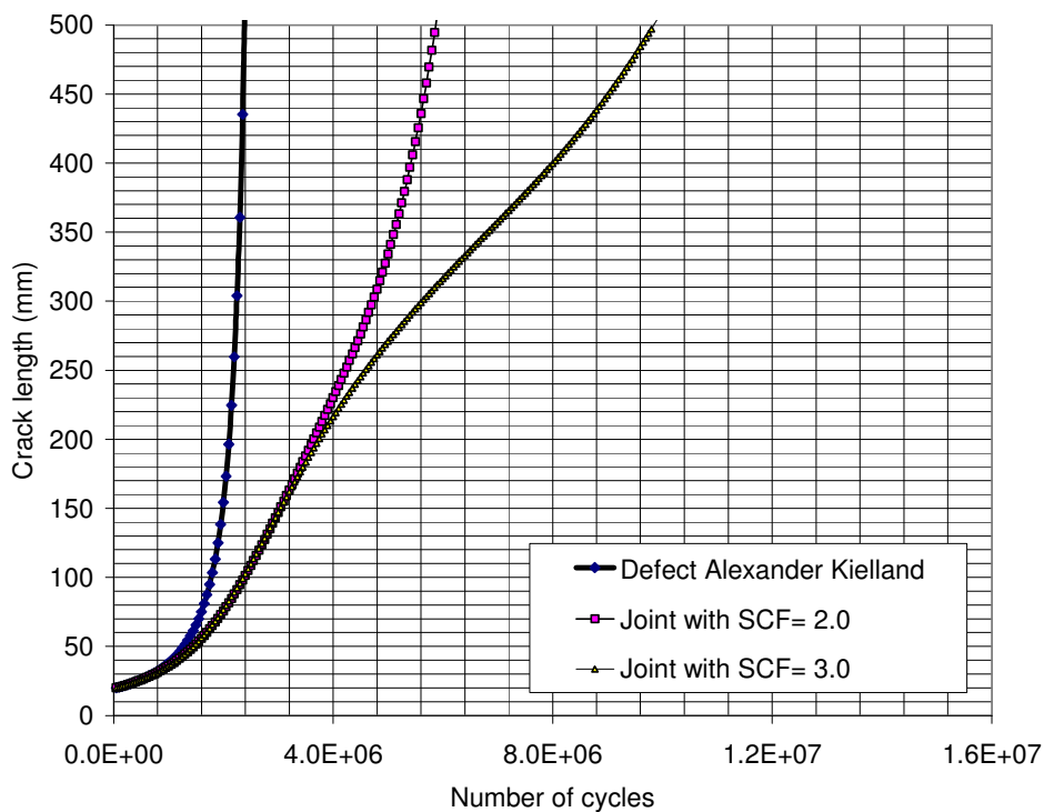
Figure A.9 - Crack growths as function of number of cycles
