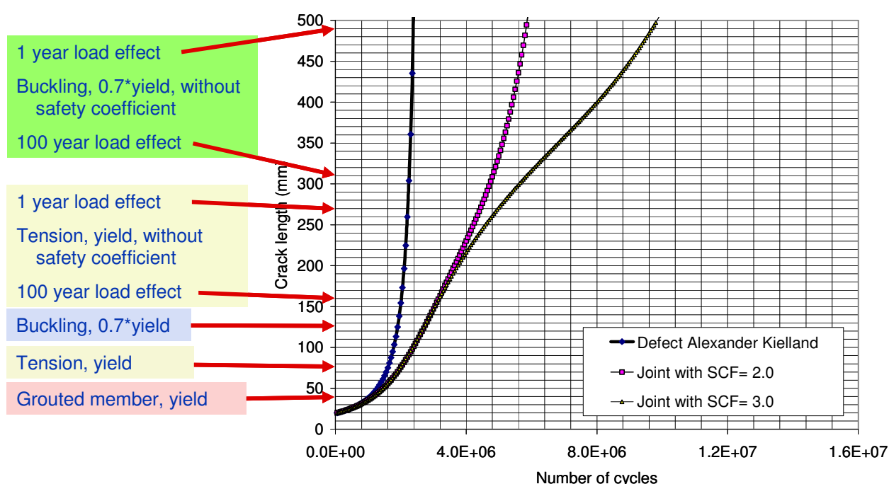
Figure A.11 - Illustration of acceptance criteria depending on assumed load effect
