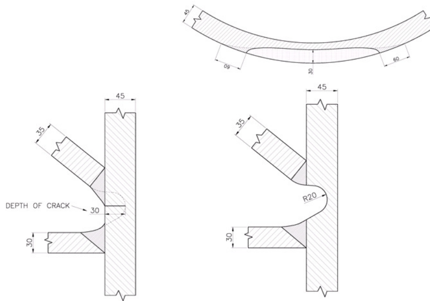
Crack at crown position in K-joint
