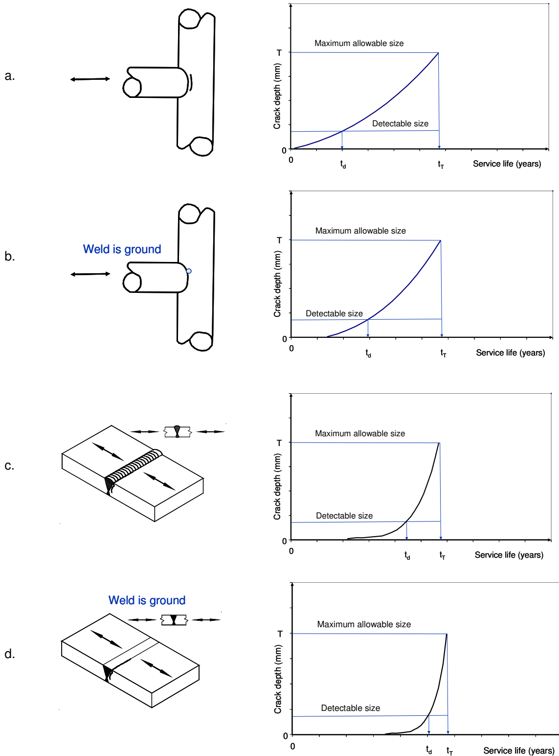
Figure A.23 - Sketch showing difference in crack growth for as welded and ground connections
