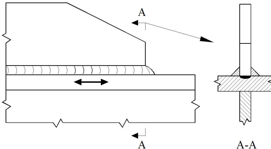
Figure A.14 - Illustration of fatigue crack growing into the member below the weld root (ref. detail 1)
