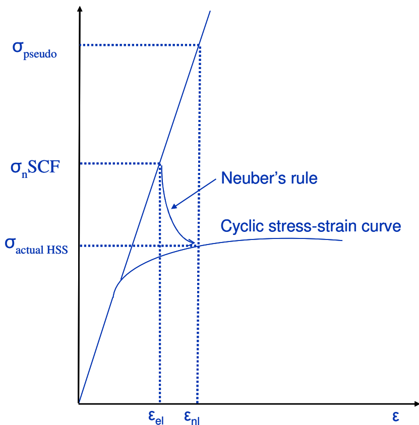
Figure A.18 - The Neuber approach and use of pseudo-elastic stress
