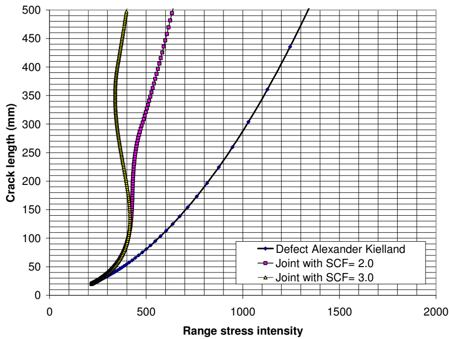
Figure A.7 - Range of stress intensity as function of crack length
