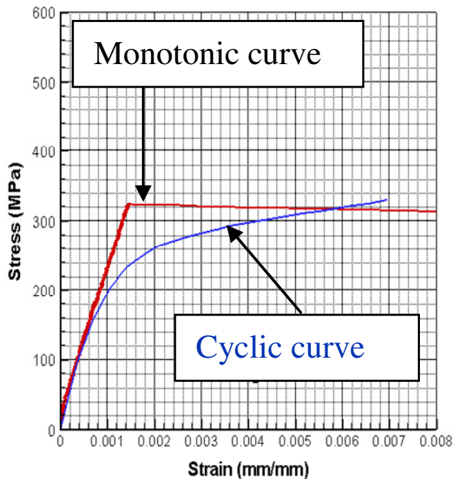
Figure A.17 - Monotonic and cyclic stress-strain curve
