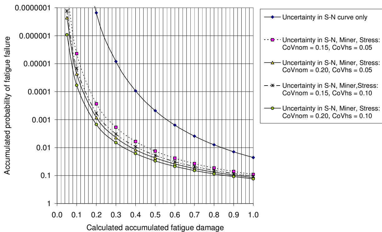
Figure A.20 - Calculated accumulated probability of fatigue failure as function of calculated accumulated fatigue damage
