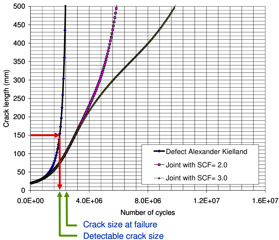
Figure A.10 - Illustration of inspection interval from detectable crack size to failure
