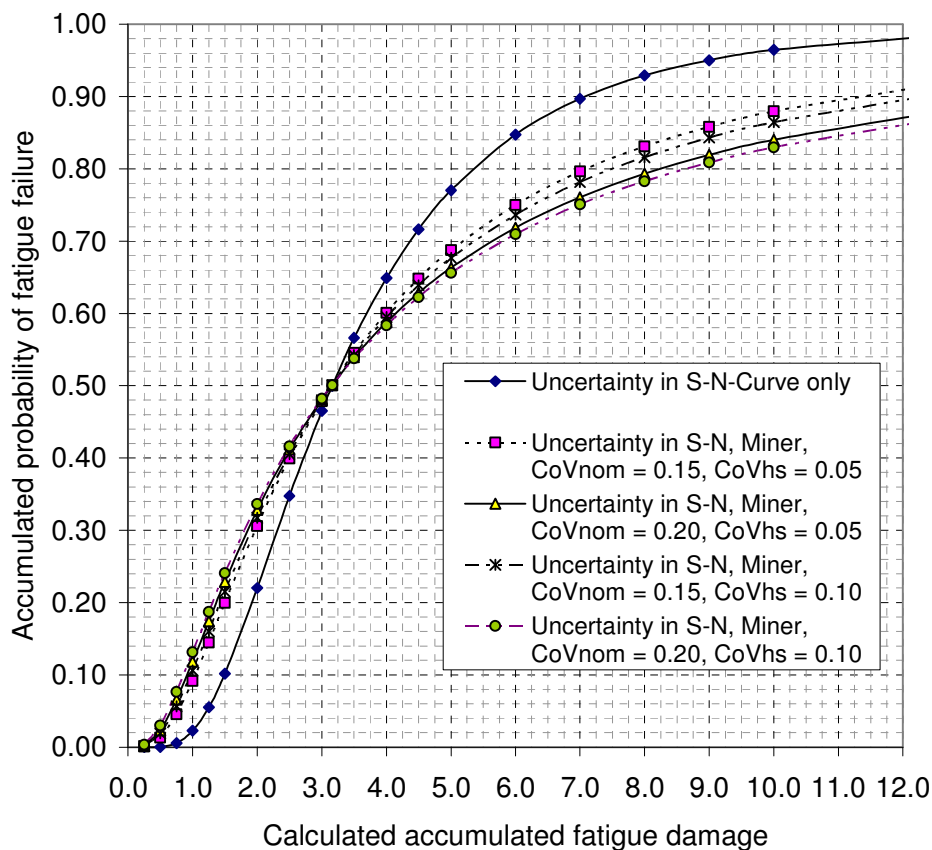
Figure A.19 - Calculated accumulated probability of fatigue failure as function of calculated accumulated fatigue damage
