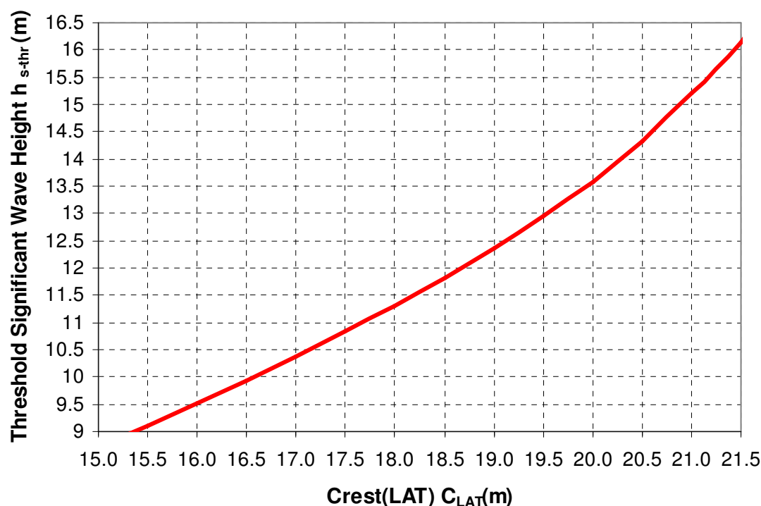
Figure A.3 - Limiting sea-state governed by main safety functions (Southern part of the North Sea)
