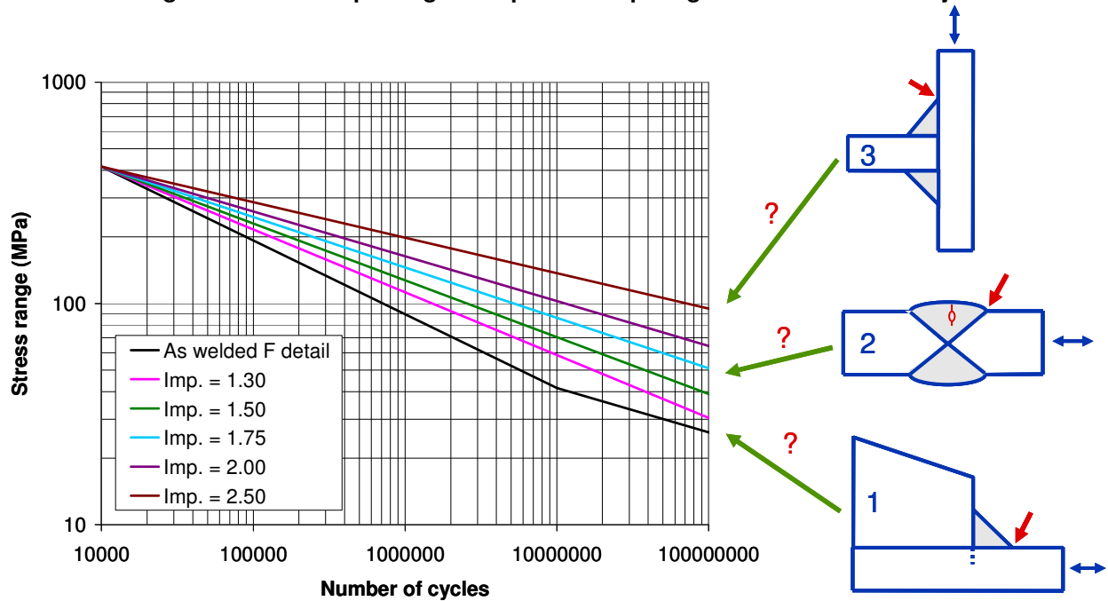
Figure A.13 - Sketch illustrating effect of improvement of welds
