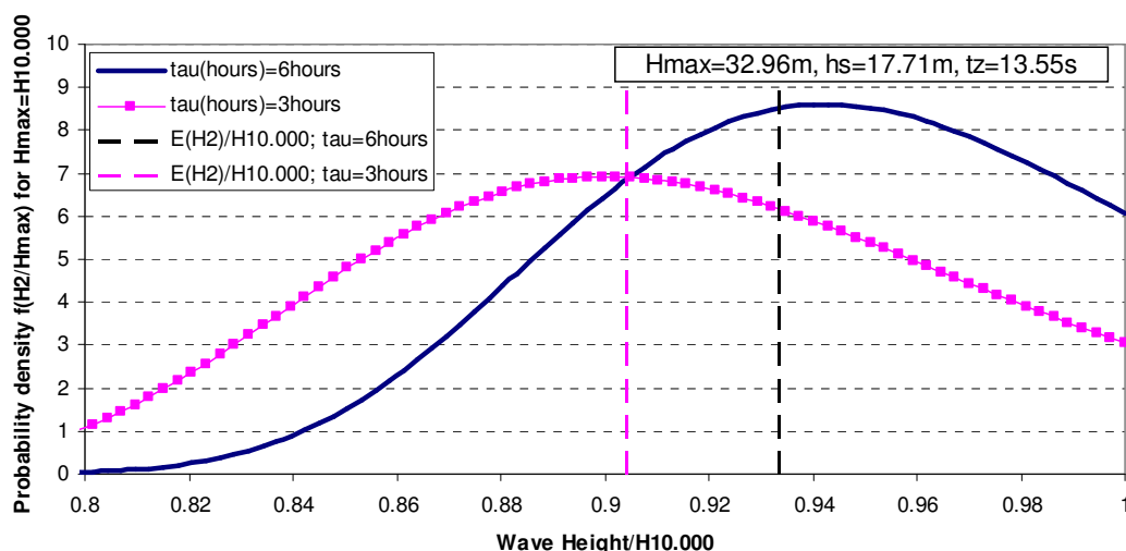
Figure A.16 - Probability density function f(h_2/H_{10\,000}) for the second highest wave in the design storm, assuming H_{\max} = H_{10\,000}
