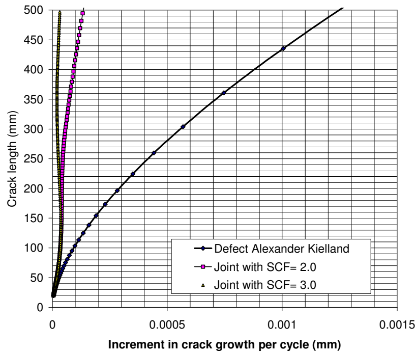
Figure A.8 - Increment in crack growth for different types of joint and crack length
