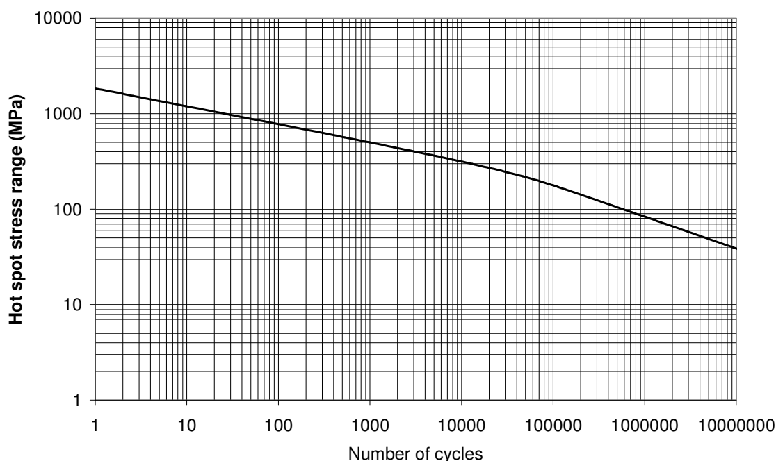
Figure 4 - S-N curve for low cycle fatigue for tubular joint in seawater with cathodic protection
