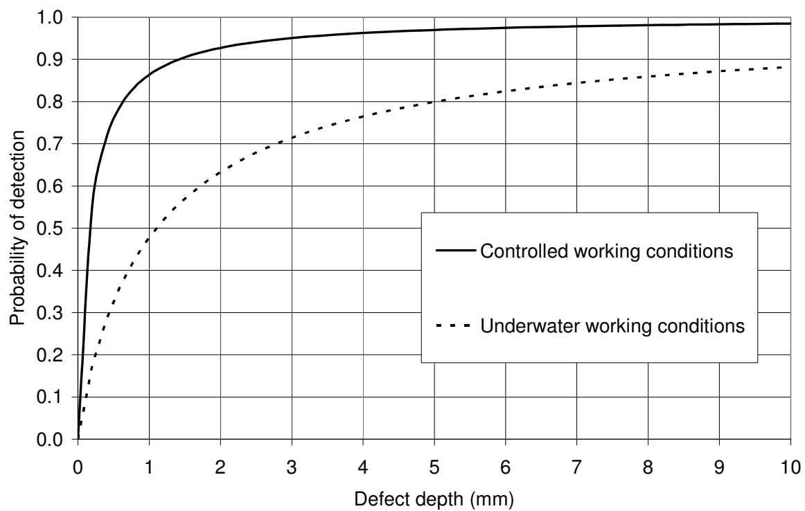
Figure A.22 - Probability of detection curves for EC and MPI
