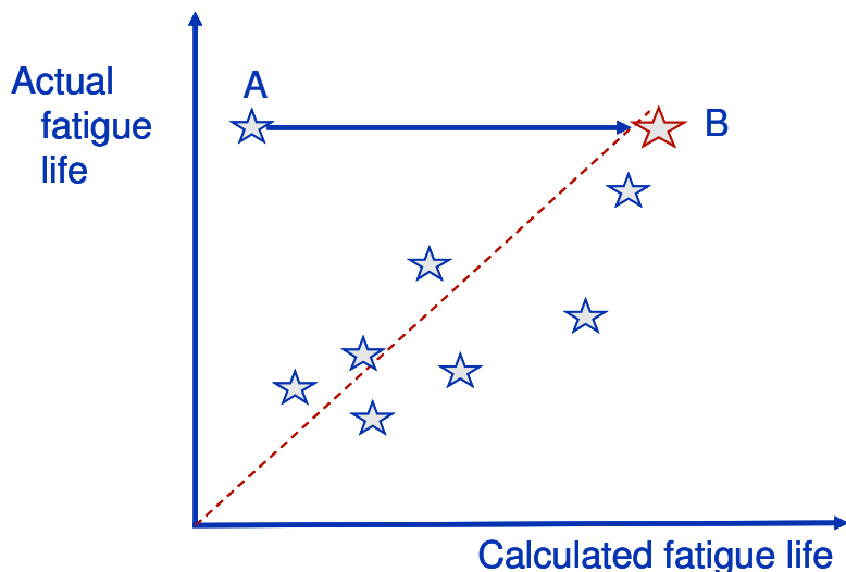
Figure A.4 - Example of calculated life versus actual life
