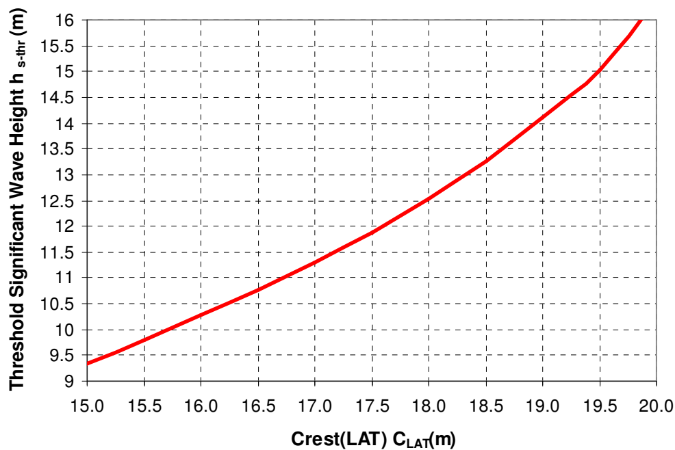
Figure A.1 - Limiting sea-state for unmanning (Southern part of the North Sea)
