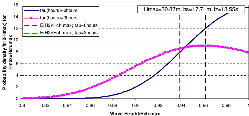
Figure A.15 - Probability density function f(h_2/H_{\text{ch,max}}) for the second highest wave in the design storm assuming H_{\max} = H_{\text{ch,max}} = characteristic largest maximum
