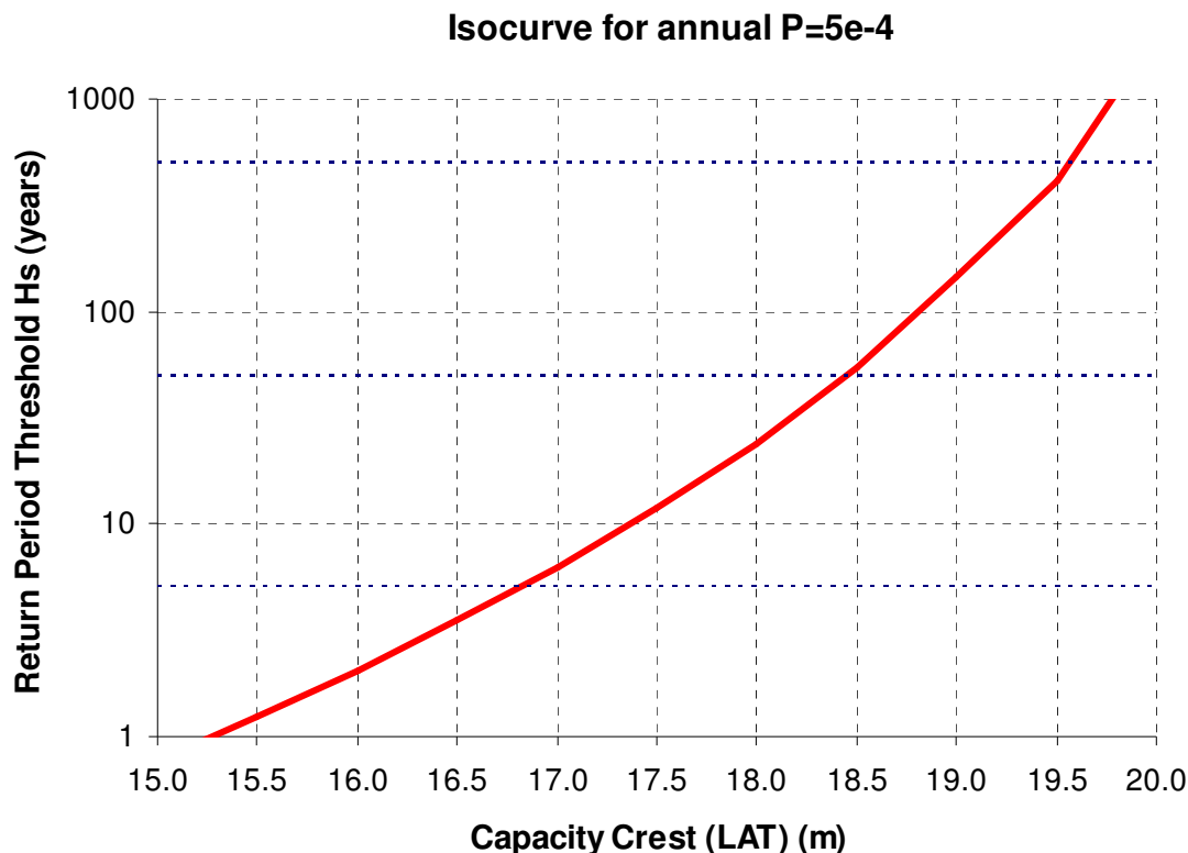
Figure A.2 - Return period for the sea-state triggering the unmanning criterion
