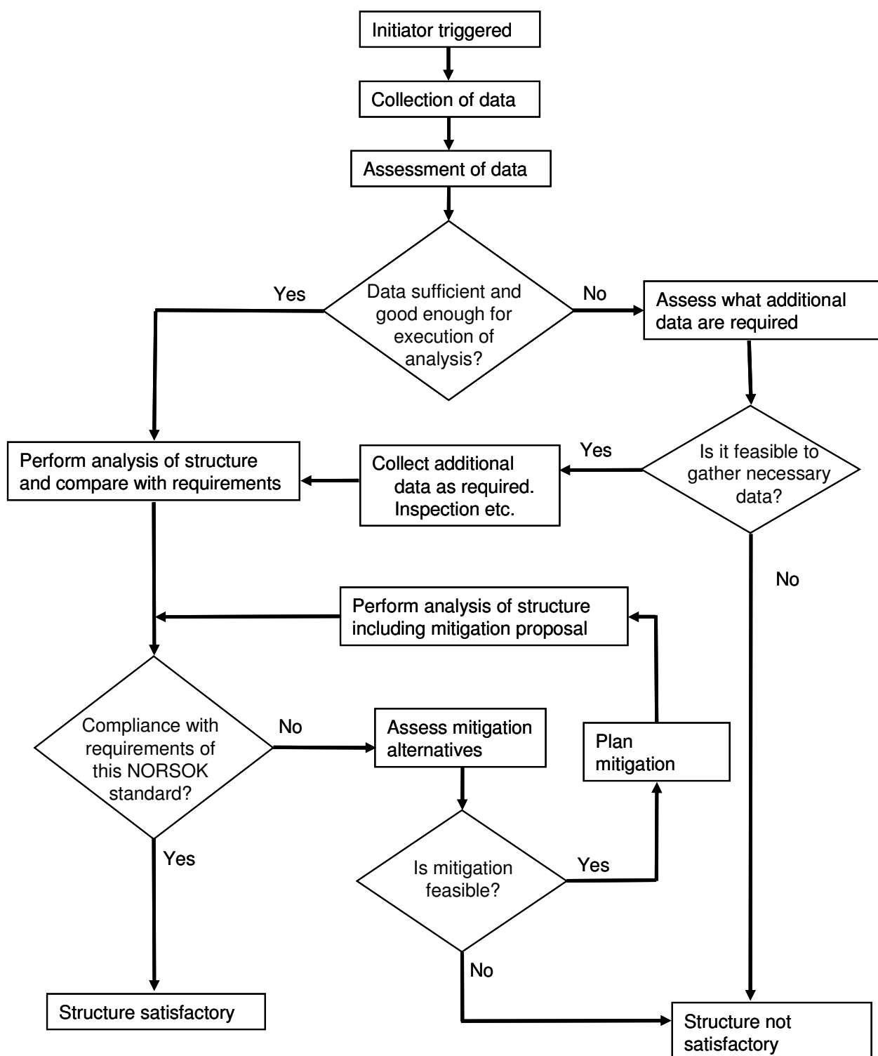
Figure 1 - Flow sheet of the assessment process
