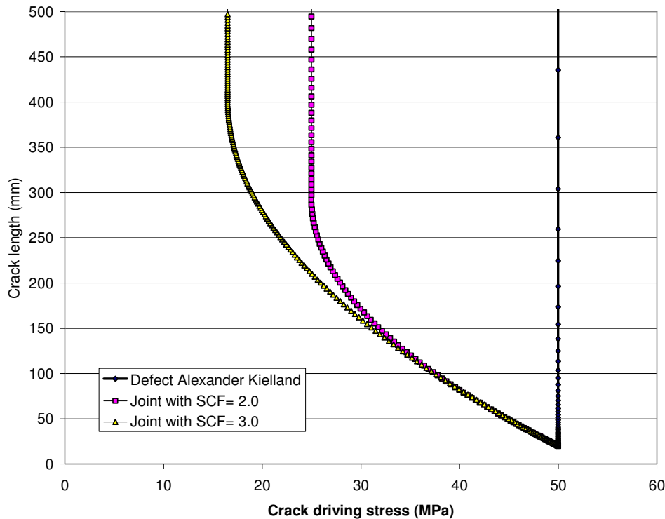
Figure A.6 - Crack driving stress as function of crack length (for illustration)
