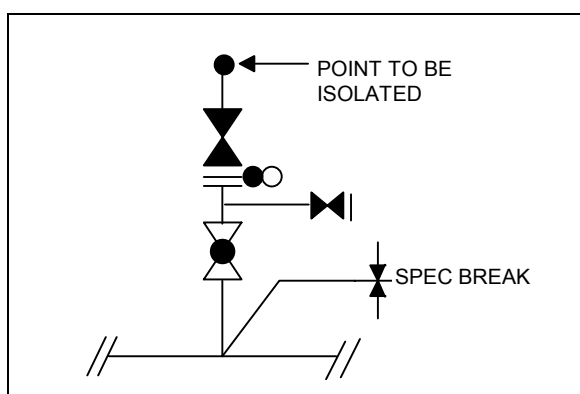
Figure 7: Double block for connection to closed drains.
