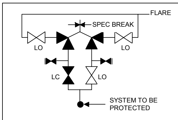
Figure 9: Arrangement for interlocked relief valves (PSV's).
