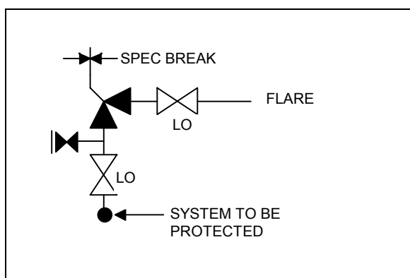
Figure 8: Arrangement for single relief valve (PSV).
