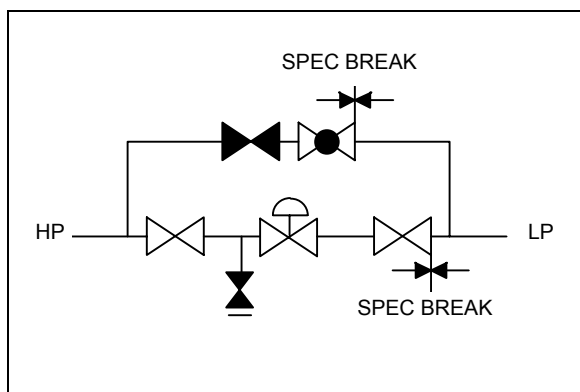
Figure 5: Isolation of control valve having bypass with tight shut off.
