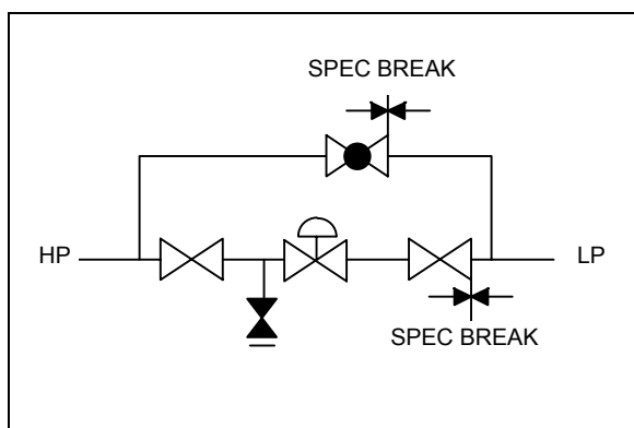
Figure 4: Isolation of control valve having bypass.
