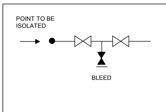
Figure 1: Double block and bleed for process systems
