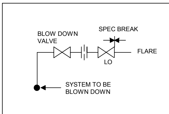
Figure 10: Blow down valve.
