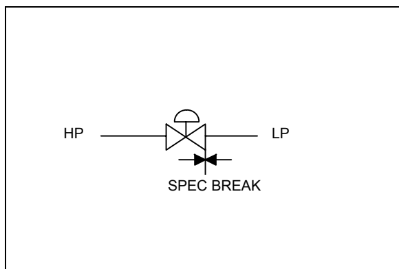
Figure 6: Single control valve on non essential systems (no isolation).
