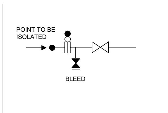
Figure 2: Single block and bleed for process systems
