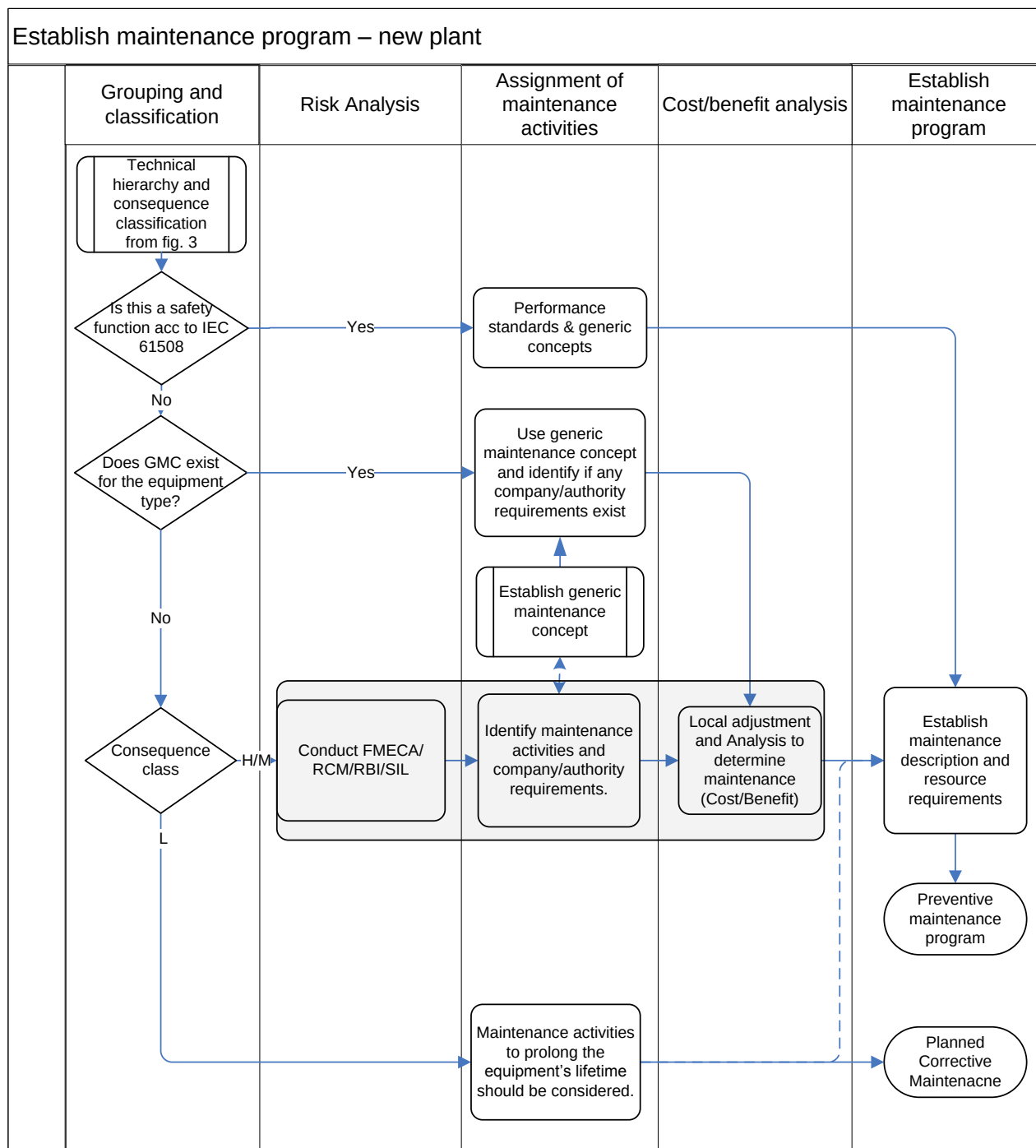
Figure 3 – Establishing maintenance programme for new plants
