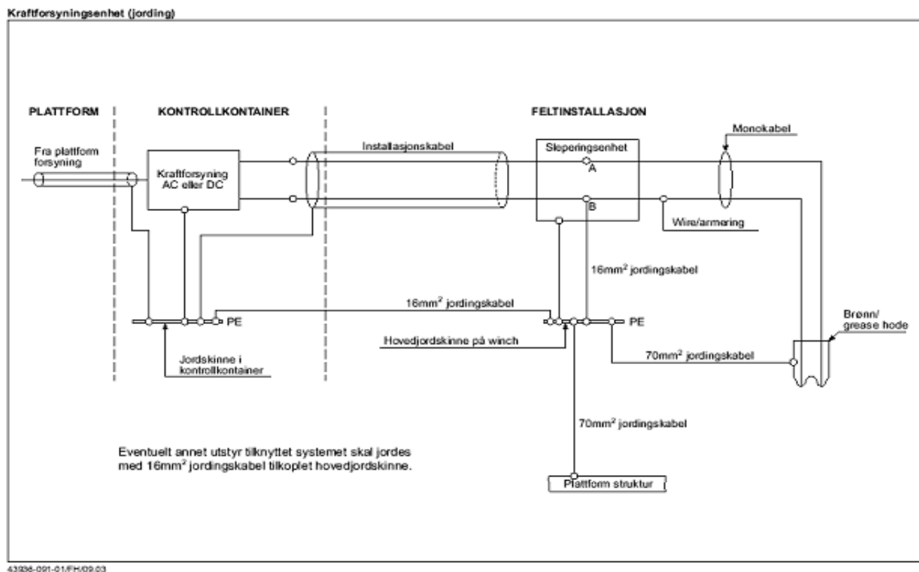
Figure F.2 – Power supply is earthed in slipping unit
