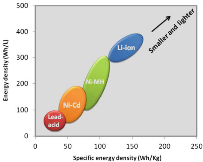
Fig. 1.1 Comparison of the different rechargeable battery technologies in terms of volumetric and gravimetric energy density
