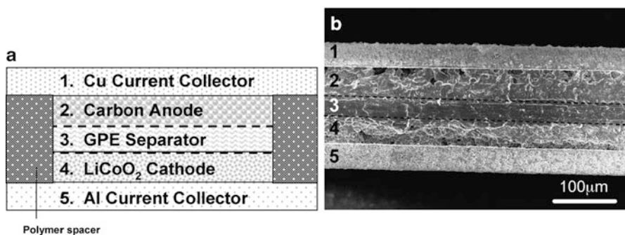
Fig. 10.15 (a) Cross-sectional schematic diagram (not to scale) of a typical lithium-ion microbattery used for this work. (b) Cross-sectional SEM micrograph of a packaged thick-film lithium-ion microbattery. The layers visible (from top to bottom) are (1) Cu current collector, (2) carbon anode, (3) GPE soaked separator, (4) LiCoO 2 cathode and (5) Al current collector. The GPE soaked separator is marked by black dashed lines (Reprinted from [9], Copyright (2011), from Elsevier)
