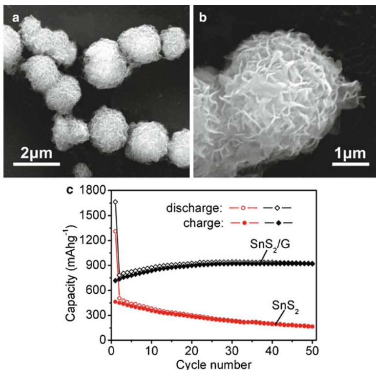
Fig. 6.20 (a) and (b) SEM images of SnS 2 /graphene composite and (c) cycling performance of SnS 2 /graphene composite at 100 mA g -1 (Reprinted with permission from Journal of Power Sources, doi:10.1016/j.jpowsour.2011.10 Copyright (2011) Springer)
