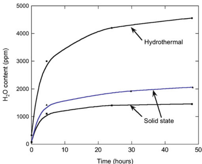
Fig. 8.15 Moisture content of several C- \text{LiFePO}_4 samples, expressed in ppm of \text{H}_2\text{O} with respect to \text{LiFePO}_4 as a function of time exposure in ambient air at 21^\circ\text{C} (55 % relative humidity). The symbols are experimental results. The lines are only guide for the eyes obtained by smooth fit of the data. None of these samples, however, correspond to the HTR and SSR samples investigated (Reprinted with permission from The Royal Society of Chemistry)
