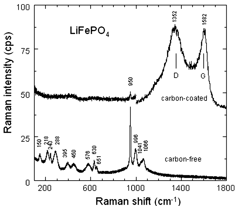
Fig. 8.8 Raman spectra of the carbon-free and carbon-coated \text{LiFePO}_4 samples. Spectra were recorded using the 514.5-nm laser line at the spectral resolution 2\text{ cm}^{-1} . RS features of the \text{LiFePO}_4 bulk material are screened by the carbon deposit for which the G and D bands are observed (Reprinted with permission from Elsevier)
