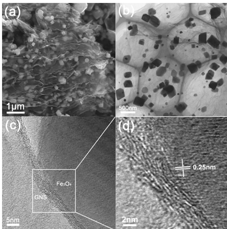
Fig. 6.24 (a) SEM micrograph of the cross-section of graphene/Fe 3 O 4 nanocomposite, (b) TEM and (c) high-resolution TEM micrographs of graphene/Fe 3 O 4 nanocomposite, and (d) detailed interface structure of the square area in (c) (Reprinted with permission from [94]. Copyright 2010 American Chemical Society)
