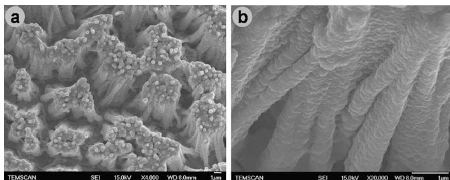
Fig. 10.4 (a) Low- and (b) high-magnification SEM images of Ni nanorod-supported \text{LiCoO}_2 deposits (Reprinted from [14], Copyright (2011), from John Wiley and Sons)
