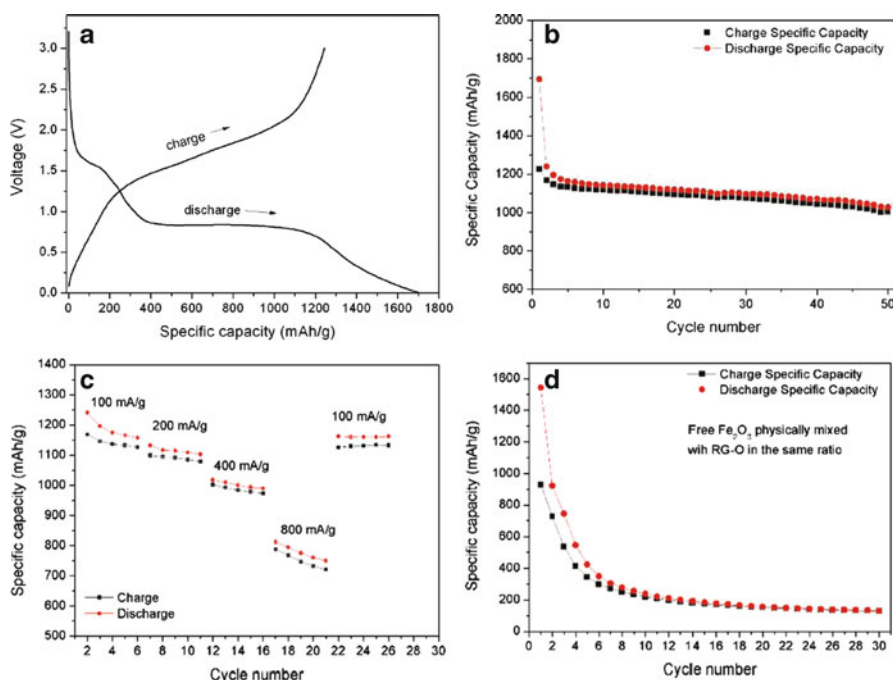
Fig. 6.23 Electrochemical performance of the RGO/Fe 2 O 3 composite. (a) Voltage profile (discharge/charge) of RGO/Fe 2 O 3 composite for the first cycle at the current density of 100 mA g -1 . (b) Cycling performance of RGO/Fe 2 O 3 composite at the current density of 100 mA g -1 . (c) Rate capacity of RGO/Fe 2 O 3 composite between 0.005 and 3.0 V with increasing current density. (d) Capacity retention of free Fe 2 O 3 nanoparticles physically mixed with RGO platelets at a current density of 100 mA g -1 (Reprinted with permission from [88]. Copyright 2011 American Chemical Society)
