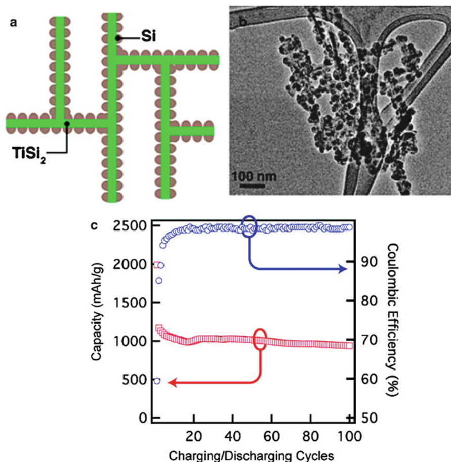
Fig. 3.11 (a) Schematic showing the silicon nanoparticles coated around the \text{TiSi}_2 nanonets. (b) TEM image showing the Si/ \text{TiSi}_2 heteronanostructure. (c) Capacity performance at a current density of 8,400 mA/g (Reprinted with permission from Ref. [63])
