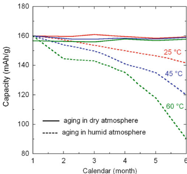
Fig. 8.17 Capacity of the C- \text{LiFePO}_4 (HTR sample)/ \text{LiPF}_6 -EC-DEC/Li cells as a function of time spent in dry atmosphere and in ambient atmosphere (55% relative humidity), at three different temperatures. The temperatures at which the full curves (in dry atmosphere) have been obtained can be distinguished by the fact that they do not overlap and the property that the lower the temperature, the higher the capacity is (Reprinted with permission from Elsevier and The Royal Society of Chemistry)
