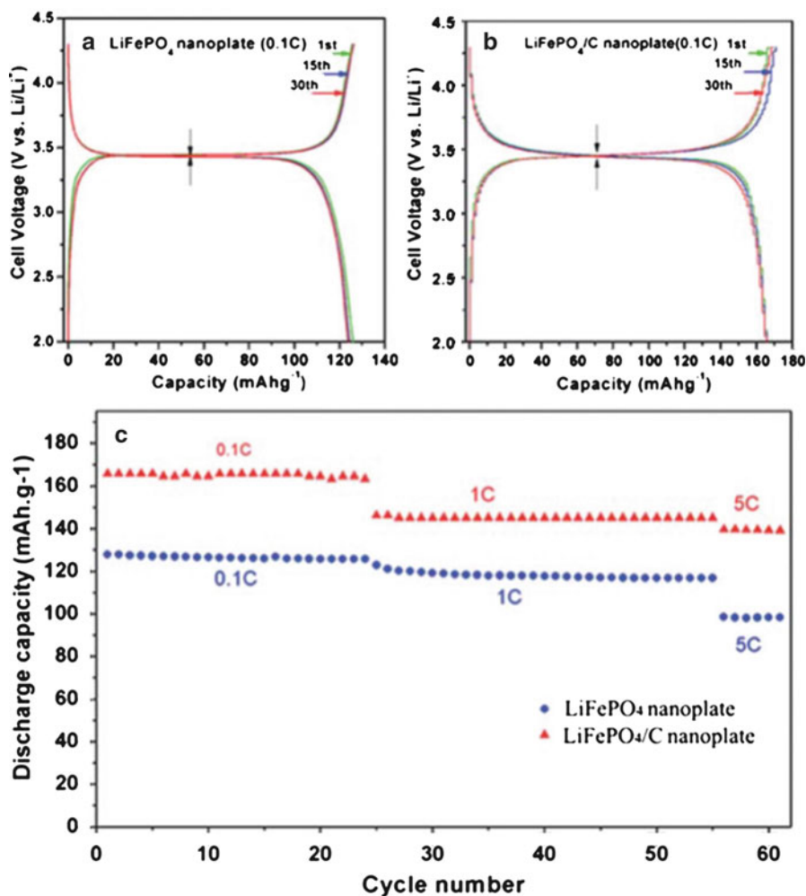
Fig. 7.4 Capacity voltage curves of (a) \text{LiFePO}_4 nanoplates and (b) carbon-coated \text{LiFePO}_4 nanoplates, (c) rate capability of \text{LiFePO}_4 nanoplates (Reproduced from Ref. [17] with permission of The Royal Society of Chemistry)
