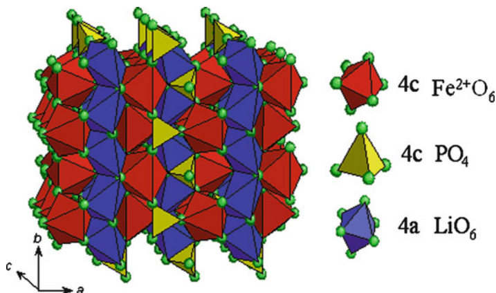
Fig. 8.3 Crystal structure of LiFePO 4 olivine. Corner-shared FeO 6 octahedra are linked together in the bc -plane, while LiO 6 octahedra form edge-sharing chains along the b -axis. The tetrahedral PO 4 groups bridge neighboring layers of FeO 6 octahedra by sharing a common edge with one FeO 6 octahedra and two edges with LiO 6 octahedra
