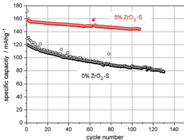
Fig. 9.3 Capacity versus charge–discharge cycles of the \text{Li}/\text{P}(\text{EO})_{20}\text{LiClO}_4 + 5\% \text{ S-ZrO}_2/\text{LiFePO}_4 battery and of the \text{Li}/\text{P}(\text{EO})_{20}\text{LiClO}_4/\text{LiFePO}_4 battery. Temperature, 90^\circ\text{C} ; rate, C/5 , corresponding to a current density of 0.20 \text{ mA cm}^{-2} for the \text{S-ZrO}_2 electrolyte battery and of C/7 ( 0.16 \text{ mA cm}^{-2} ) for the ceramic-free electrolyte battery. The capacity values are referred to the cathode (Reprinted from [26], Copyright (2011), from Elsevier)
