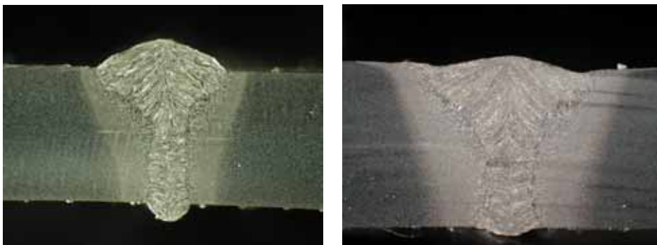
Figure 2.18. Typical cross-sections of hybrid welds in 6 mm mild steel with a \text{CO}_2 laser and MAG. Laser power 4.8 kW, distance D_{LA} 3 mm, welding speed 1.2 m/min, arc current 180–230 A, arc voltage 32–35 V. (Fellman, 2002)
