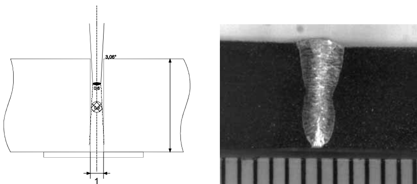
Figure 5.1. The set-up and cross-section of the weld made by the optimal parameter combination received from the single pass TAGUCHI experiments with filler wire. The welding speed 0.6 m/min. Weld OPTI 2. in Appendix 1.
