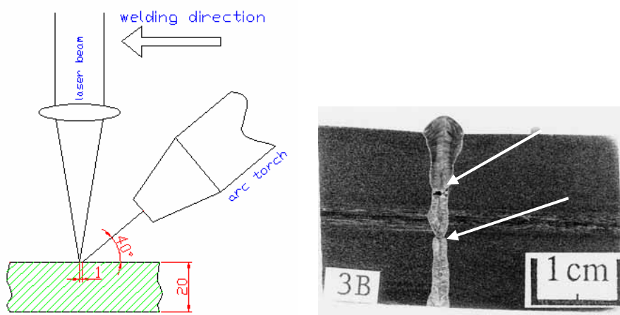
Figure 4.25. The set-up condition and the cross-section of the weld with a thickness of 20 mm, testpiece 3B. The defects are pointed out with arrows. Parameters in Appendix 5.
