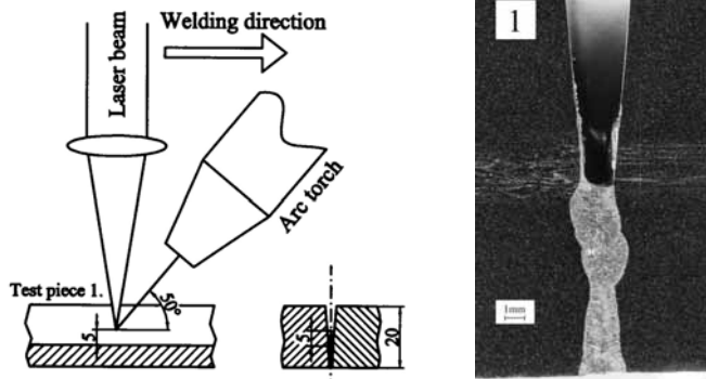
Figure A7-1. The set-up and cross-section of testpiece 1. in the TAGUCHI experiments for the first filling pass with hybrid welding. Parameters in Appendix 4.
