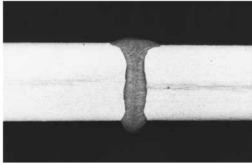
Figure 4.5. The set-up and cross-section of the hybrid weld with a thickness of 6.7 mm. Other parameters: Laser power 3 kW, air gap 1 mm, welding speed 0.9 m/min and filler wire feed 12.5 m/min.
