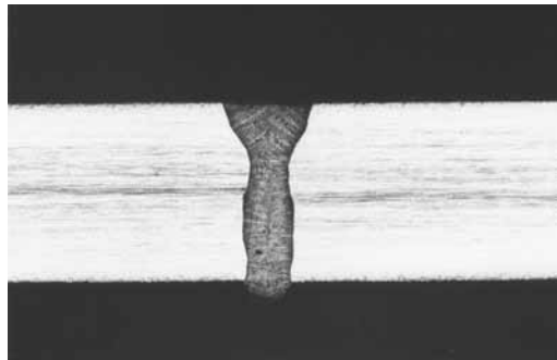
Figure 4.6. The set-up and cross-section of the hybrid weld with a thickness of 6.8 mm. Other parameters: Laser power 3 kW, air gap 1 mm, welding speed 0.9 m/min and filler wire feed 12.5 m/min.
