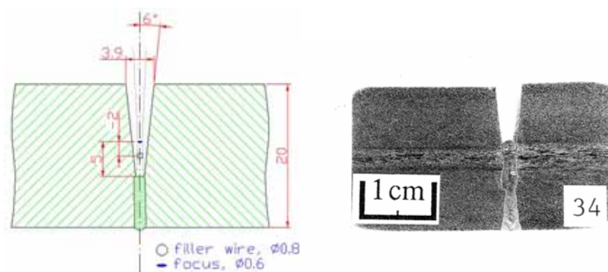
Figure 4.9. The set-up and cross-section of the first filling weld, testpiece 3.4. Parameters in Appendix 2.
