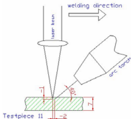
Figure 4.6. The set-up and cross-section of the hybrid weld with a thickness of 6.8 mm. Other parameters: Laser power 3 kW, air gap 1 mm, welding speed 0.9 m/min and filler wire feed 12.5 m/min.
