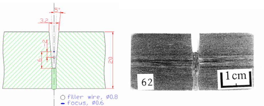
Figure 4.11. The set-up and cross-section of the first filling weld, testpiece 6.2. Parameters in Appendix 2.
