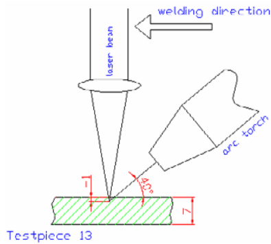
Figure 4.5. The set-up and cross-section of the hybrid weld with a thickness of 6.7 mm. Other parameters: Laser power 3 kW, air gap 1 mm, welding speed 0.9 m/min and filler wire feed 12.5 m/min.
