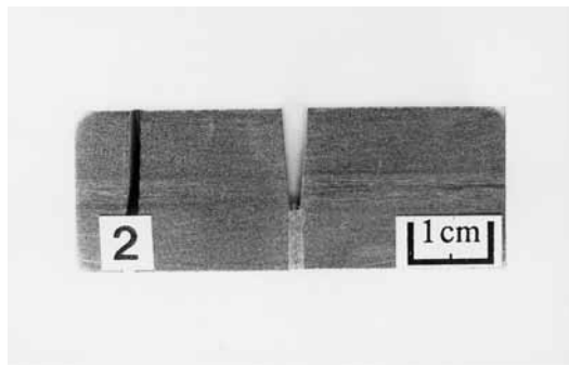
Figure 4.7. The groove geometry and the root weld with acceptable quality. Parameters in Table 3.4.
