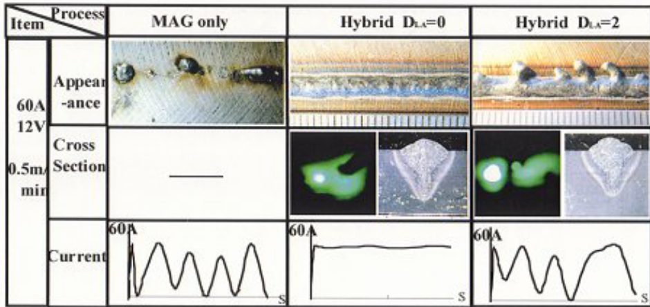
Figure 2.15. Comparison of the weld bead, cross-section and arc stability in hybrid welding with a MAG and CO_2 laser. D_{LA} = Distance between the arc impingement point and a point of the laser beam at the surface of the workpiece. (Kutsuna and Chen, 2002)
