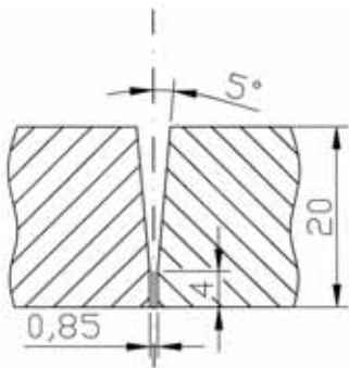
Figure 4.7. The groove geometry and the root weld with acceptable quality. Parameters in Table 3.4.
