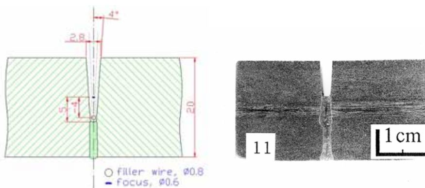
Figure 4.10. The set-up and cross-section of the first filling weld, testpiece 1.1. Parameters in Appendix 2.
