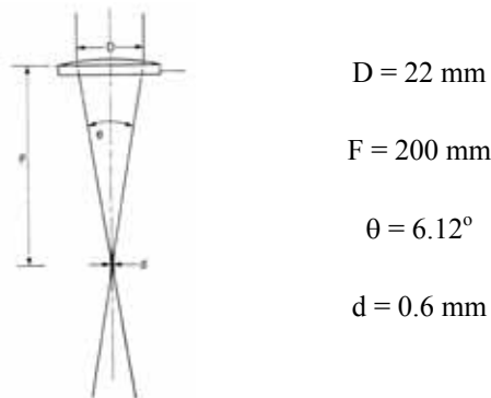
Figure 3.2. Geometry of the focused laser beam used in the experiments.
