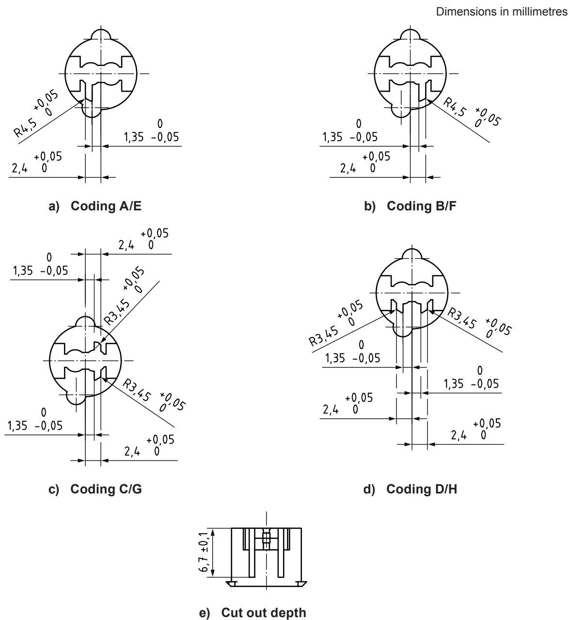
Figure 2 — Dimensions and position of coding keys
