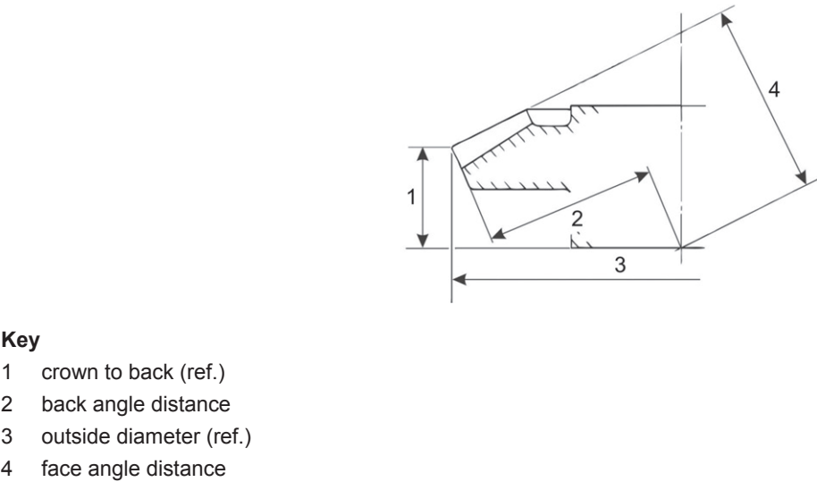
Figure 14 — Method 1 for specifying blank tolerances on bevel gears
