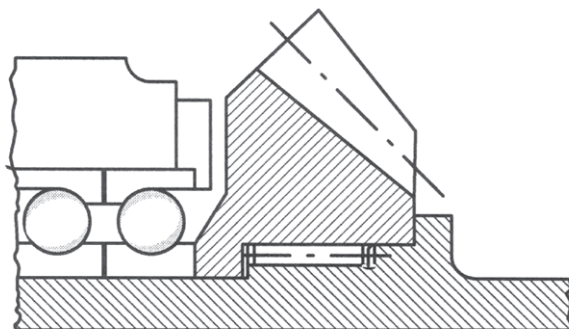
Figure 10 — Spline mounting
