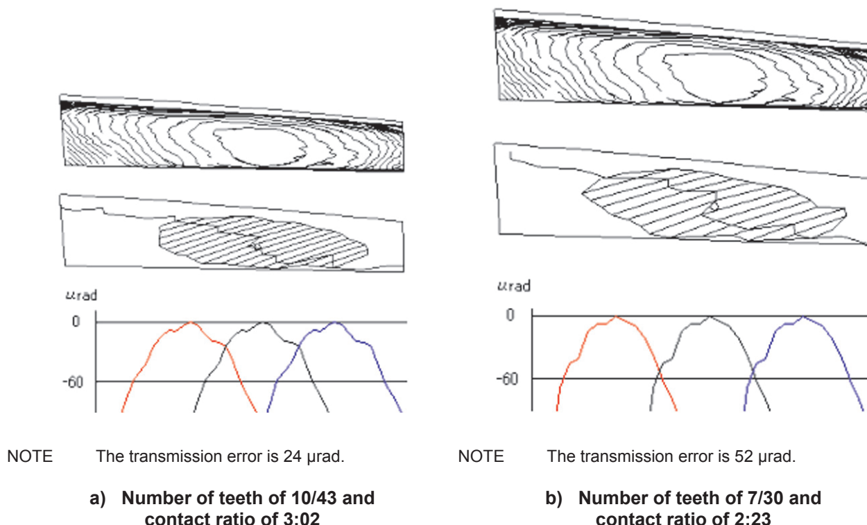
Figure 3 — The effect of design contact ratio on transmission error
