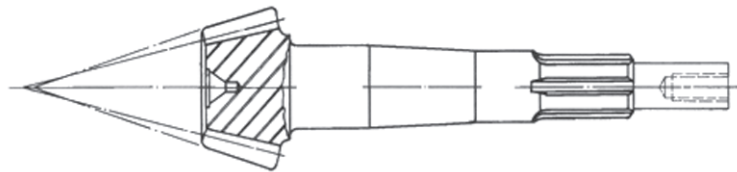
Figure 8 — Shank-type pinion with tapped hole
