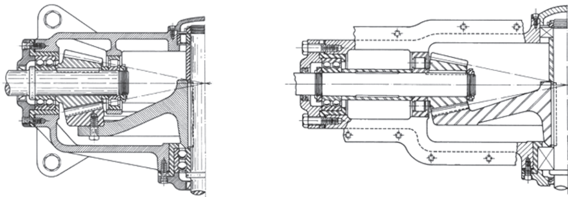
a) Straddle mounting for both members
