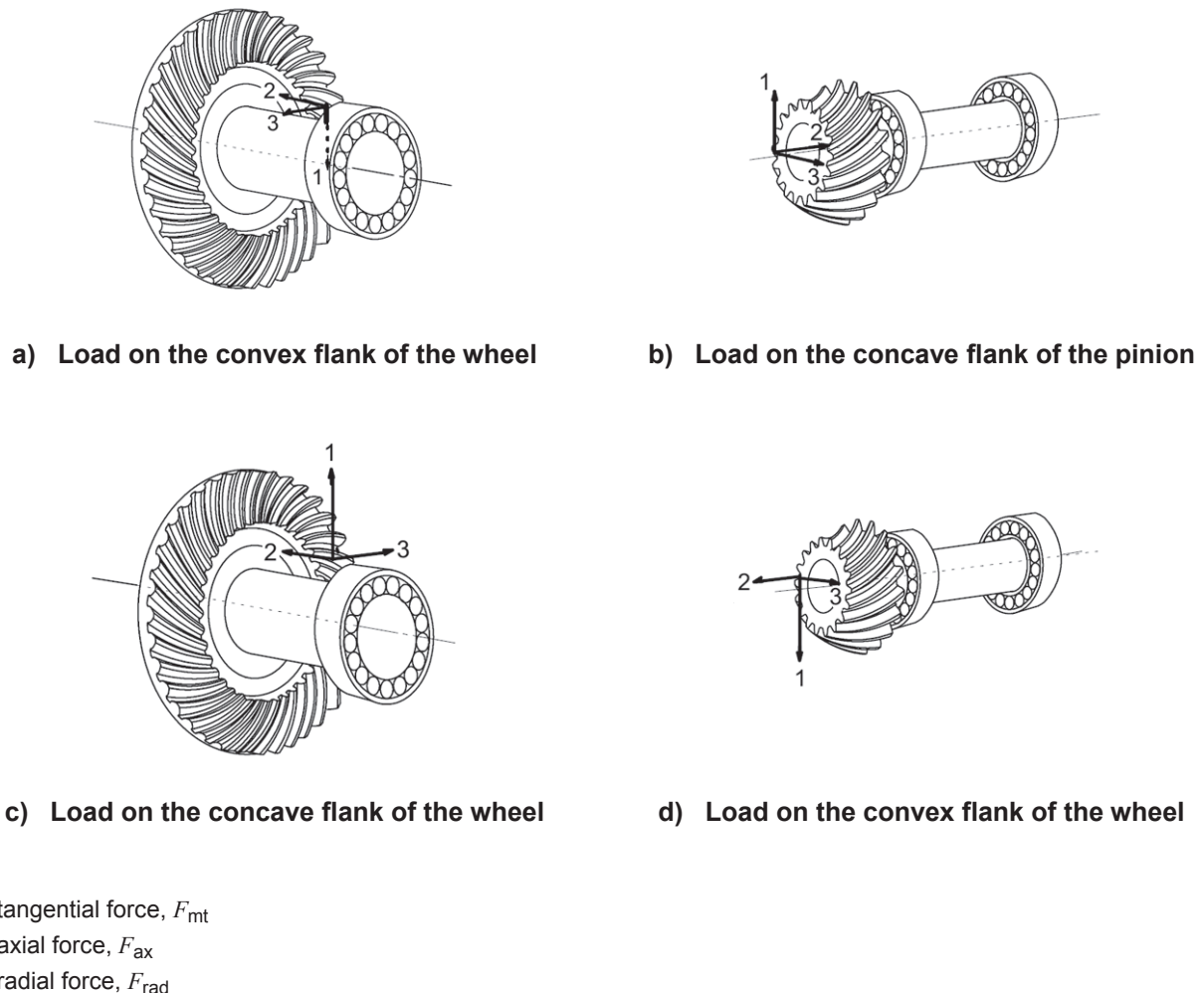
Figure 26 — Typical gear tooth forces
