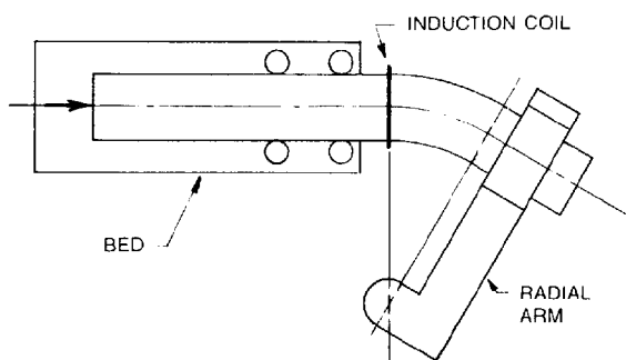
FIGURE 3.4.3 INDUCTION BENDING
