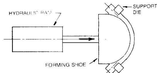
FIGURE 3.5.2 RAM BENDING
