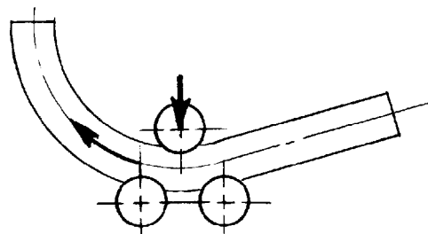
FIGURE 3.5.3 ROLL BENDING
