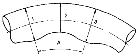
FIGURE 6.2 APPLICATION OF PIPE WALL BUCKLING TOLERANCES
