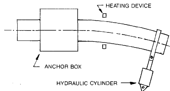
FIGURE 3.4.2 INCREMENTAL BENDING
