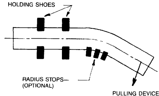
FIGURE 3.4.1 FURNACE BENDING
