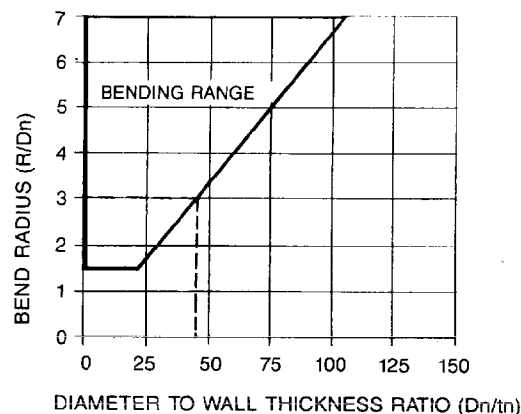
FIGURE 6.5.2 INDUCTION AND INCREMENTAL BENDING RANGE
