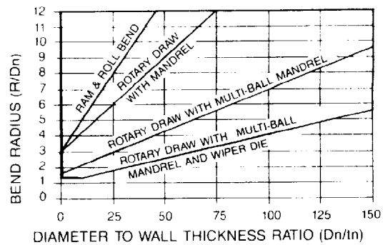
FIGURE 6.8.1 COLD BENDING RANGE
