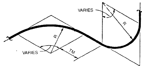
FIGURE 7.5.4 TANGENT LENGTHS
