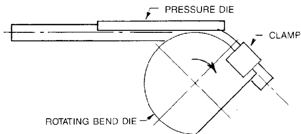
FIGURE 3.5.1 ROTARY DRAW BENDING
