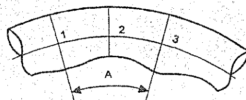
FIGURE 6.2 APPLICATION OF PIPE WALL BUCKLING TOLERANCES
