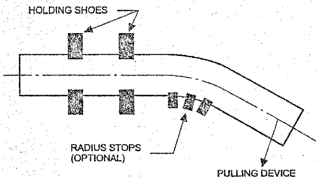
FIGURE 3.4.1 FURNACE BENDING
