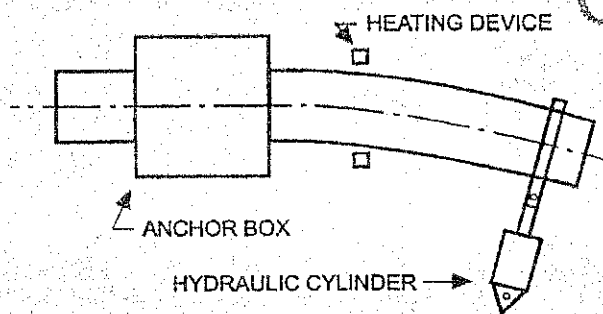
FIGURE 3.4.2 INCREMENTAL BENDING
