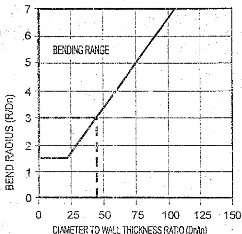
FIGURE 6.5.2 INDUCTION AND INCREMENTAL BENDING RANGE
