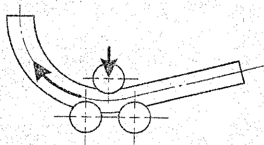
FIGURE 3.5.3 ROLL BENDING
