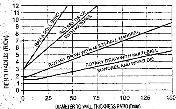
FIGURE 6.8.1 COLD BENDING RANGE
