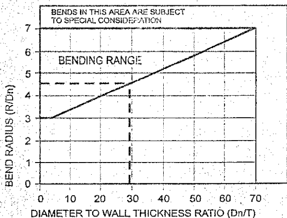
FIGURE 6.5.1 FURNACE BENDING RANGE
