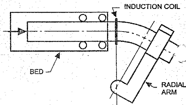
FIGURE 3.4.3 INDUCTION BENDING
