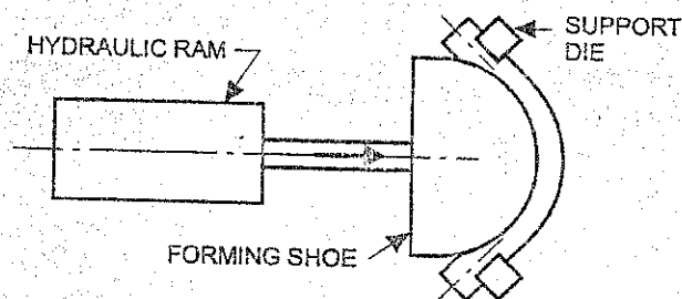
FIGURE 3.5.2 RAM BENDING
