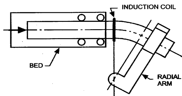
FIGURE 3.4.3 INDUCTION BENDING
