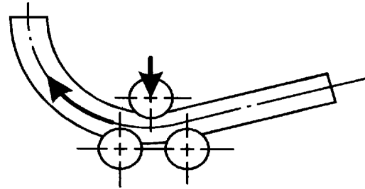
FIGURE 3.5.3 ROLL BENDING
