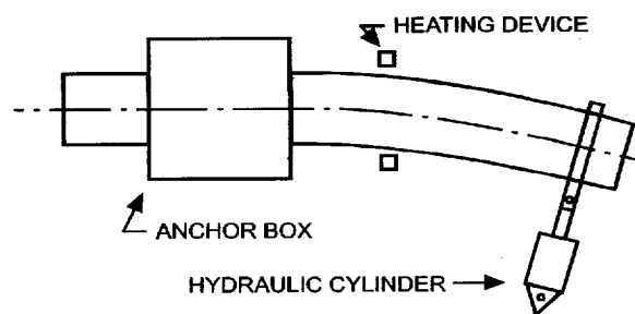
FIGURE 3.4.2 INCREMENTAL BENDING
