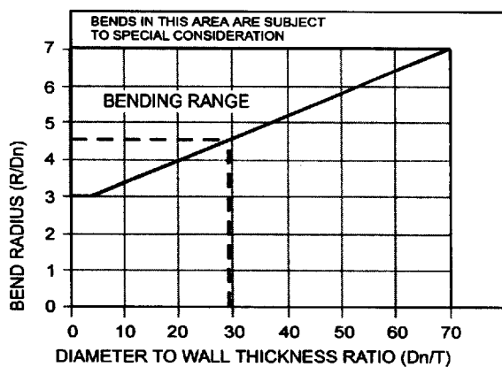
FIGURE 6.5.1 FURNACE BENDING RANGE
