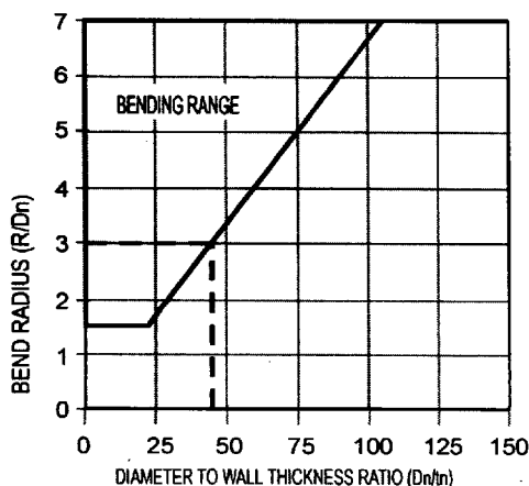
FIGURE 6.5.2 INDUCTION AND INCREMENTAL BENDING RANGE
