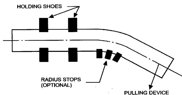
FIGURE 3.4.1 FURNACE BENDING
