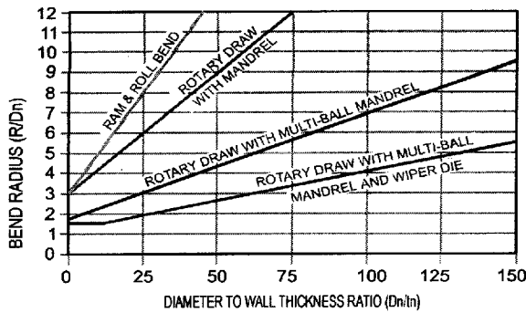
FIGURE 6.8.1 COLD BENDING RANGE
