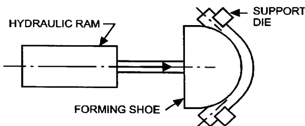
FIGURE 3.5.2 RAM BENDING
