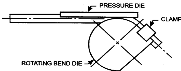
FIGURE 3.5.1 ROTARY DRAW BENDING
