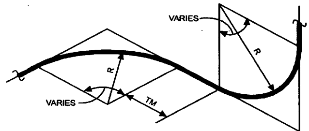
FIGURE 7.5.4 TANGENT LENGTHS
