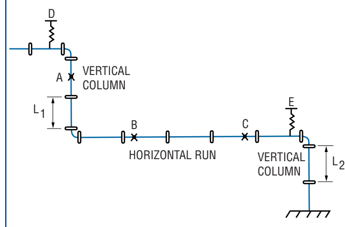
FIGURE 43 - PRESSURE THRUST
