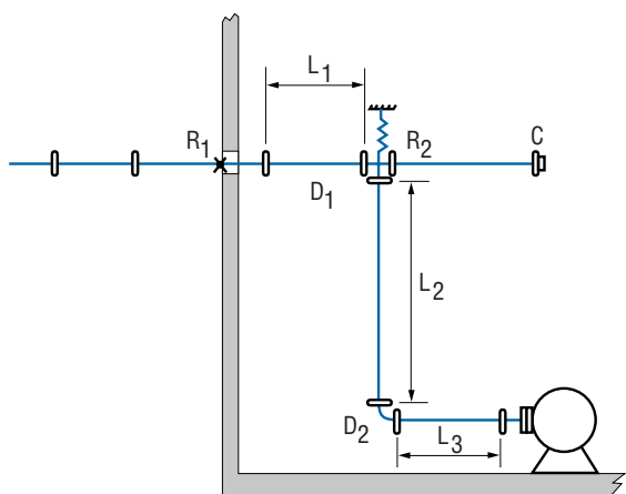
FIGURE 42 - PRESSURE THRUST
