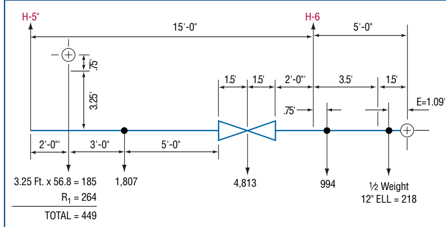
FIGURE 8 – ELEVATION VIEW
