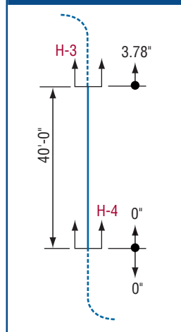
FIG. 13A – MOVEMENT AT H-3
