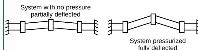
FIGURE 44 - LATERAL RESTRAINT
