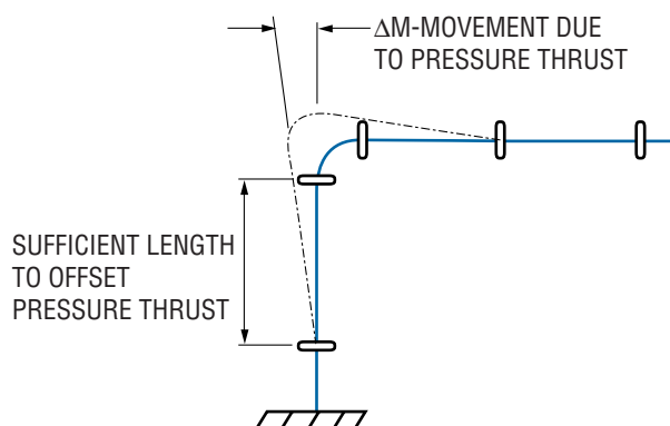
FIGURE 41 - PRESSURE THRUST
