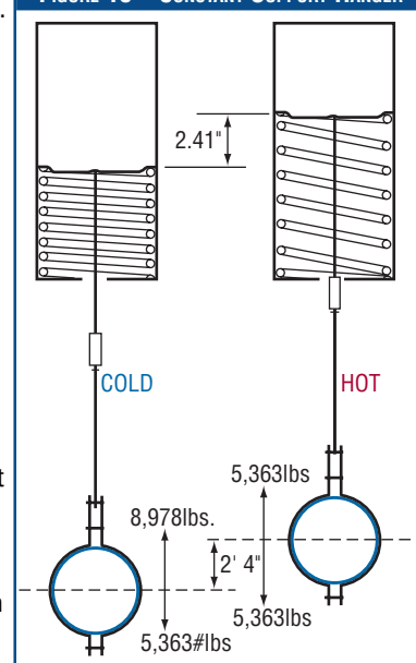
FIGURE 18 – CONSTANT SUPPORT HANGER
