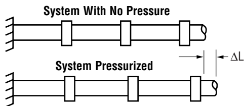
FIGURE 40 - PRESSURE THRUST
