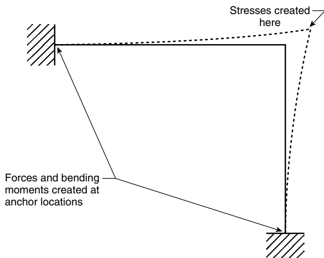
FIGURE 7.1 Changes in a simple L pipe connection. The solid line shows ambient pipe and the dashed line shows expanded pipe.
