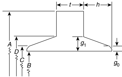
FIGURE 9.3 Anchor flange
