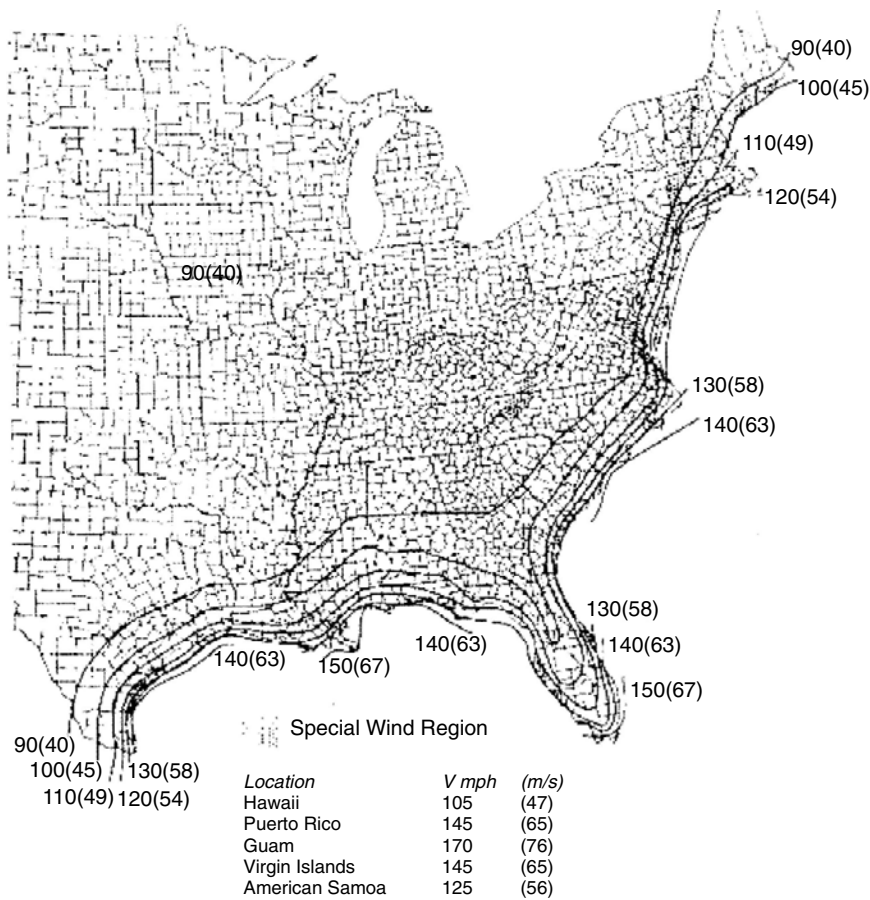
FIGURE 11.2 Basic wind speeds for eastern United States ( Source: From ASCE; used with permission.)
