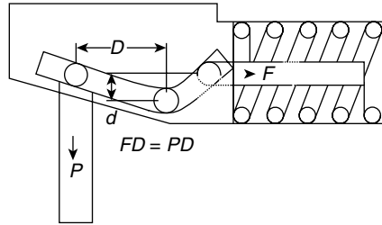
FIGURE 8.4 Constant force hanger arrangement
