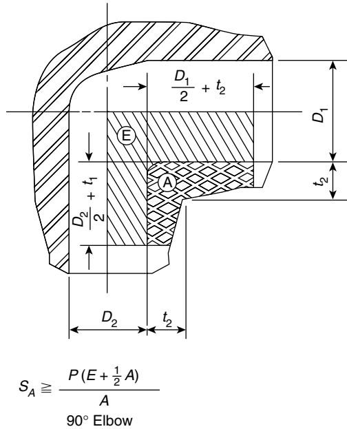
FIGURE 6.4 Pressure area elbow
