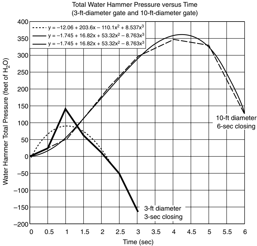
FIGURE 12.2 Water hammer pressure time
