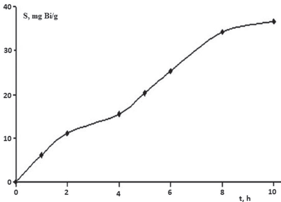
Figure 5-1. Kinetic curve of the Bi(III)-containing cation sorption at 55^\circ\text{C} on the AV-17 polymer.
