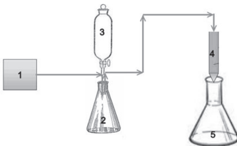
Figure 7-71. Installation scheme for the experiments: 1 – air pump, 2 – KI and \text{H}_2\text{SO}_4 solution, 3 – \text{KMnO}_4 solution, 4 – column with AV-17 (Bi), and 5 – starch solution.
