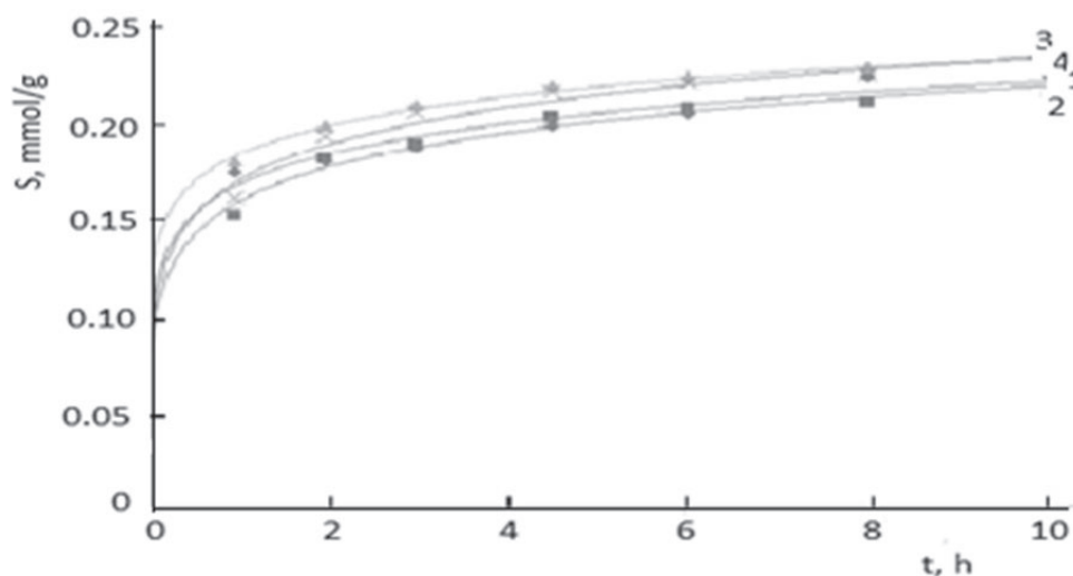
Figure 4-5. The kinetic curve of \text{Nd}^{3+} ion sorption on Purolite A-400, obtained experimentally at 50 (3) and 21°C (1) and calculated with the pseudo-second-order kinetic model at 50 (4) and 21°C (2).
