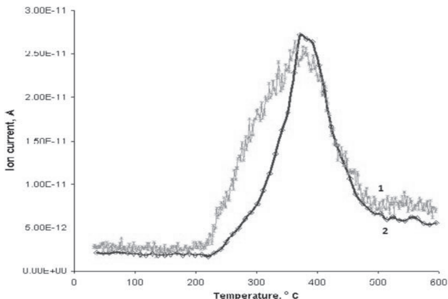
Figure 7-9. Ionic current variation with temperature for the sorbent AV-17(Cr) containing \text{Cr}_2\text{O}_7^{2-} (1) and sorbent AV-17(Cr) containing \text{CrO}_4^{2-} (2) for the m/z=30 fragment.
