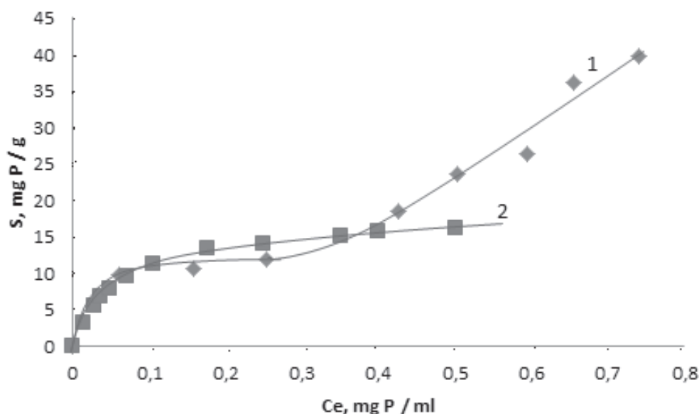
Figure 7-32. Equilibrium sorption isotherm of phosphate on AV-17(Cr): obtained experimentally (1) and calculated by the BET (2) sorption model.
