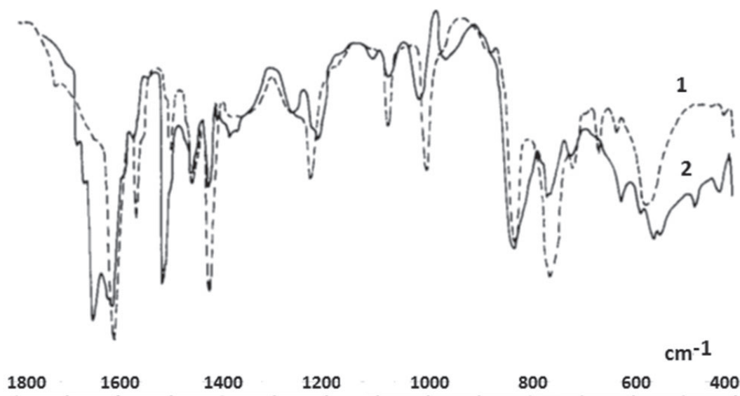
Figure 1-17. IR spectra 4-VP-8% DVB gel type copolymer (1) and 4-VP: 8% DVB gel-type copolymer – Fe(III) complex (2).
