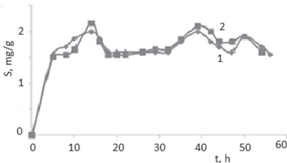
Figure 7-83. Kinetic curves of Ga(III)-containing (1) and In(III)-containing cations sorption (2) on AV-17 polymer at 60°C.
