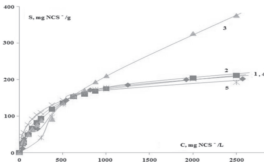
Figure 7-54. Equilibrium sorption isotherm of \text{NCS}^- ions on AV-17(Cr) in a large range of \text{NCS}^- concentration: obtained experimentally (1), calculated by Langmuir (2), Freundlich (3), Sips (4) and Dubinin-Radushkevich (5) sorption models.
