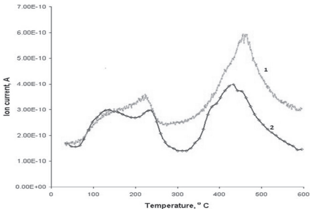
Figure 7-7. Ionic current variation with temperature for the sorbent AV-17(Cr) containing \text{Cr}_2\text{O}_7^{2-} (1) and sorbent AV-17(Cr) containing \text{CrO}_4^{2-} (2) for the m/z -18 fragment.
