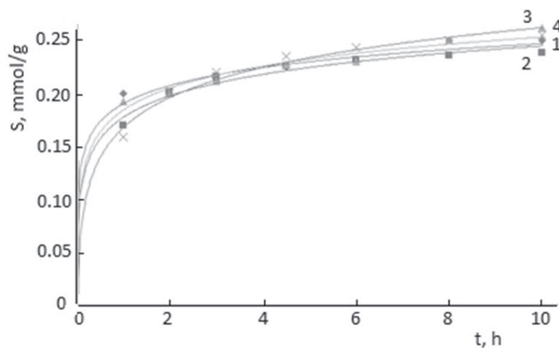
Figure 4-7. The kinetic curve of \text{Er}^{3+} ion sorption on Purolite A-400, obtained experimentally at 50 (3) and 21°C (1) and calculated with the pseudo-second-order kinetic model at 50 (4) and 21°C (2)
