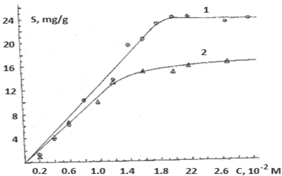
Figure 3-3. Sorption isotherms of Al (III)-containing cations on polymers AV-17 (1) and Varion-AD (2).
