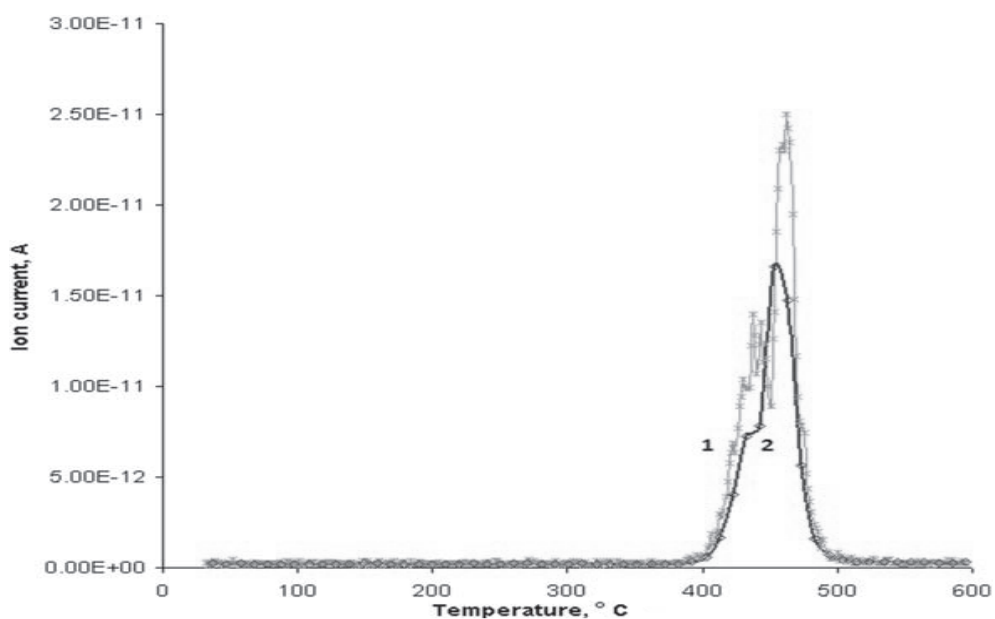
Figure 7-13. Ionic current variation with temperature for the sorbent AV-17(Cr) containing \text{Cr}_2\text{O}_7^{2-} (1) and sorbent AV-17(Cr) containing \text{CrO}_4^{2-} (2) for the m/z -120 fragment.
