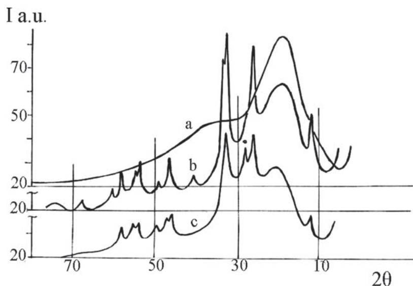
Figure 5-6. X-ray diffraction spectra of the (a) Bi(III)-containing AV-17 and the Bi(III)-containing polymer after heating in (b) water and (c) in 0.1M \text{Na}_2\text{SO}_4 solution. I, signal intensity, arbitrary units.
