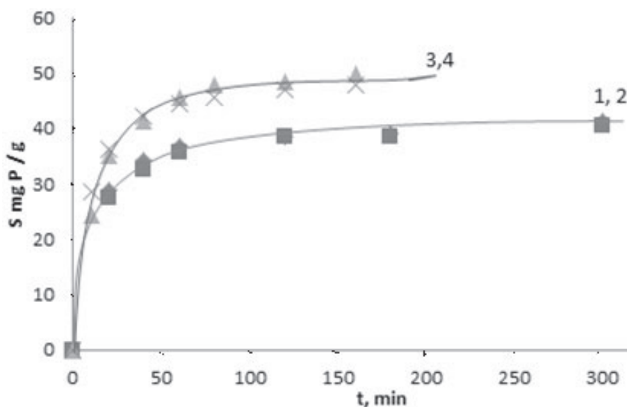
Figure 7-27. Integral kinetic curves of phosphate sorption on AV-17(Cl) at 20°C: 1 – experimentally obtained, 2 – calculated with the PSO kinetic model; and at 54°C: 3 – experimentally obtained and 4 – calculated with the PSO kinetic model.
