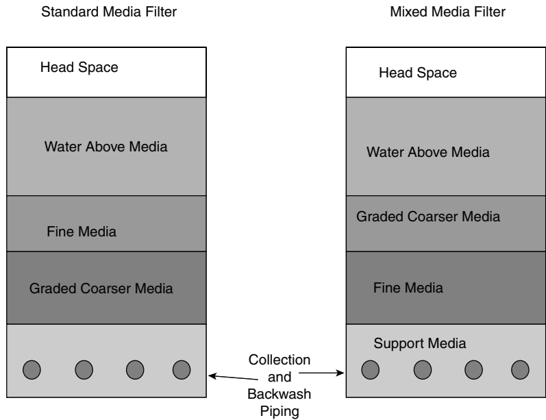
FIGURE 8.1 Comparison of conventional and mixed media filters.
