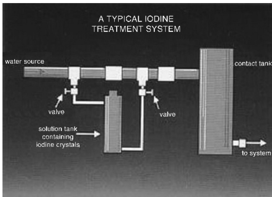
FIGURE 9.9 Schematic drawing of a bypass iodinator—United States patent 4555347.
