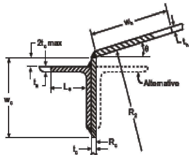
Detail a
