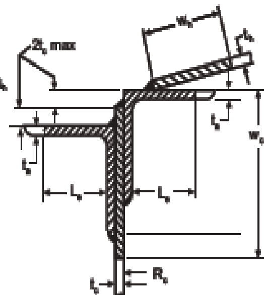
Detail g
