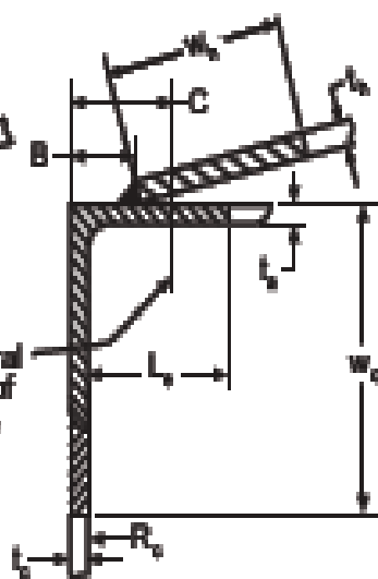
Detail e
