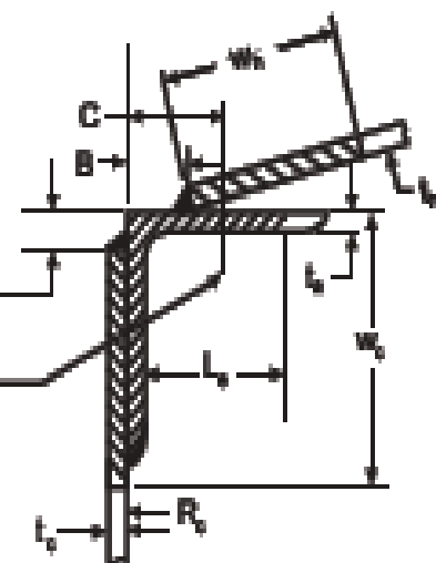
Detail c
