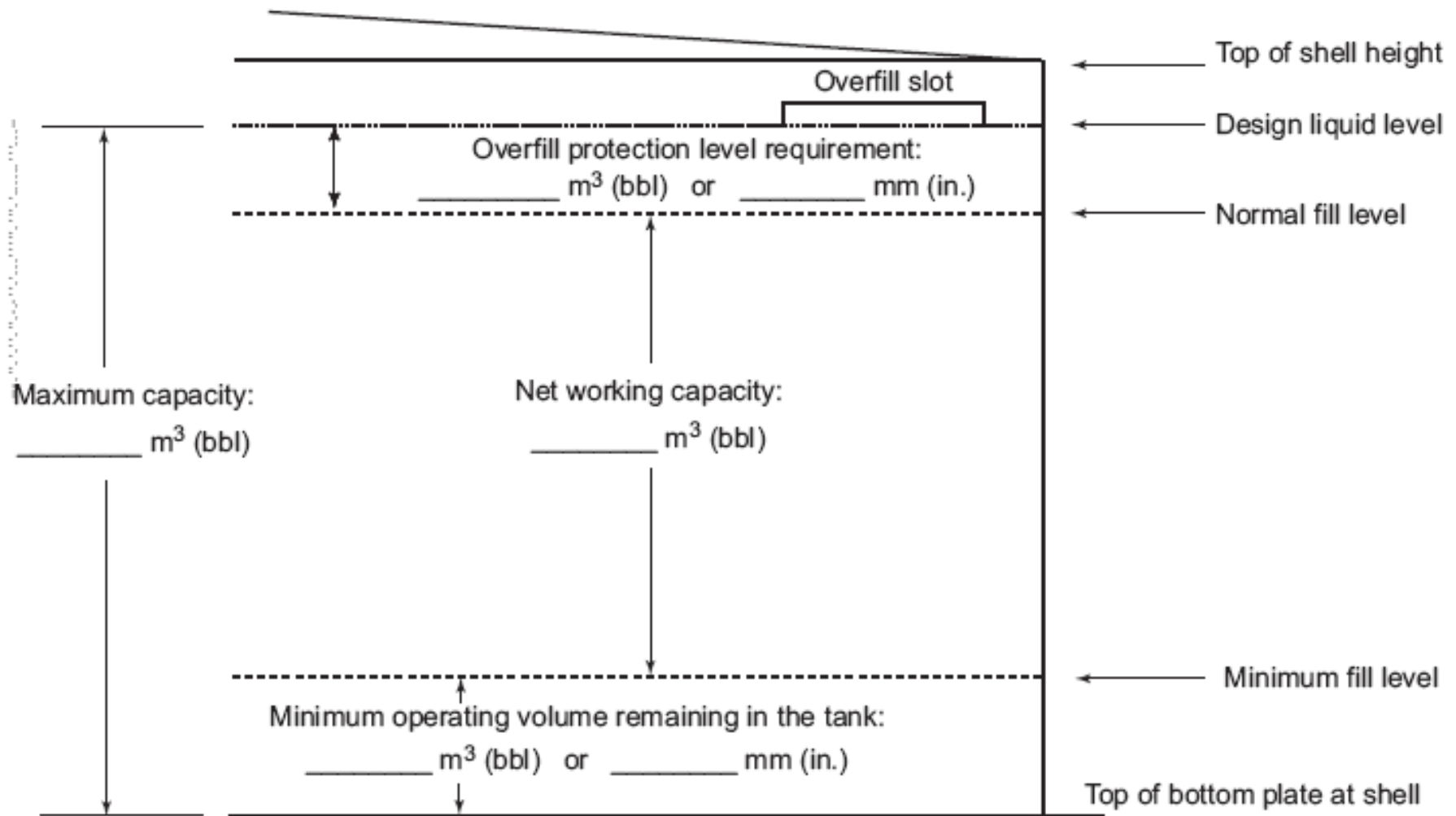
Figure 5.4—Storage Tank
