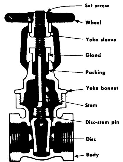
No. 459 Underwriters' Pattern Outside Screw & Yoke Wedge Disc
