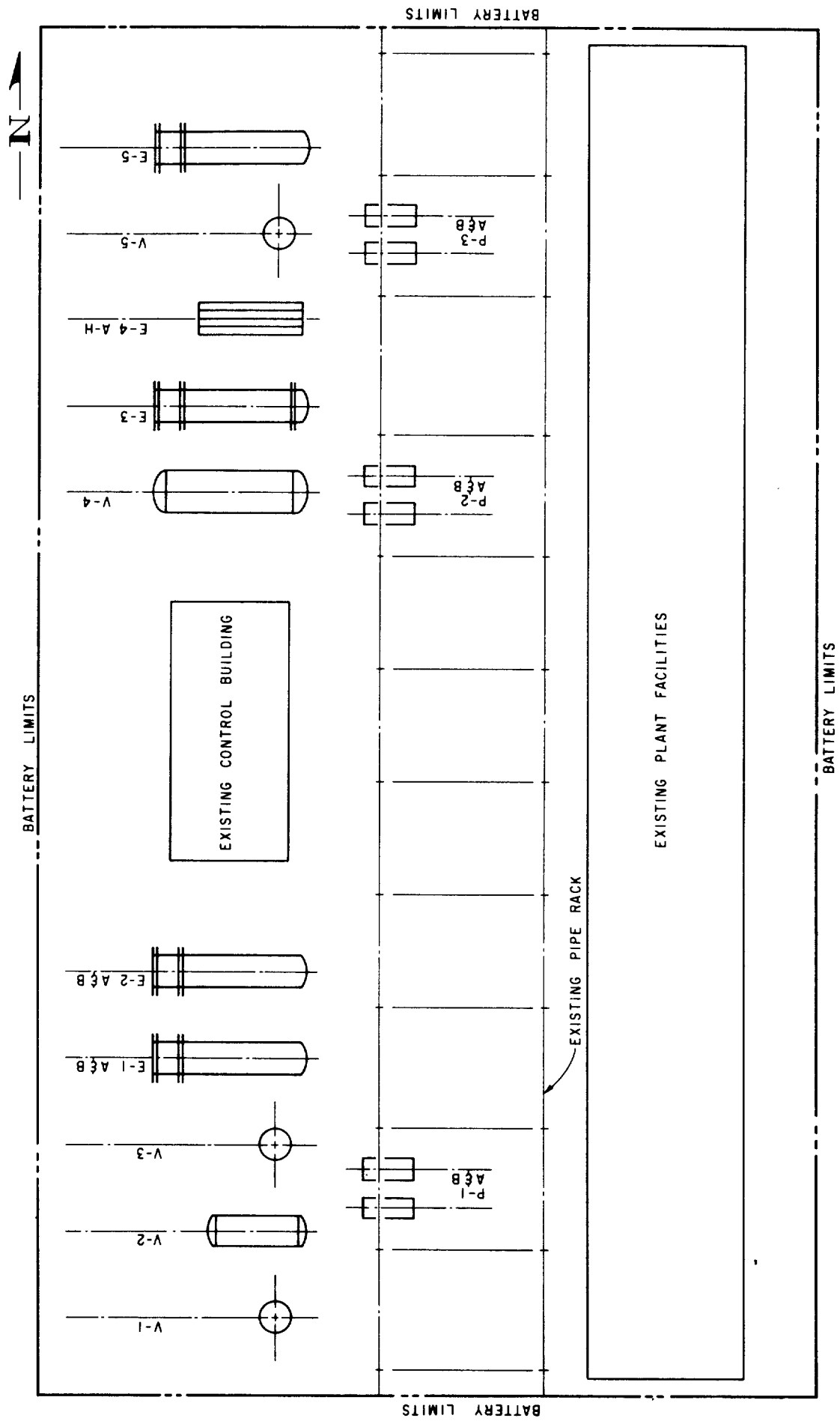
Figure 5-1. Plot Plan.
