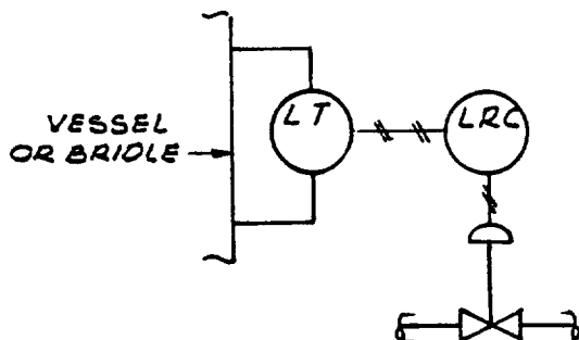
Flow Diagram Symbol
