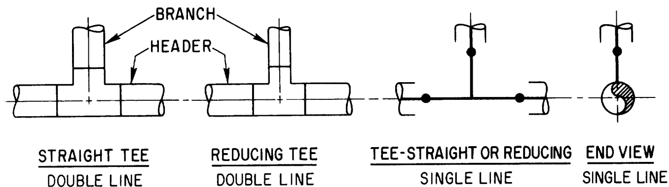
Figure 2-7. Weld tee.
