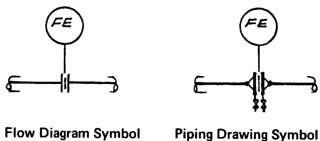
Figure 3-4b. Flow Element (FE) is used for testing flow with portable equipment. Consists of orifice set with plate and plugged tap valves. Up-and-down stream pipe section lengths (see meter runs) are critical and are considered a part of the measuring device.
