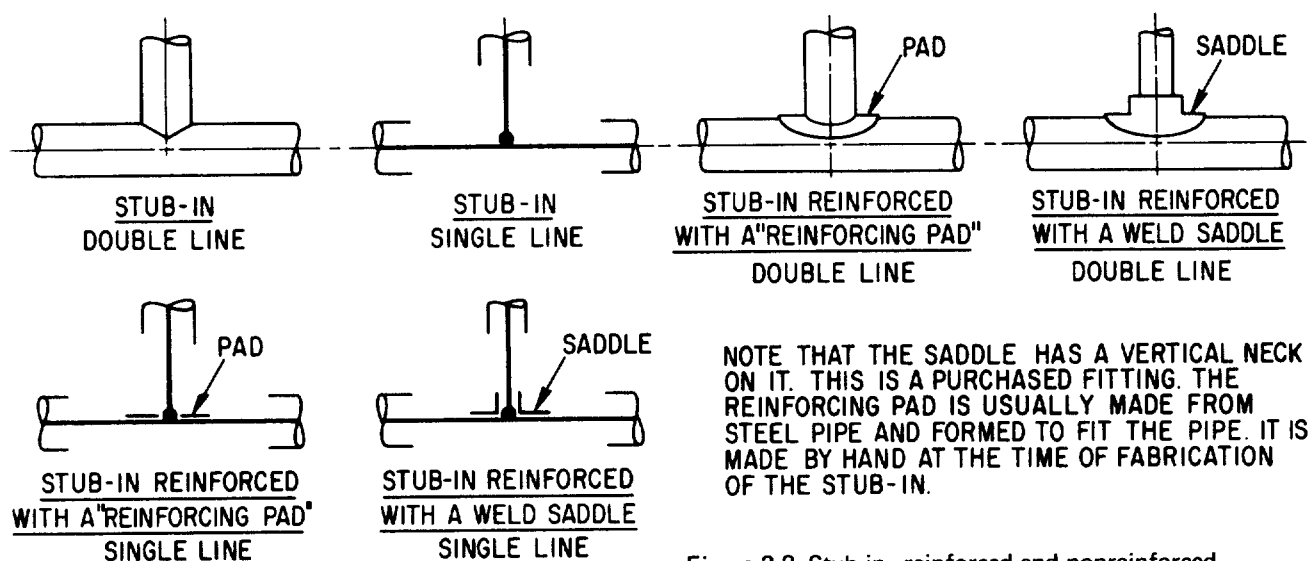
Figure 2-8. Stub-in—reinforced and nonreinforced.
