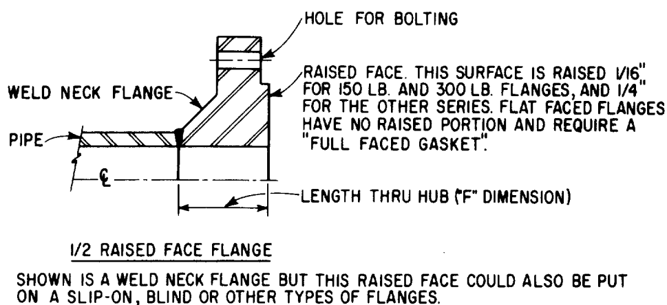
Figure 2-16. Weld neck raised face flange.
