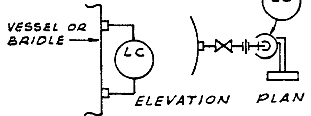
Piping Drawing Symbol
