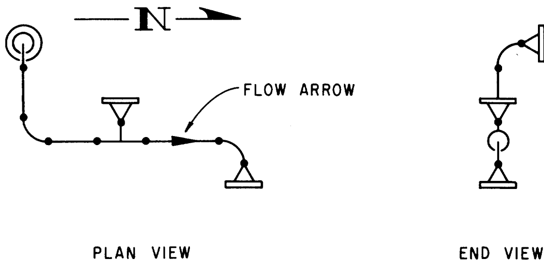
Figure 8-3. Orthographic #1.
