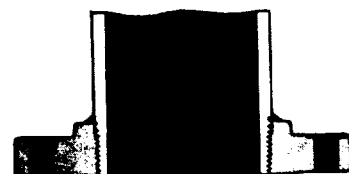
Screwed Flange Seal-Welded and Refaced
