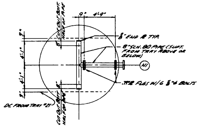
DETAIL OF INTERNALS FOR N1 SCALE: 1/2" = 1'-0"
