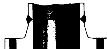
Welding Neck Flange Butt-Welded to Pipe
