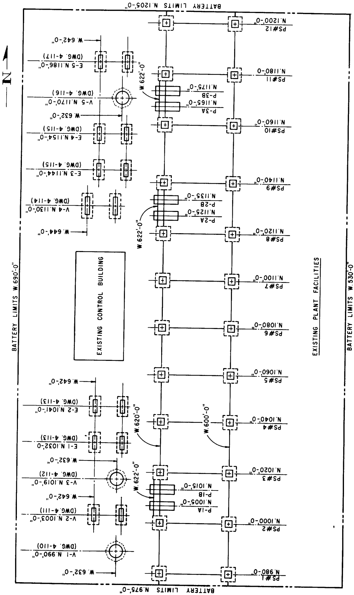
Figure 5-2. Foundation Location Plan.
