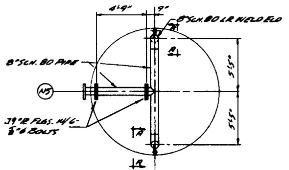
DETAIL OF INTERNALS FOR N5 SCALE: 1/2" = 1'-0"
