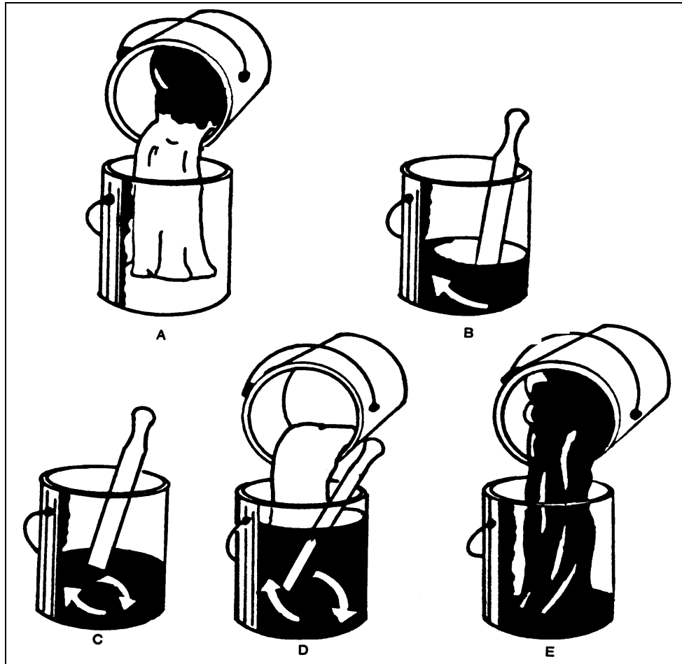
Figure 7 Illustration of Mixing and "Boxing" One-Component Paint: A - Pouring Off Pigment-Poor Vehicle, B and C - Mixing Pigment to Form Smooth Paste, D - Pouring in Vehicle and Mixing, E - Boxing Paint
