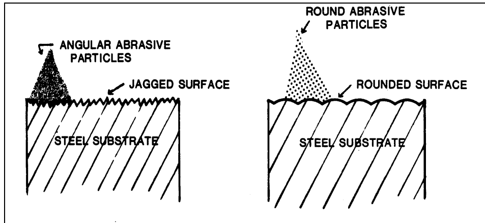
Figure 4 Drawing Illustrating Effect of Shape of Abrasive Particle on Contour of Blast-Cleaned Metallic Substrate
