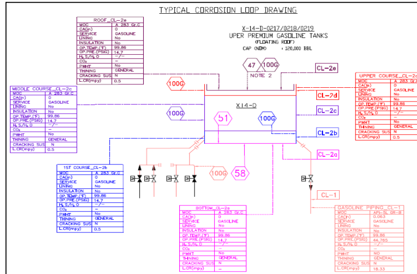
Figure 3 - Typical Corrosion Loop Drawing for Tank
