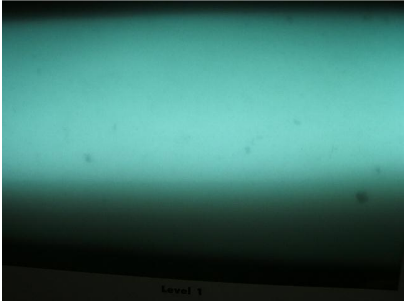
Category B1 Sand and slag inclusions
