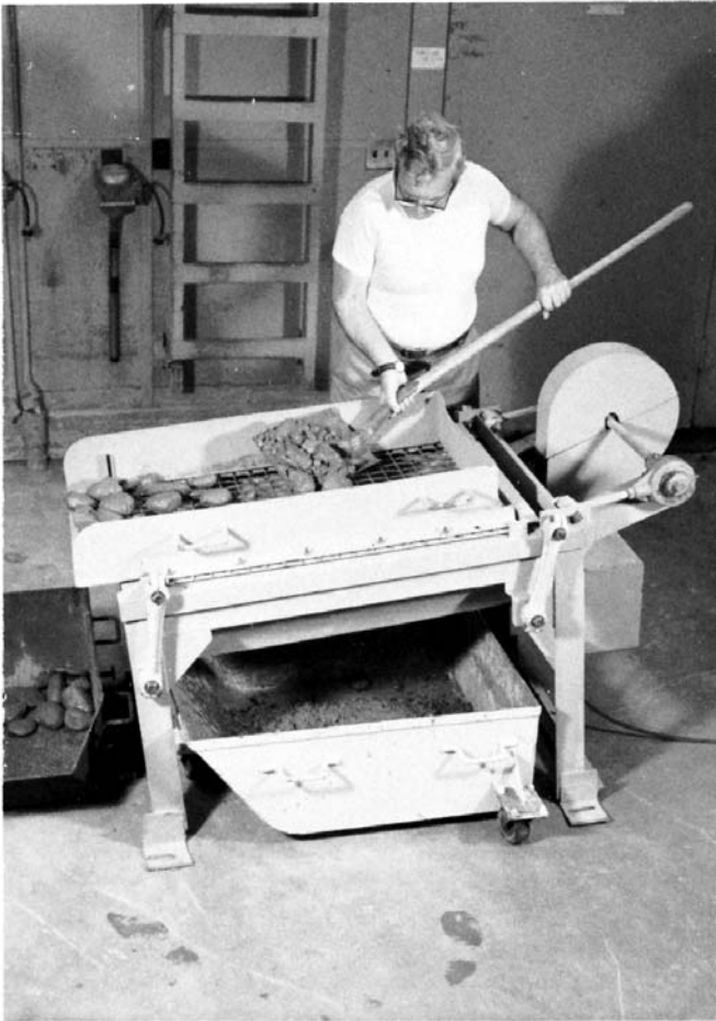
FIG. 6 Mechanical Equipment for Wet Sieving Concrete
