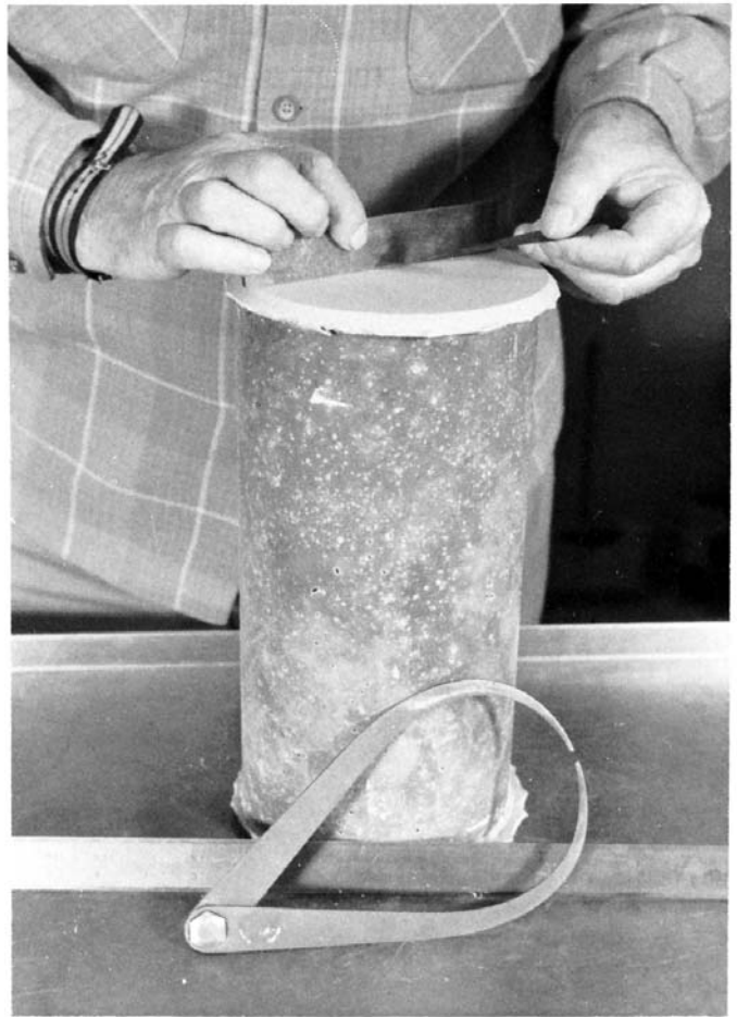
FIG. 1 Checking Planeness of the Capped End of a Concrete Cylinder Prior to Testing Using a 6-in. (152-mm) Machinists' Parallel and a 0.002-in. (0.05-mm) Feeler Gauge
