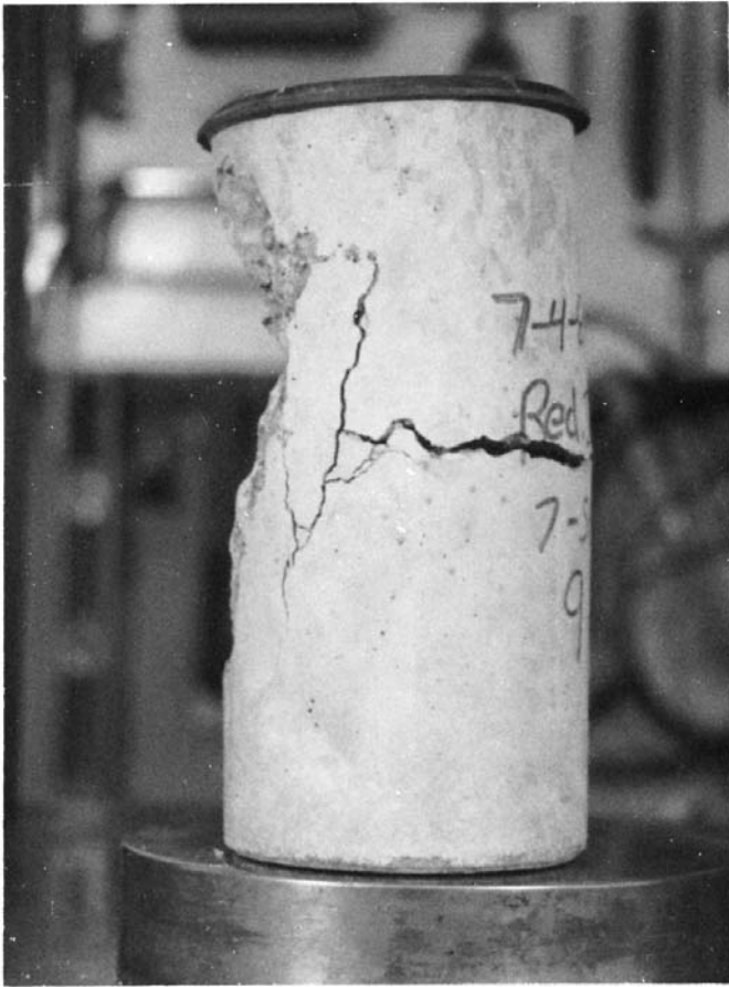
FIG. 3 Atypical Failure of a Concrete Cylinder Due to Incorrect Testing Procedures
