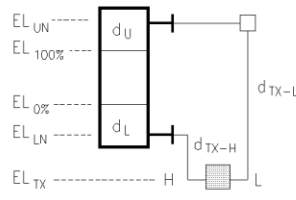
Arrangement-2: Closed equipment; Wet reference leg.
