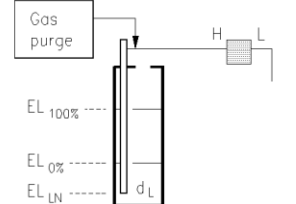
Arrangement-5: Open equipment; No reference leg; External gas purging (entry point near purge pipe); Terms T-1/3/4 = 0.
