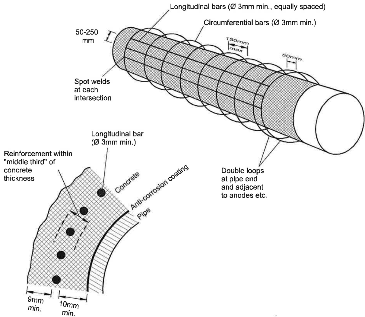
Figure 1 Reinforcement details
