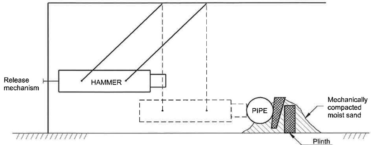
Figure 3 Impact test rig
