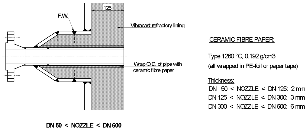
Figure 8-4: Typical nozzle for dense (vibra-)cast refractory linings
