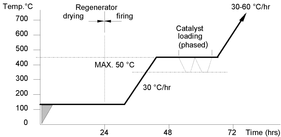
Figure 2: Curing, drying and firing of FCCU unshaped refractory materials
