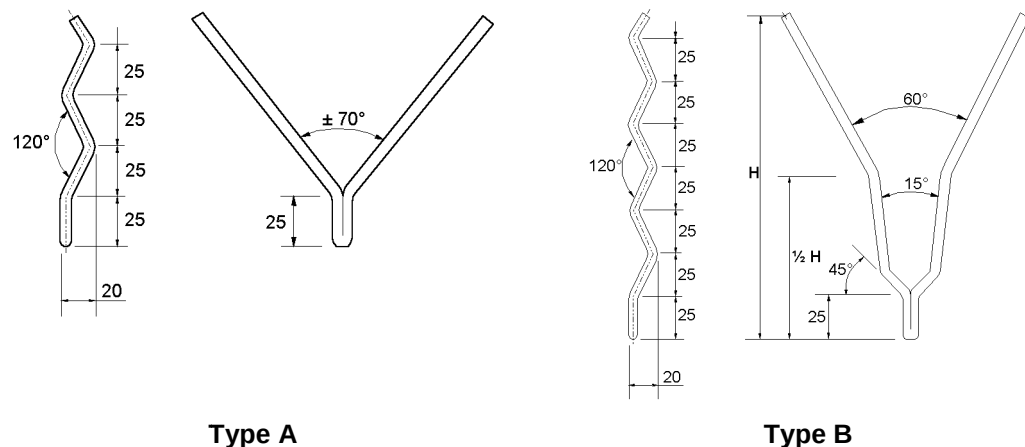
Figure 2 Dimensions of V-anchors for stud welding only
