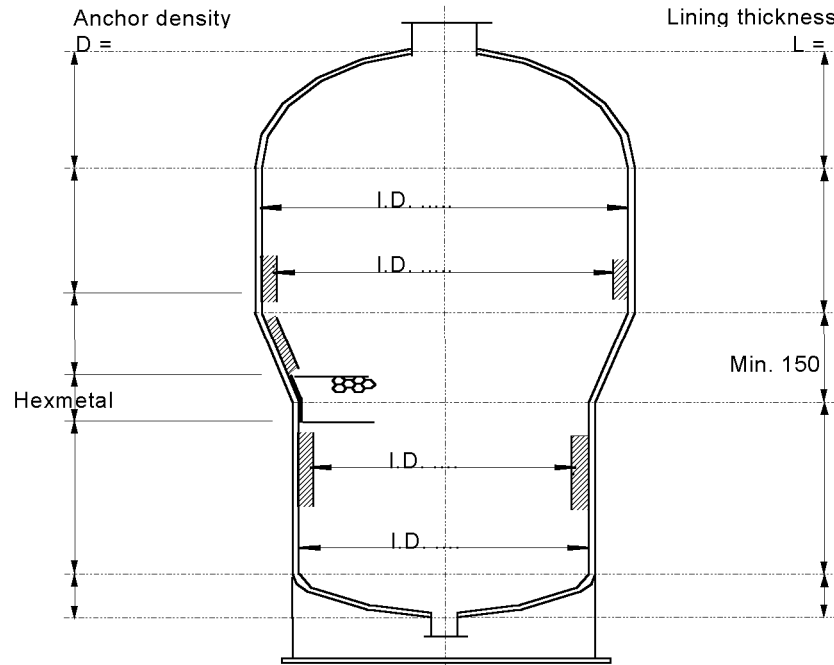
Figure 2 Anchors for FCCU Regenerator refractory linings (typical only)
