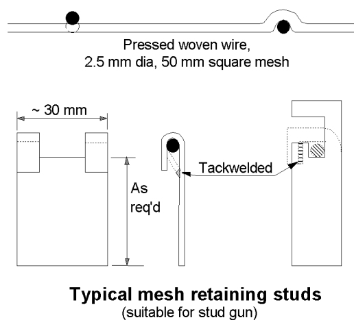
Figure 5 Typical wire mesh arrangement
