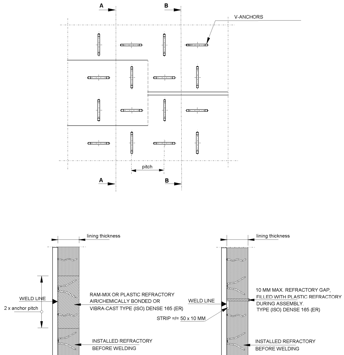
Figure 6 Refractory lining detail at field welds
