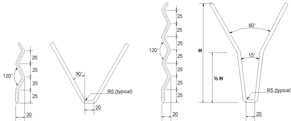
Figure 1 Dimensions for V-anchors for single and double layers
