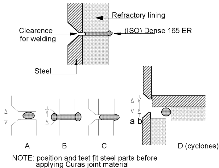
Figure 4 Typical jointing detail of shop/field joints
