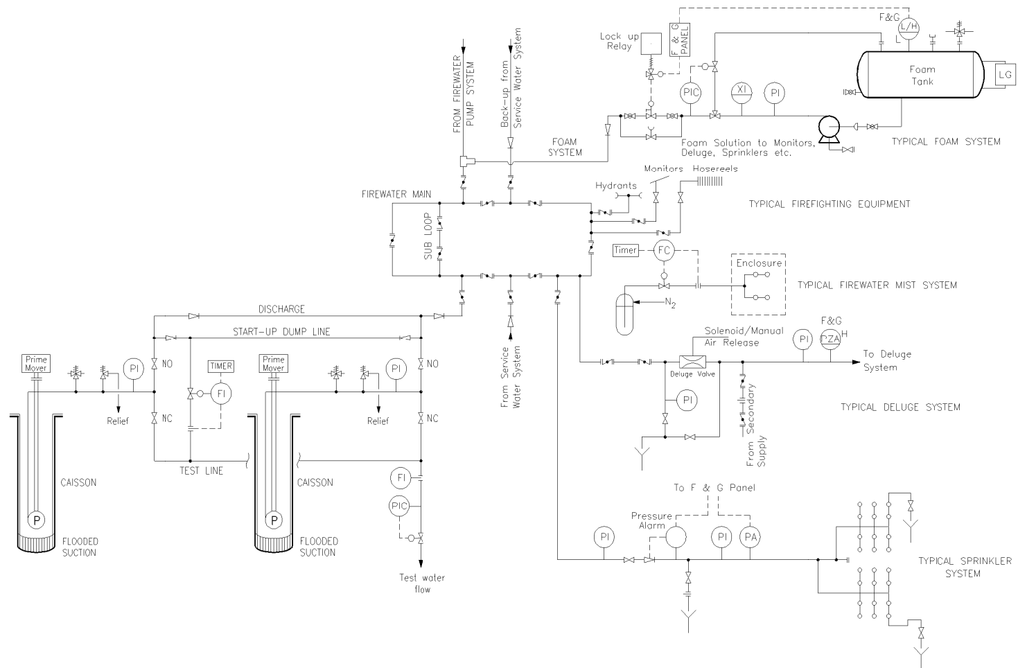
FIGURE 1 FIREWATER MAIN SYSTEM ELEMENTS
