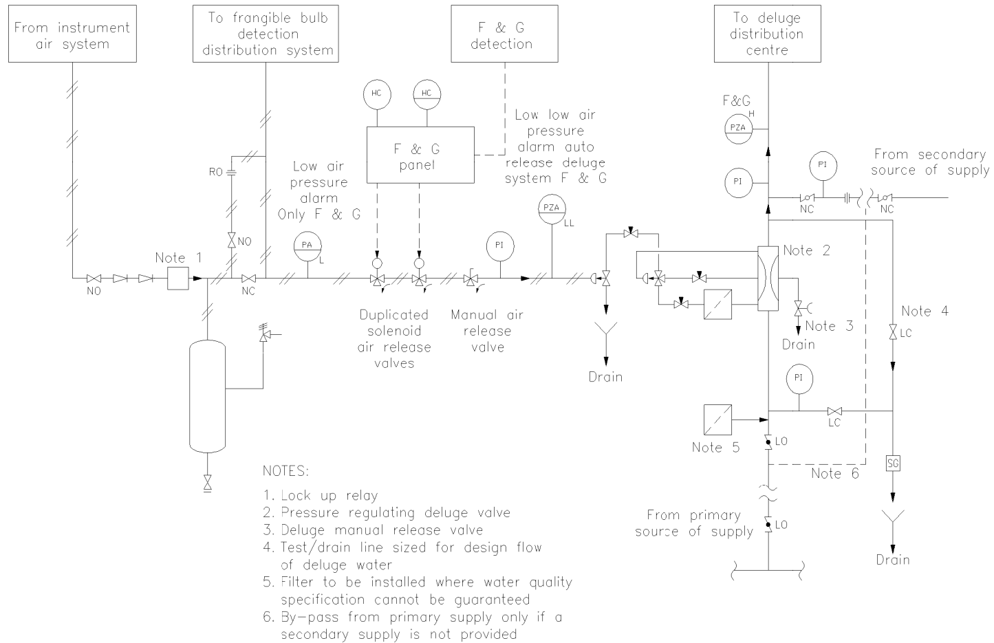
FIGURE 6 PEFS FOR TYPICAL DELUGE VALVE SET
