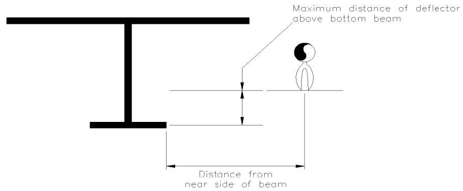
FIGURE 7 SPRAY HEAD LOCATION WITH RESPECT TO BEAMS
