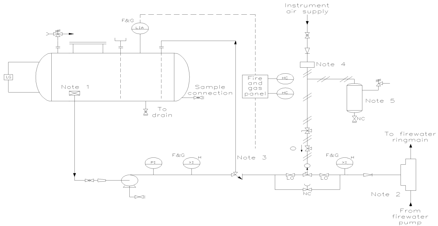
FIGURE 10 TYPICAL CENTRAL FOAM PROPORTIONING SCHEMATIC
