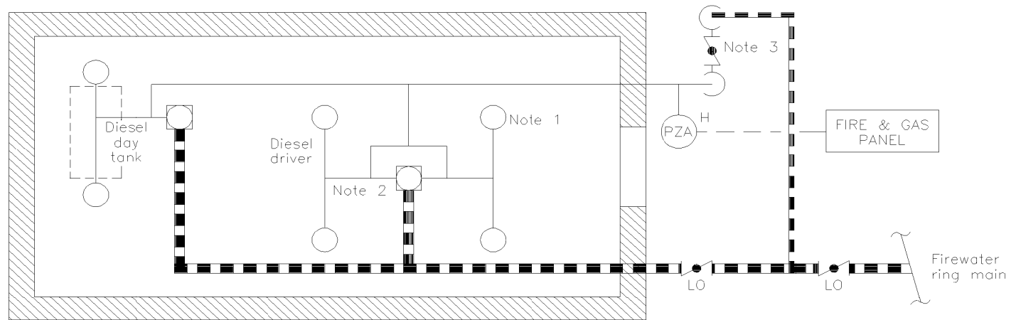
FIGURE 9 SCHEMATIC LAYOUT OF A TYPICAL MINI-DELUGE SYSTEM
