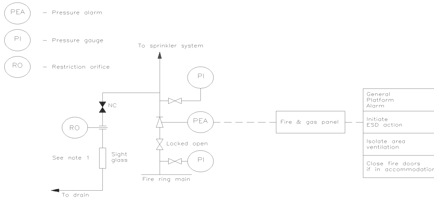
FIGURE 5 P&ID FOR TYPICAL SPRINKLER VALVE ASSEMBLY
