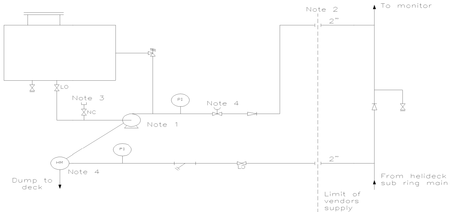
FIGURE 11 HELIDECK FIRE FIGHTING FOAM TANK SCHEMATIC
