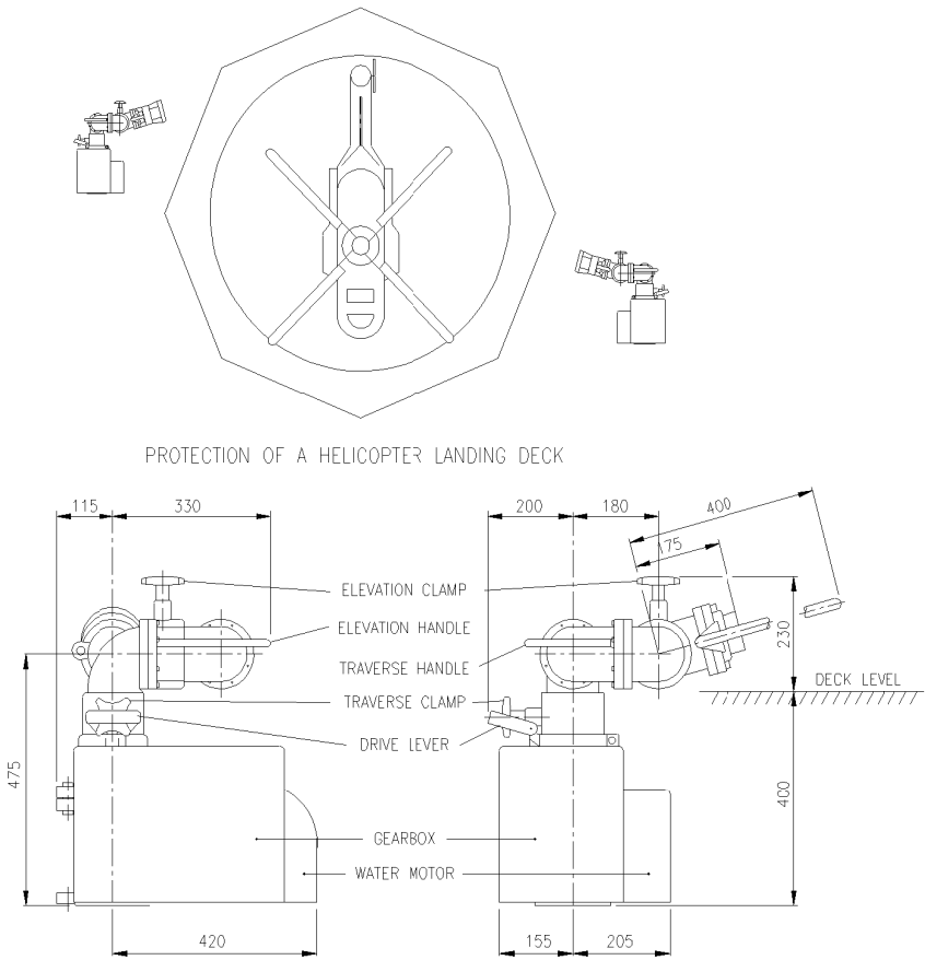
FIGURE 12.2 TYPICAL OSCILLATING MONITORS USED FOR HELIDECK PROTECTION
