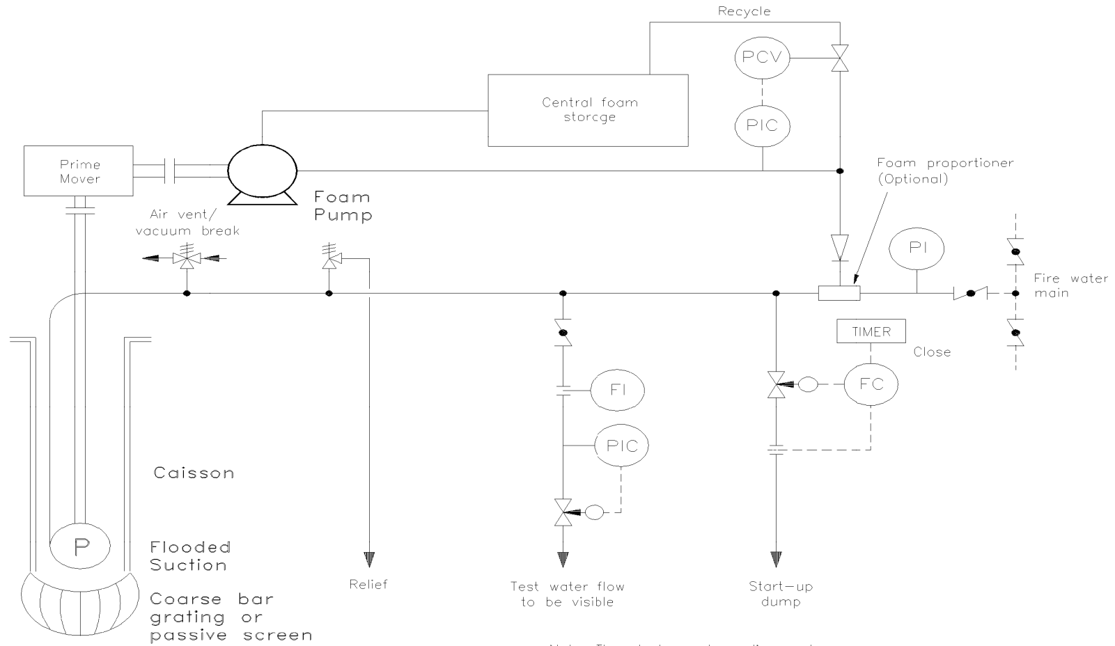
FIGURE 2 FIREWATER PUMP PIPING AND INSTRUMENT DIAGRAM
