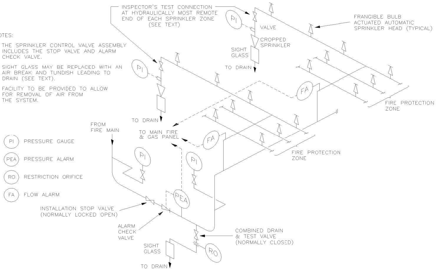
FIGURE 4 SCHEMATIC DIAGRAM OF TYPICAL SPRINKLER SYSTEM (SALT WATER FILLED)
