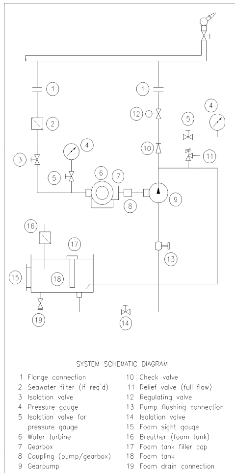
FIGURE 12.3 TYPICAL PROPORTIONING PACKAGE WITH HELIDECK PROTECTION SYSTEMS
