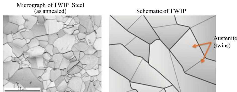
Fig. 4.8 TWIP microstructure of twinned austenite [Source WorldAutoSteel]
