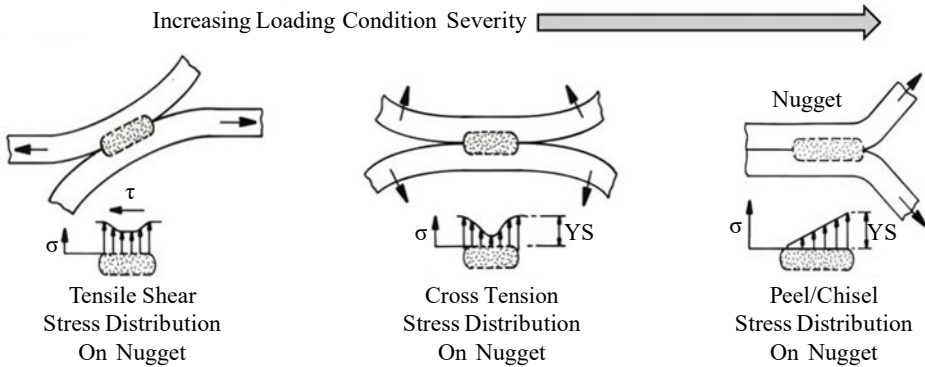
Fig. 8.2 The effect of loading condition on nugget stress distribution
