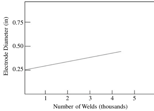
Fig. 10.1 Typical relationship between electrode diameter and number of welds made during electrode life testing
