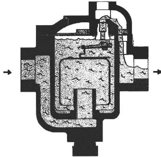
Figure 15-1 Inverted-bucket trap.
