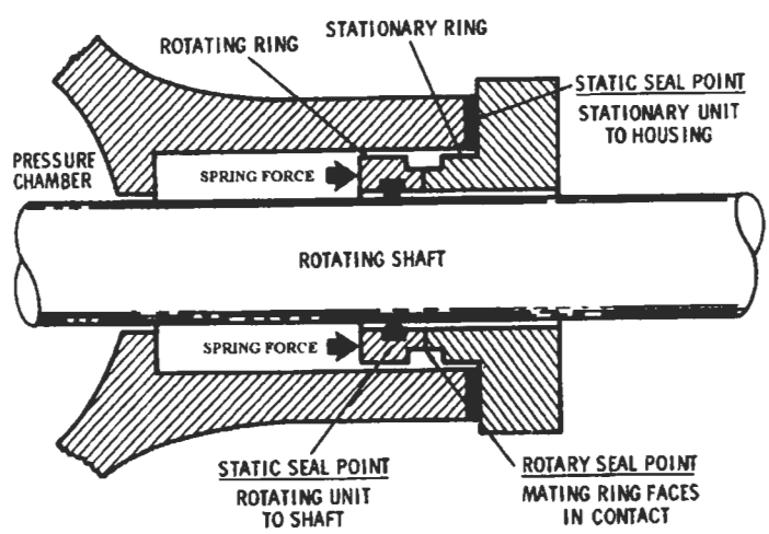
Figure 18-2 Simple mechanical seal (Bearings Inc. catalogue).
