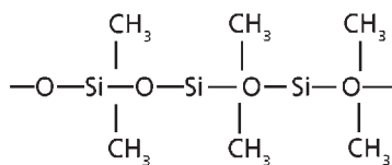
Silicone polymer
