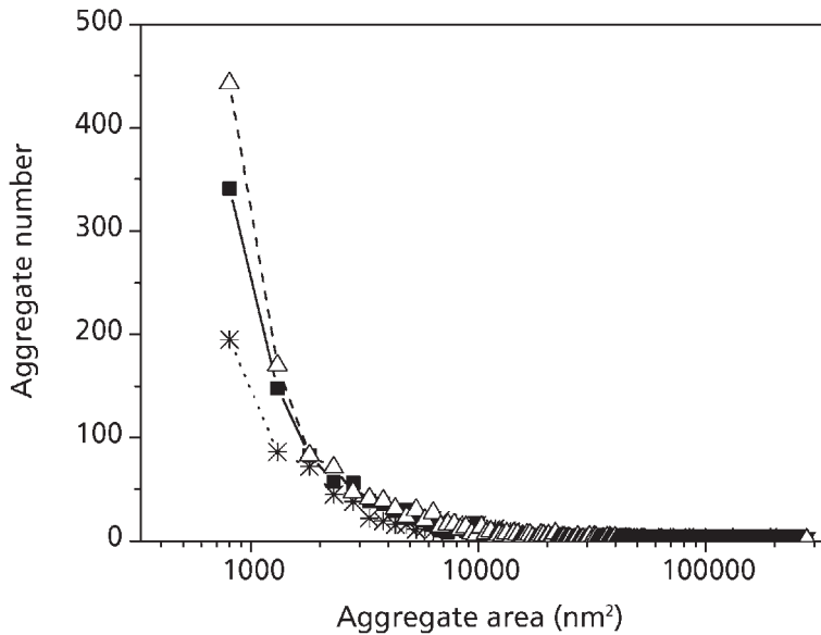
Figure 1.11 Aggregate number of silica against their area in compounds based on: △ SBR; ■ NR; * BR
