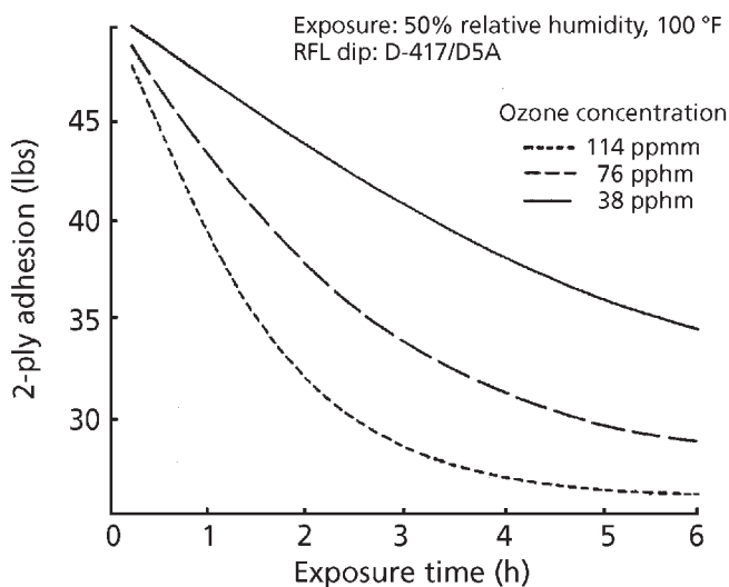
Figure 4.47 Influence of adhesion to exposure time to three ozone concentrations for polyester cords. pphm = parts per hundred million
