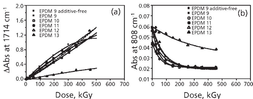
Figure 10.12 Increase in the absorbance at 1714\text{ cm}^{-1} (a) and decay in the absorbance at 808\text{ cm}^{-1} (b) as a function of the dose for various formulations of EPDM films \gamma -irradiated under an oxygen atmosphere
