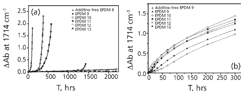
Figure 10.13 Increase in the absorbance at 1714 cm -1 as a function of thermooxidation duration at 100 °C (a) and as a function of photooxidation duration (b) for various formulations of EPDM films
