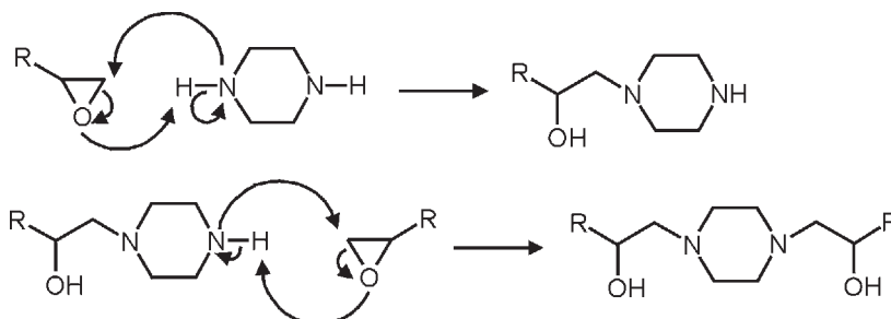
Figure 4.37 Maturing reaction of piperazine with two epoxy molecules
