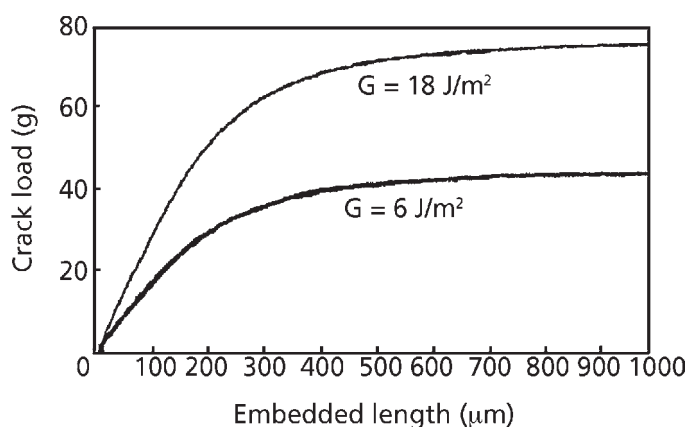
Figure 4.68 Load versus embedded length plots for different theoretical values for G_C
