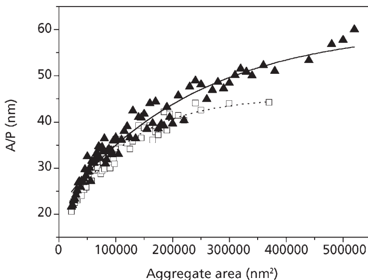
Figure 1.14 A/P ratio of aggregates in SBR-compounds loaded with 35 phr of filler as a function of their area: \blacktriangle \text{SiO}_2 ; \square TESPT- \text{SiO}_2
