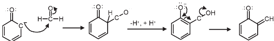
Figure 4.20 Reaction of phenol with formaldehyde
