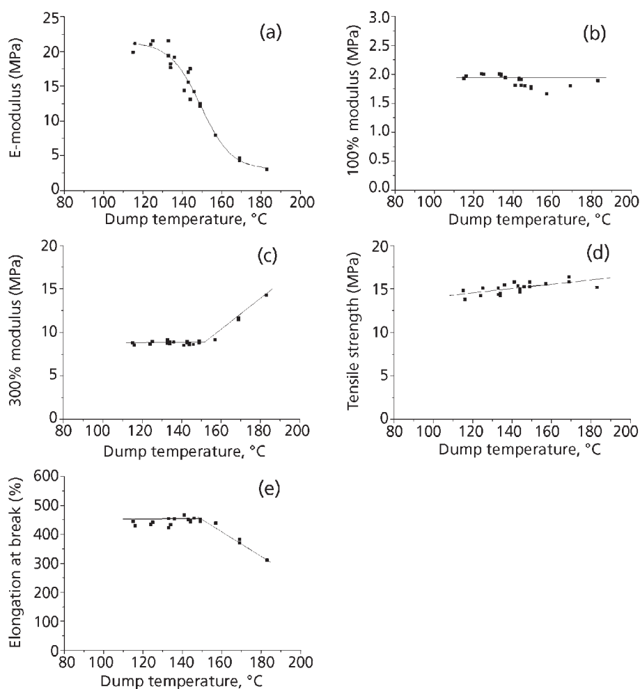
Figure 3.11 Tensile properties of cured compounds as a function of dump temperature.
