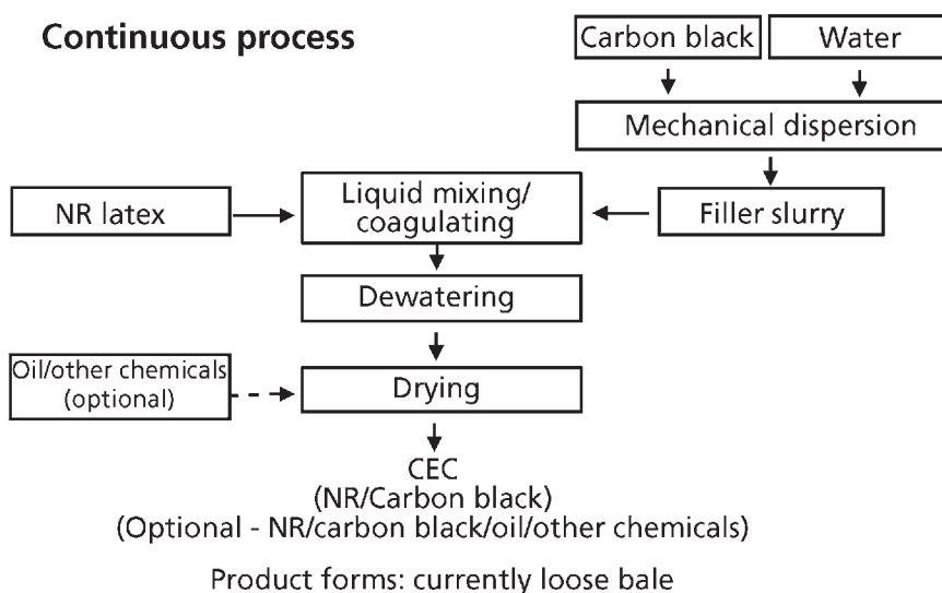
Figure 6.11 Flow diagram of the CEC process
