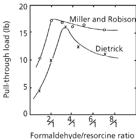
Figure 4.42 Effect of F/R ratio on the pull through load (Note: 1 lb load \equiv 4.448N force)
