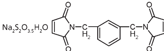
Figure 4.63 Structure of the thiosulfate and bismaleimide used
