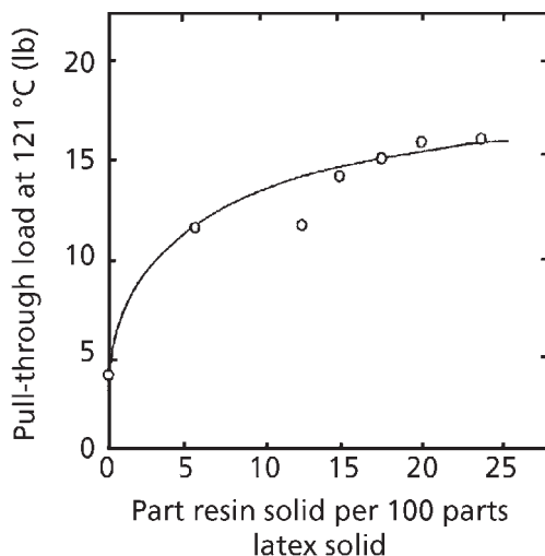
Figure 4.43 Pull through load versus RF/L ratio [14] (Note: 1 lb load \equiv 4.448N force)
