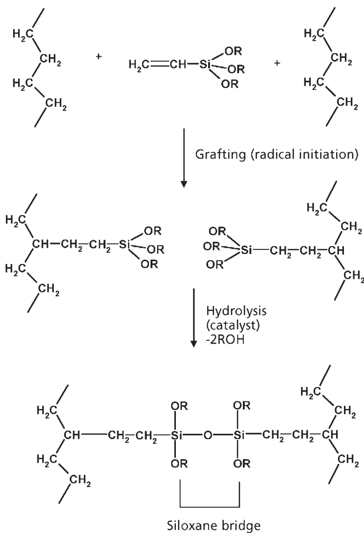
Figure 8.11 Crosslinking of polyethylene by Sioplas technique
