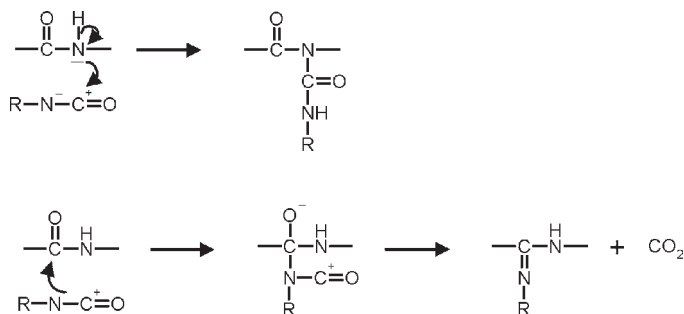
Figure 4.34 Probable mechanism for the two reactions of isocyanate with aramid
