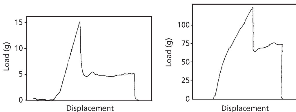
Figure 4.67 Load-displacements plots for fibre pullout tests for small embedded lengths (left) and large embedded lengths (right)
