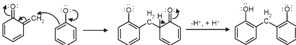
Figure 4.21 Bakelite formation
