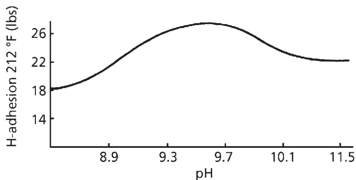
Figure 4.45 Value for the adhesion as a function of the pH when NaOH is used [54] (Note: 212 °F \equiv 100 °C; 1 lb load \equiv 4.448N force)
