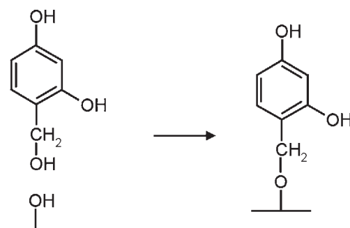
Figure 4.29 Reaction of the RF resin with the hydroxyl group of Rayon according to Moulst
