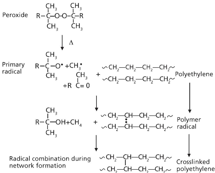
Figure 8.9 Peroxide curing of polyurethane
