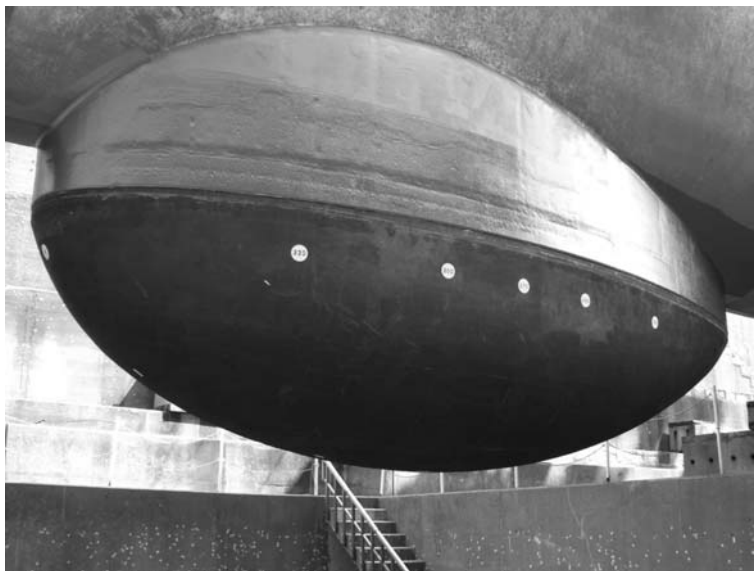
Figure 5.4 Composite keel dome composed of two resin-impregnated fibreglass outer layers and a soft rubber core. The geometry of the structure is tuned to be acoustically transparent over a limited frequency range
