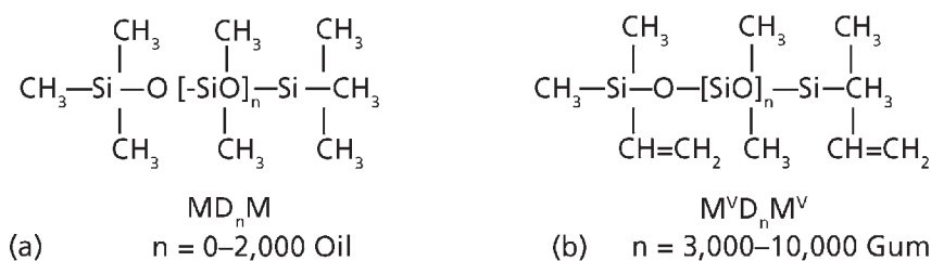
Figure 11.3 (a) Polydimethylsiloxane (MQ); (b) Polyvinylmethyilsiloxane (VMQ)
