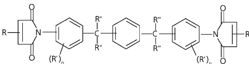
Aromatic bismaleimide
