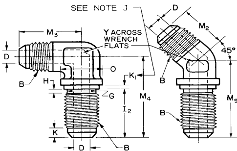
FIGURE 7A—90 DEGREE BULKHEAD ELBOW (070701)
