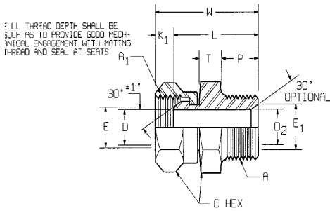
FIGURE 47A—FEMALE ADAPTER UNION TO MALE PIPE (140130)
