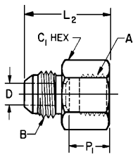
FIGURE 2D— FEMALE CONNECTOR (070103)
