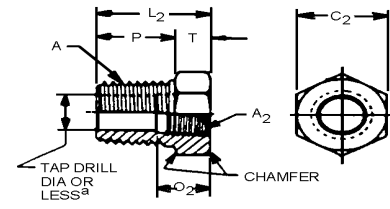
FIGURE 42—REDUCER BUSHINGS (140140)
