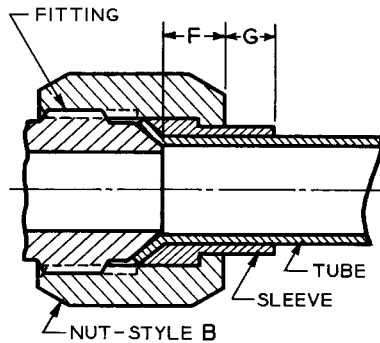
FIGURE 1A—THREE PIECE TUBE ASSEMBLY
