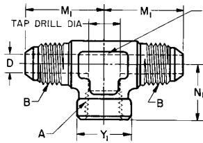
FIGURE 6A—FEMALE BRANCH TEE (070427)
