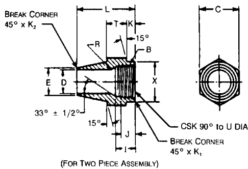
FIGURE 11—STYLE A NUT (070111)
