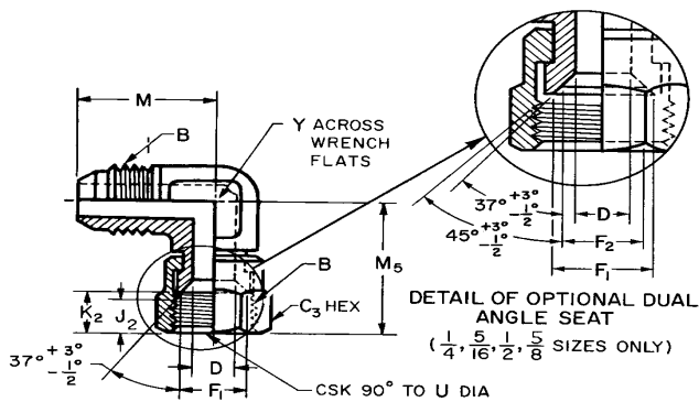
FIGURE 8C—90 DEGREE SWIVEL ELBOW (070221)
