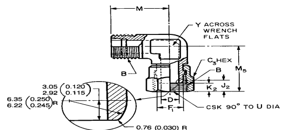
FIGURE 25C—90 DEGREE SWIVEL ELBOW (080221)
