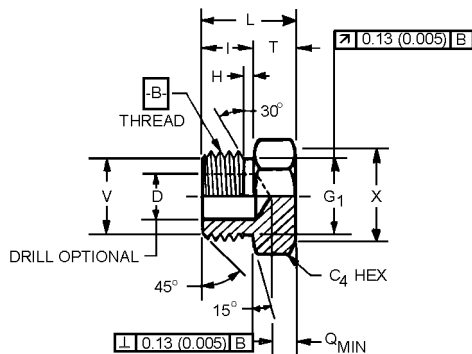
FIGURE 34A—HEXAGON HEAD O-RING BOSS PLUG (090109A)
