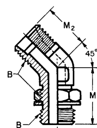
FIGURE 27B—45 DEGREE STRAIGHT THREAD ELBOW† (080320)
