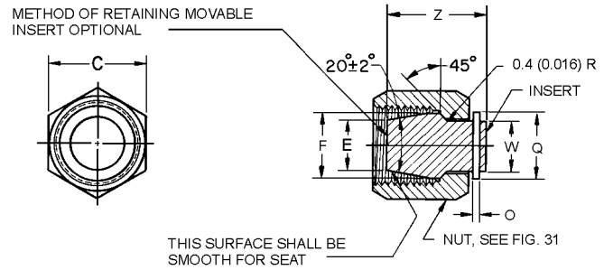
FIGURE 32—CAP ASSEMBLY (080112)
