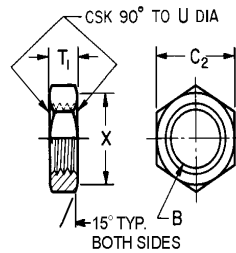
FIGURE 25B—BULKHEAD LOCKNUT (080118)
