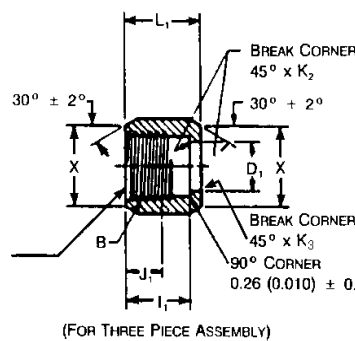
FIGURE 12—STYLE B NUT (070110)
