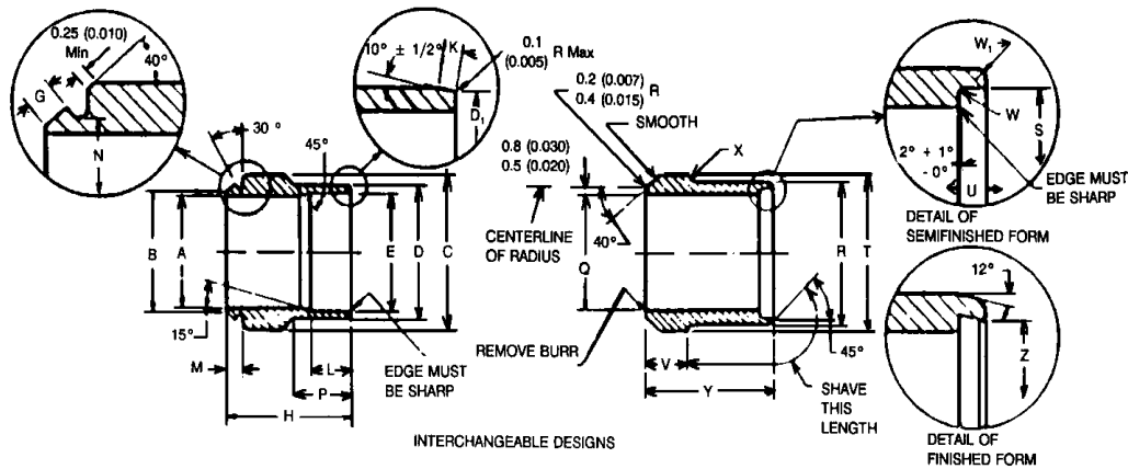
FIGURE 28—STYLE A FERRULE (080115A)
