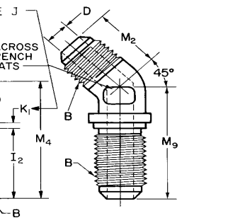
FIGURE 7B—45 DEGREE BULKHEAD ELBOW (070801)
