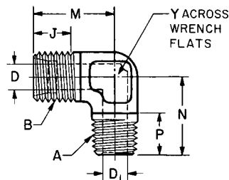
FIGURE 21A—90 DEGREE MALE ELBOW (080202)
