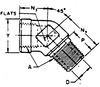
FIGURE 43D—45 DEGREE STREET ELBOW (140339)
