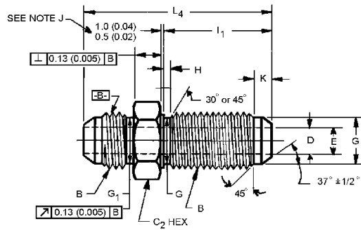
FIGURE 3A—BULKHEAD UNION (070601) SEE NOTE J
