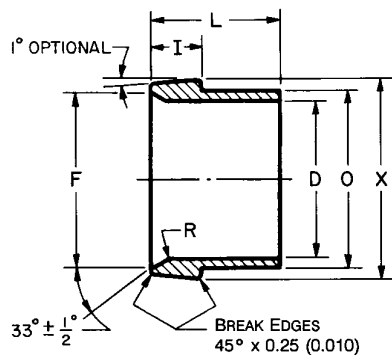
FIGURE 14—SLEEVE (070115)
