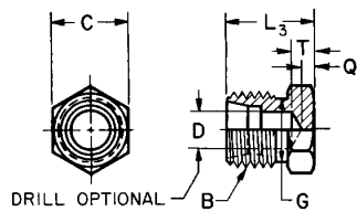
FIGURE 20D—PLUG (080109)
