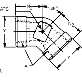
FIGURE 43B—45 DEGREE PIPE ELBOW (140338)
