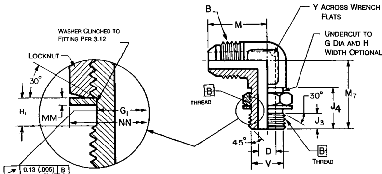
FIGURE 10A—90 DEGREE STRAIGHT THREAD ELBOW† (070220)
