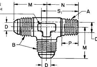
FIGURE 5C—MALE RUN TEE (070424)
