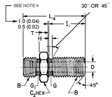
FIGURE 20A—BULKHEAD UNION (080601)
