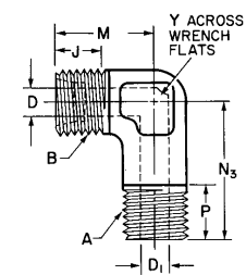
FIGURE 21B—90 DEGREE MALE LONG ELBOW (071502)
