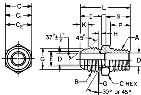
FIGURE 2A—MALE CONNECTOR (070102)
