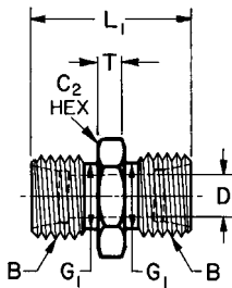
FIGURE 19C—LARGE HEX UNION* (080119)
