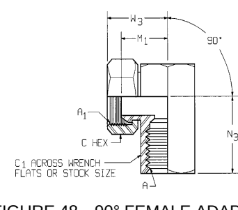
FIGURE 48—90° FEMALE ADAPTER UNION TO FEMALE PIPE (140231)
