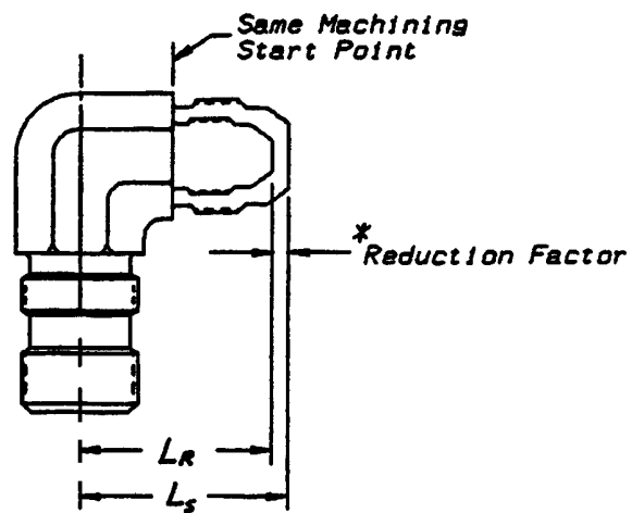
FIGURE 51A—JUMP SIZE CALCULATIONS—PORT SIZE
