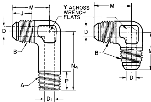
FIGURE 4C—90 DEGREE MALE EXTRA LONG ELBOW (071602)
