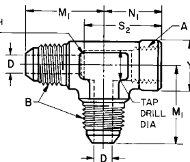
FIGURE 6B—FEMALE RUN TEE (070426)
