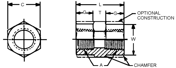
FIGURE 39—HEXAGON PIPE COUPLING (140138)
