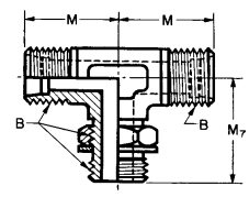
FIGURE 26D—STRAIGHT THREAD BRANCH TEE † (080429)
