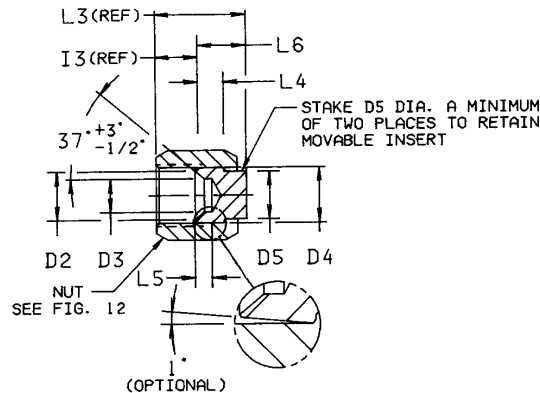
FIGURE 13A—CAP ASSEMBLY (MOVEABLE INSERT) (070112A)
