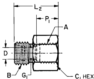
FIGURE 19D—FEMALE CONNECTOR (080103)
