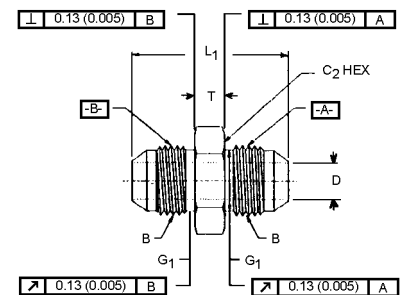
FIGURE 2C—LARGE HEX UNION* (070119)
