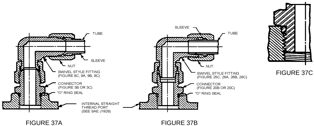
FIGURE 37—SWIVEL STYLE FITTINGS
