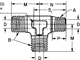
FIGURE 22C—MALE RUN TEE (080424)
