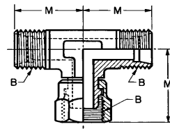
FIGURE 26C—SWIVEL BRANCH TEE (080433)
