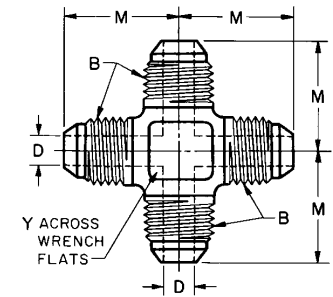
FIGURE 6C—CROSS (070501)
