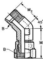
FIGURE 26A—45 DEGREE SWIVEL ELBOW (080321)
