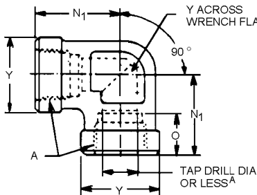
FIGURE 43A—90 DEGREE PIPE ELBOW (140238)
