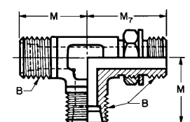
FIGURE 27C—STRAIGHT THREAD RUN TEE† (08428)
