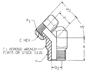
FIGURE 47B—45° FEMALE ADAPTER UNION TO MALE PIPE (140330)
