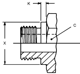
FIGURE 50—SMALLER NONADJUSTABLE STRAIGHT THREAD END
