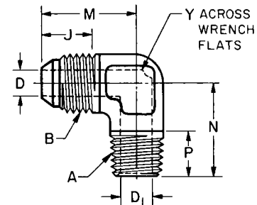
FIGURE 4A—90 DEGREE MALE ELBOW (070202)
