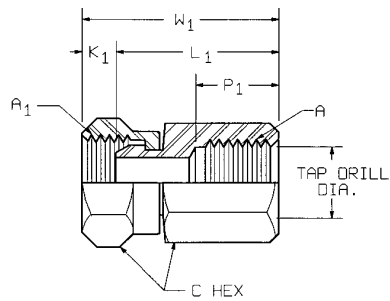
FIGURE 48A—FEMALE ADAPTER UNION TO FEMALE PIPE (140131)
