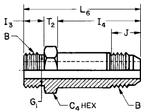
FIGURE 3C—STRAIGHT THREAD CONNECTOR LONG* (070122)
