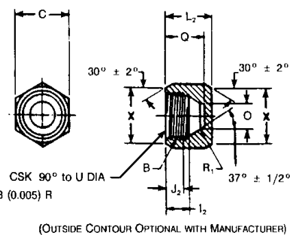
FIGURE 13—CAP (070112)
