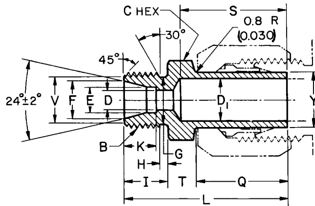
FIGURE 30—REDUCER (080123)
