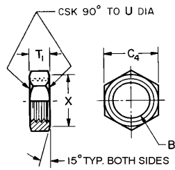
FIGURE 25A—STRAIGHT THREAD LOCKNUT* (080117)
