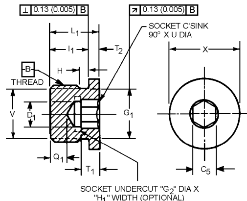
FIGURE 34B—HEXAGON SOCKET O-RING BOSS PLUG (090109B)
