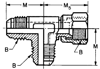
FIGURE 9B—SWIVEL RUN TEE (070432)
