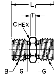
FIGURE 19B—UNION (080101)
