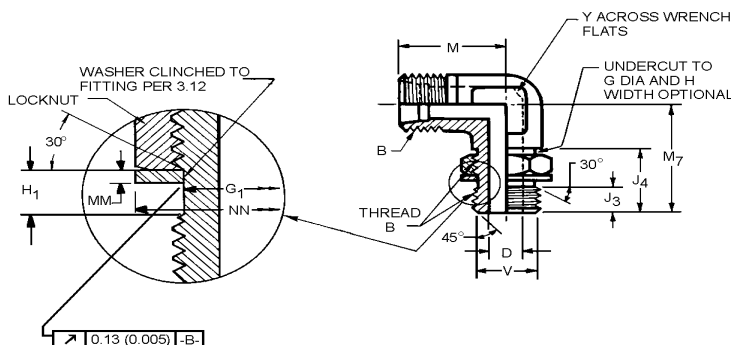
FIGURE 27A—90 DEGREE STRAIGHT THREAD ELBOW† (080220)
