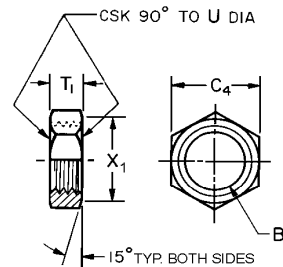
FIGURE 8A—STRAIGHT THREAD LOCKNUT* (070117)
