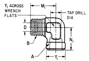
FIGURE 22A—90 DEGREE FEMALE ELBOW (080203)
