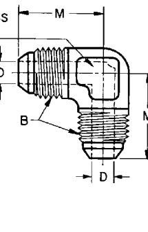
FIGURE 4D—90 DEGREE UNION ELBOW (070201)
