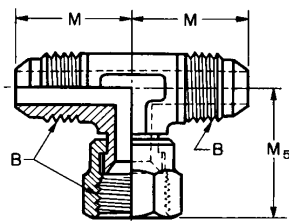
FIGURE 9C—SWIVEL BRANCH TEE (070433)
