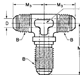
FIGURE 7C—BULKHEAD BRANCH TEE (070959)
