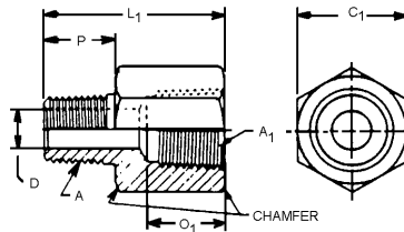
FIGURE 41—INCREASE ADAPTERS (140139)
