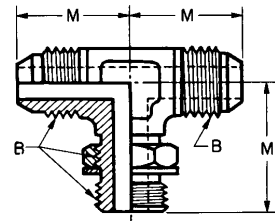
FIGURE 9D—STRAIGHT THREAD BRANCH TEE† (070429)
