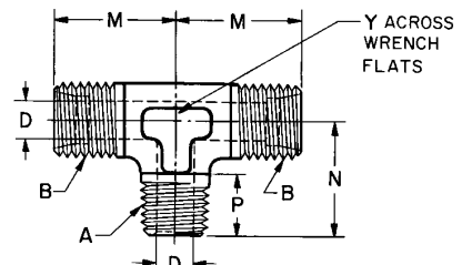
FIGURE 22D—MALE BRANCH TEE (080425)
