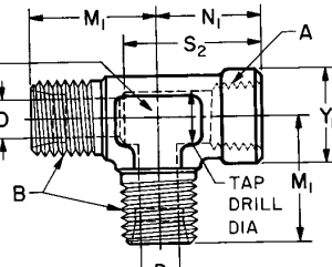
FIGURE 23B—FEMALE RUN TEE (080426)
