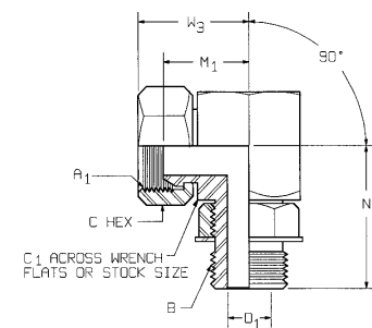
FIGURE 49C—90° FEMALE ADAPTER UNION TO ADJ. MALE STRAIGHT THREAD (140257)
