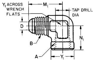
FIGURE 5A—90 DEGREE FEMALE ELBOW (070203)
