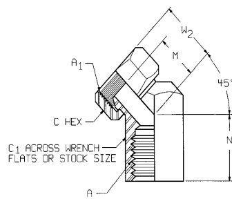
FIGURE 48B—45° FEMALE ADAPTER UNION TO FEMALE PIPE (140331)
