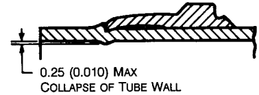
FIGURE 17—ENLARGED VIEW OF STYLE A FERRULE BITE
