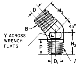
FIGURE 21E—45 DEGREE MALE ELBOW (080302)
