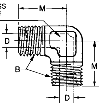
FIGURE 21C—90 DEGREE MALE EXTRA LONG ELBOW (081602)
