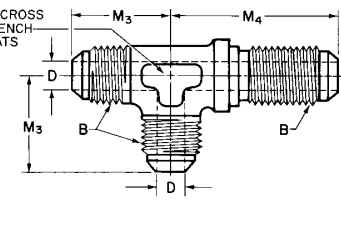
FIGURE 7D—BULKHEAD RUN TEE (070958)
