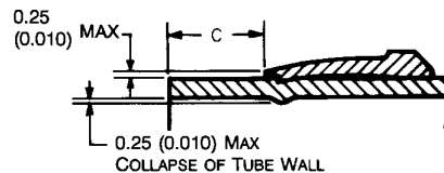
FIGURE 18—ENLARGED VIEW OF STYLE B FERRULE BITE
