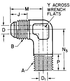
FIGURE 4B—90 DEGREE MALE LONG ELBOW (071502)
