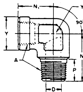
FIGURE 43C—90 DEGREE STREET ELBOW (140239)
