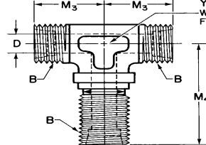
FIGURE 24C—BULKHEAD BRANCH TEE (080959)
