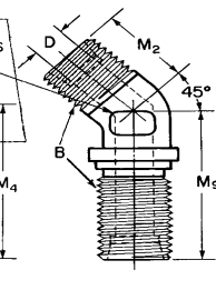
FIGURE 24B—45 DEGREE BULKHEAD ELBOW (080801)
