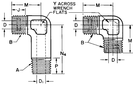
FIGURE 21C—90 DEGREE MALE EXTRA LONG ELBOW (081602)
