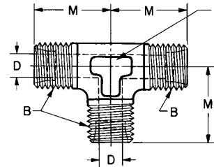
FIGURE 22B—UNION TEE (080401)
