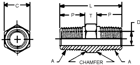
FIGURE 38—HEXAGON PIPE NIPPLE (140137)
