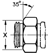
FIGURE 35—MODIFIED HEXAGON CHAMBER
