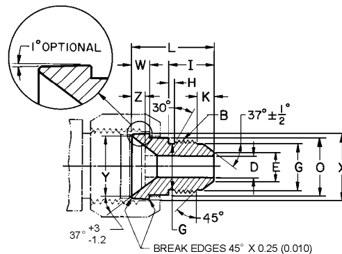
FIGURE 15—REDUCING ADAPTER (070123)
