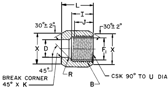
FIGURE 31—NUT (080110)
