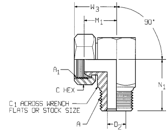
FIGURE 47C—90° FEMALE ADAPTER UNION TO MALE PIPE (140230)
