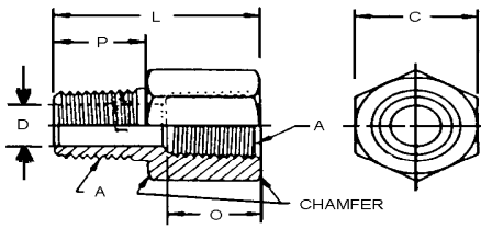
FIGURE 40—ADAPTER (140139)
