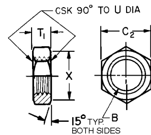
FIGURE 8B—BULKHEAD LOCKNUT (070118)
