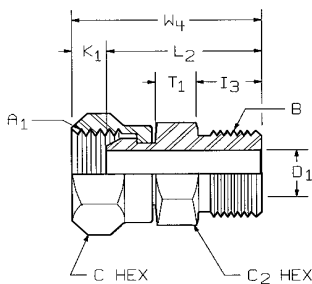
FIGURE 49A—FEMALE ADAPTER UNION TO MALE STRAIGHT THREAD (140157)
