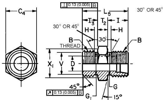
FIGURE 20B—STRAIGHT THREAD CONNECTOR SHORT* (080120)
