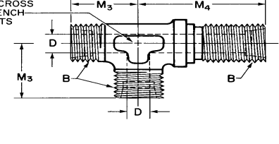
FIGURE 24D—BULKHEAD RUN TEE (080958)
