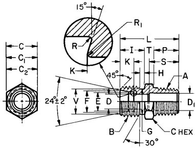
FIGURE 19A—MALE CONNECTOR (080102)
