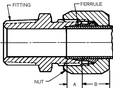
FIGURE 16A—ASSEMBLY WITH STYLE A FERRULE (FIGURE 28)
