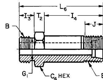
FIGURE 20C—STRAIGHT THREAD CONNECTOR LONG* (080122)
