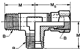
FIGURE 26B—SWIVEL RUN TEE (080432)
