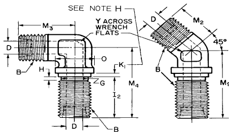
FIGURE 24A—90 DEGREE BULKHEAD ELBOW (080701)
