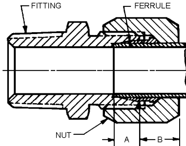
FIGURE 16B—ASSEMBLY WITH STYLE B FERRULE (FIGURE 29)
