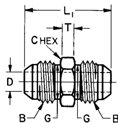
FIGURE 2B—UNION (070101)
