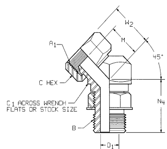
FIGURE 49B—45° FEMALE ADAPTER UNION TO ADJ. MALE STRAIGHT THREAD (140357)
