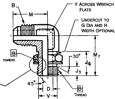
FIGURE 10B—45 DEGREE STRAIGHT THREAD ELBOW† (070320)
