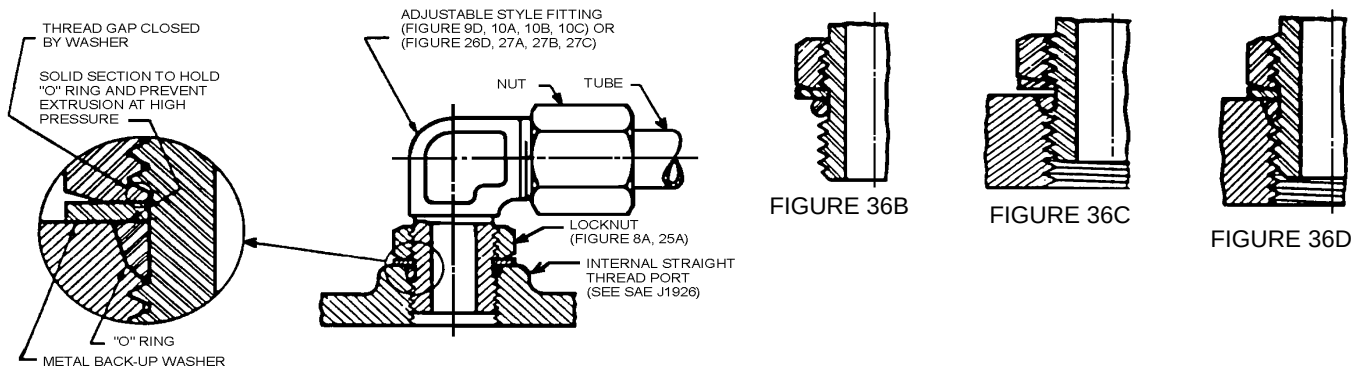
FIGURE 36A FIGURE 36—ADJUSTABLE STYLE FITTINGS
