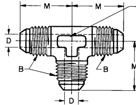
FIGURE 5B—UNION TEE (070401)
