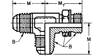
FIGURE 10C—STRAIGHT THREAD RUN TEE† (070428)
