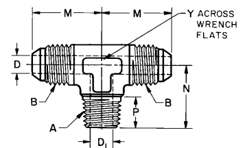
FIGURE 5D—MALE BRANCH TEE (070425)
