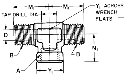
FIGURE 23A—FEMALE BRANCH TEE (080427)
