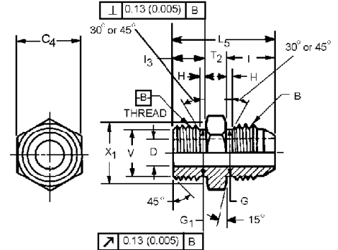
FIGURE 3B—STRAIGHT THREAD CONNECTOR SHORT* (070120)
