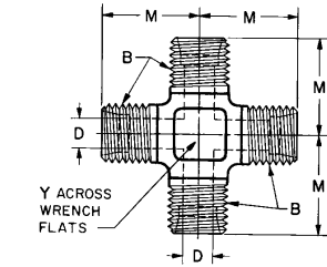
FIGURE 23—CROSS (080501)
