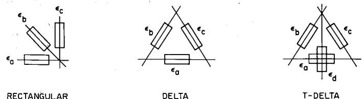
FIGURE 2—RECTANGULAR, DELTA, AND T-DELTA ROSETTES
