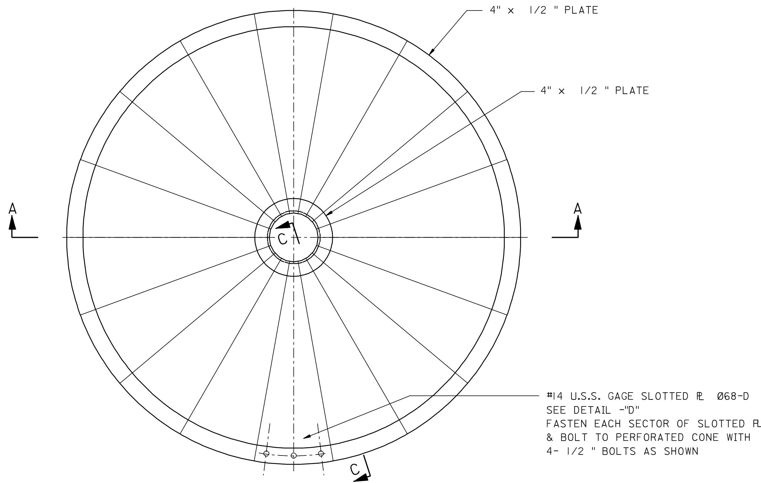
ASSEMBLY OF SLOTTED PLATES
