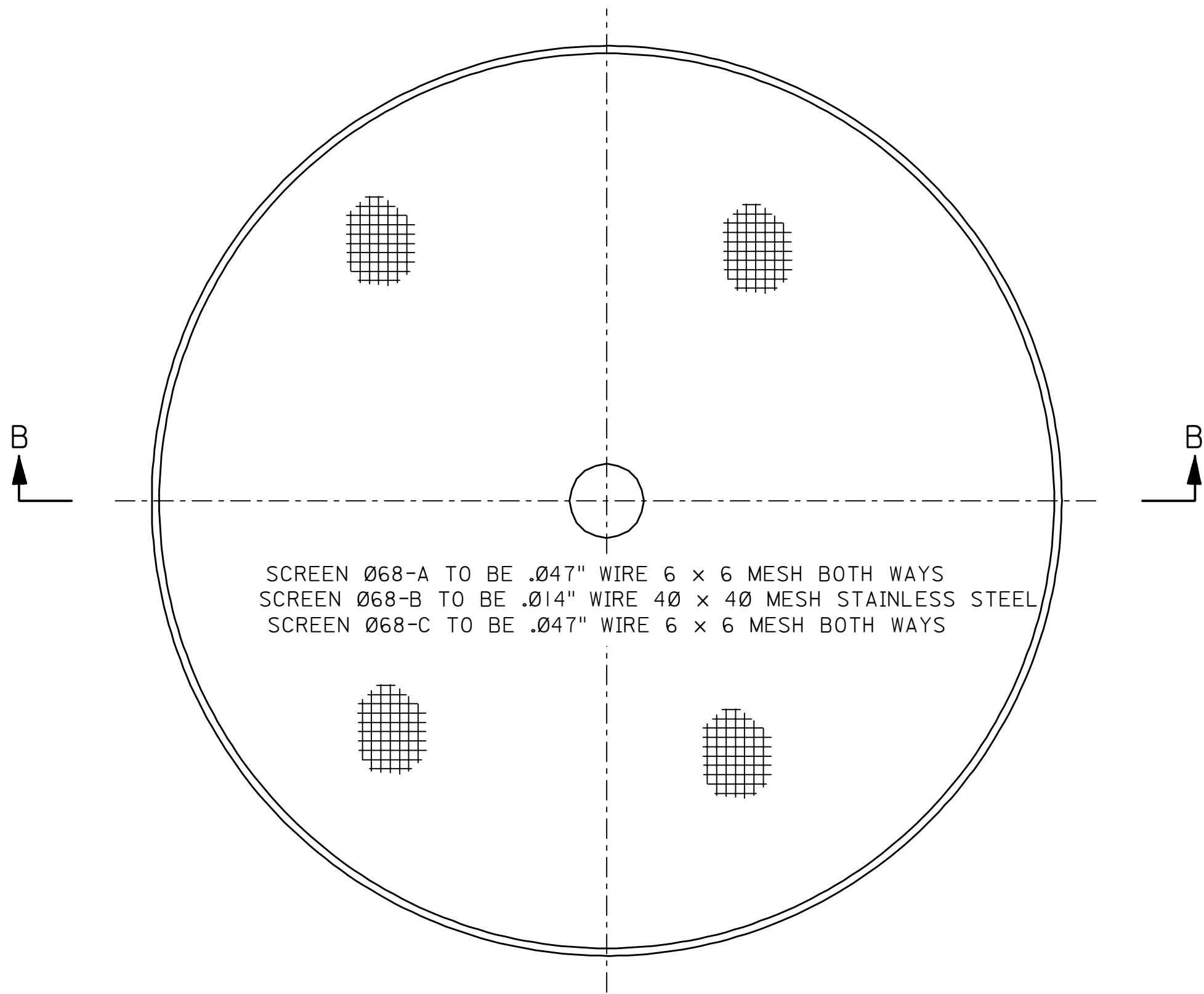
PLAN OF SCREEN
