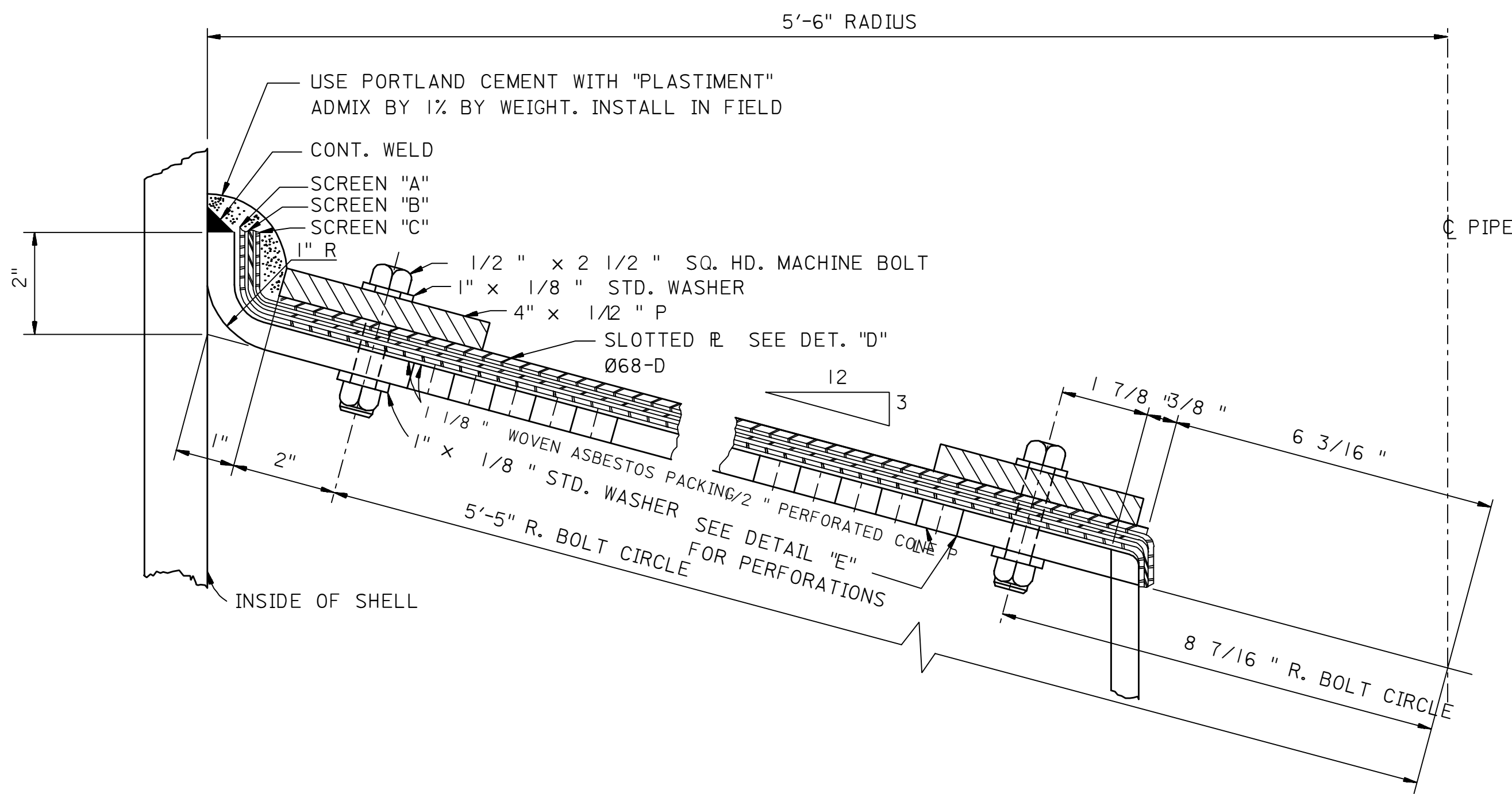
SECTION C-C ASSEMBLY OF SCREENS
