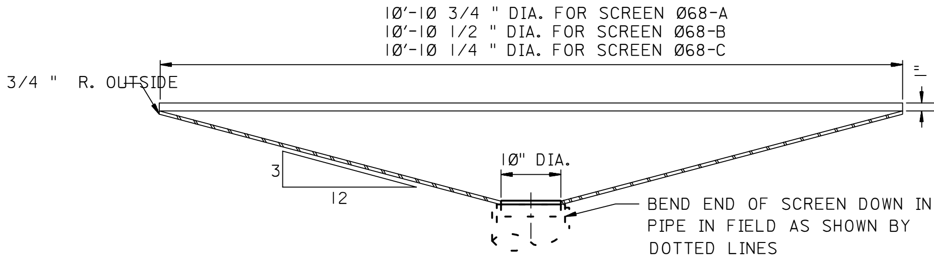
SECTION B-B
