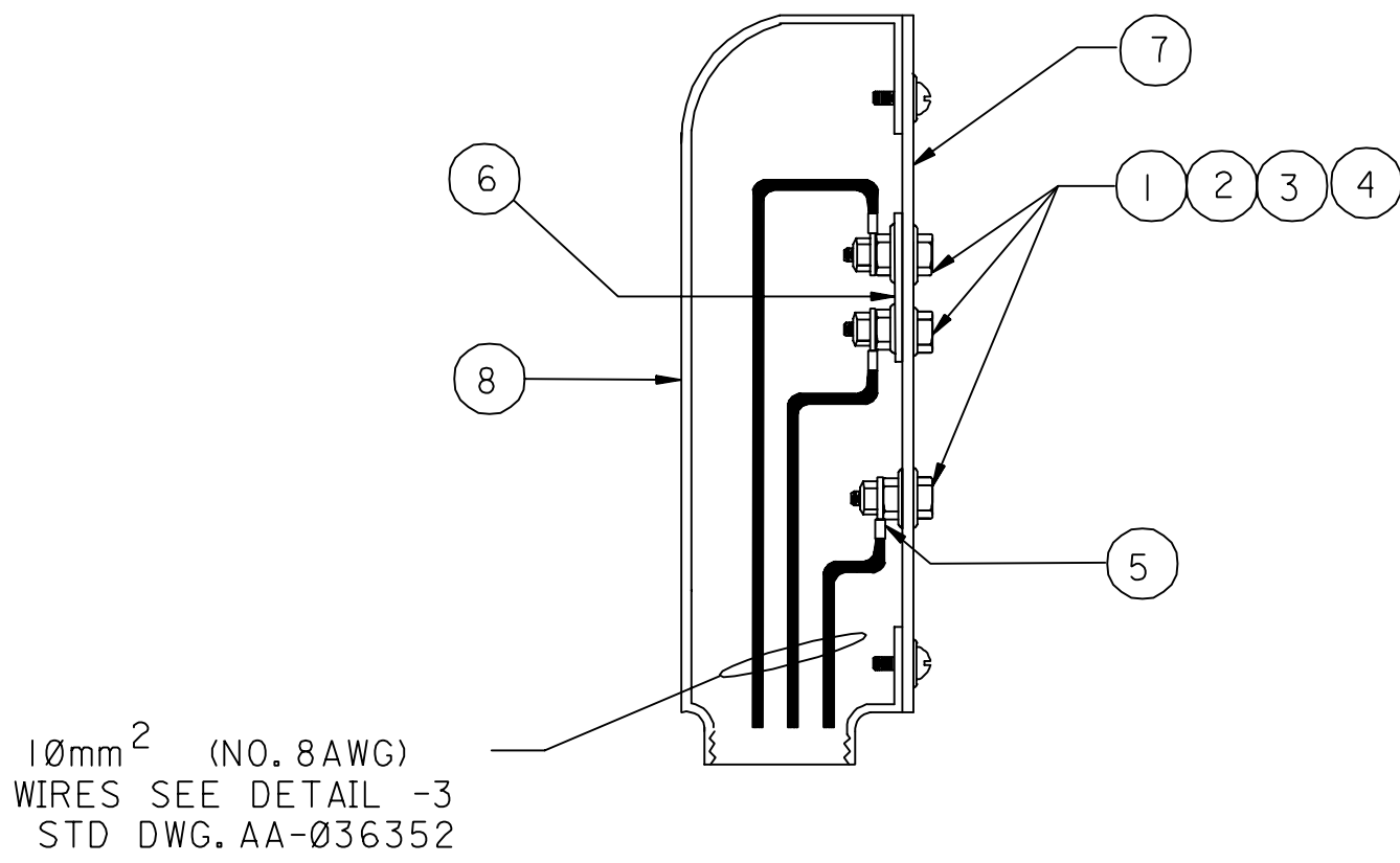
GALVANIC ANODE 3-PIN TEST STATION
