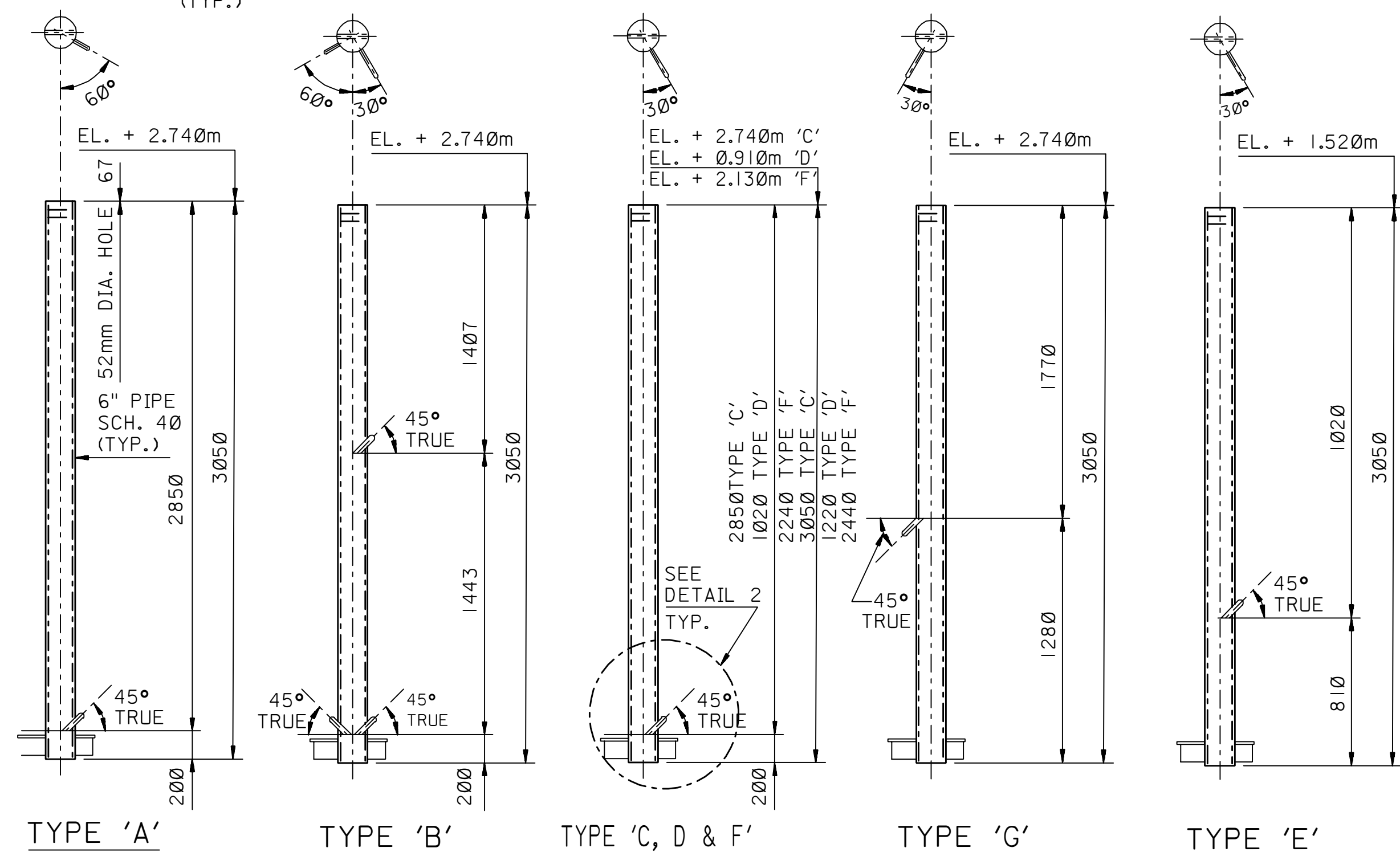
LOCATION OF HOOKS ON HANGERS
