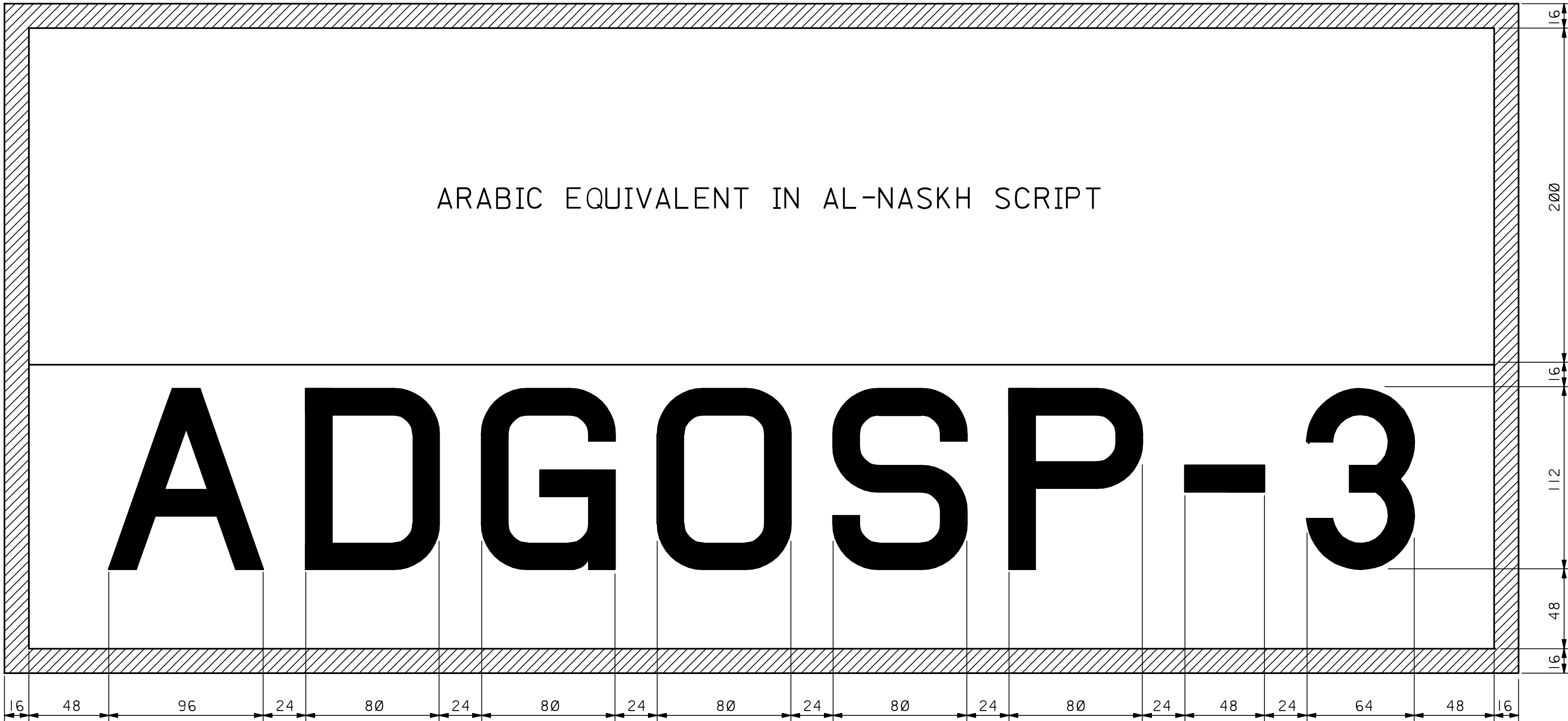
EXAMPLE OF SIGN-PLATE AND LETTERING DIMENSIONS FOR AIN DAR GOSP-3 ALL DIMENSIONS ARE IN MILLIMETERS ( TOLERANCE ± 10% )
