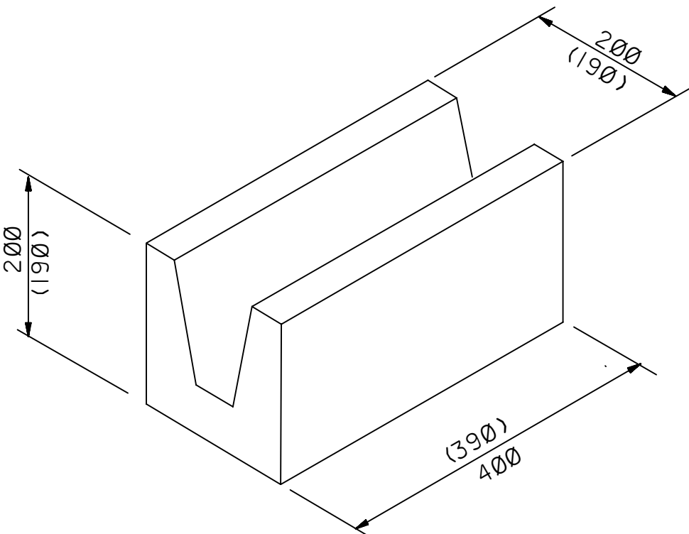
BOND BEAM
