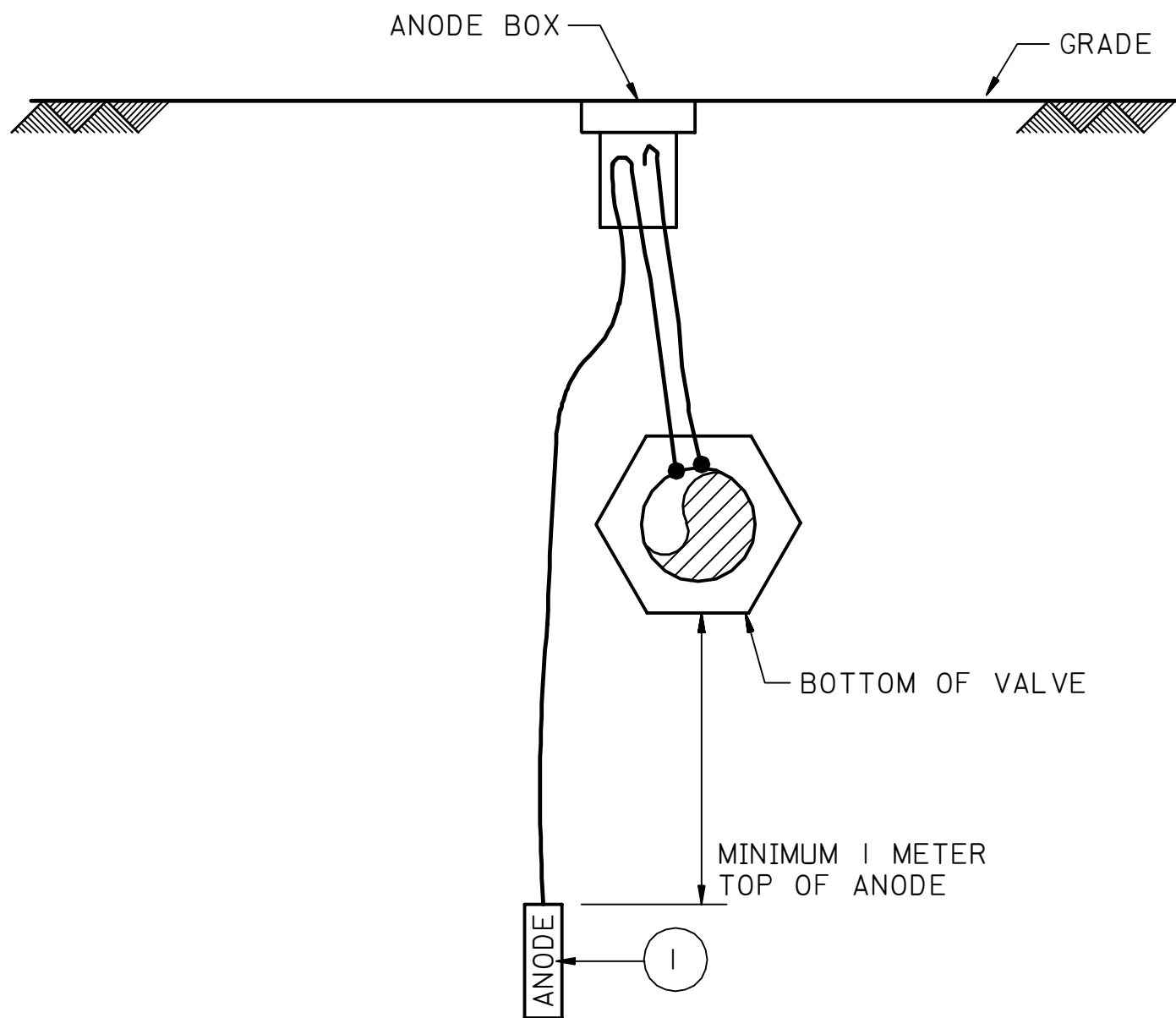
DETAIL-5
