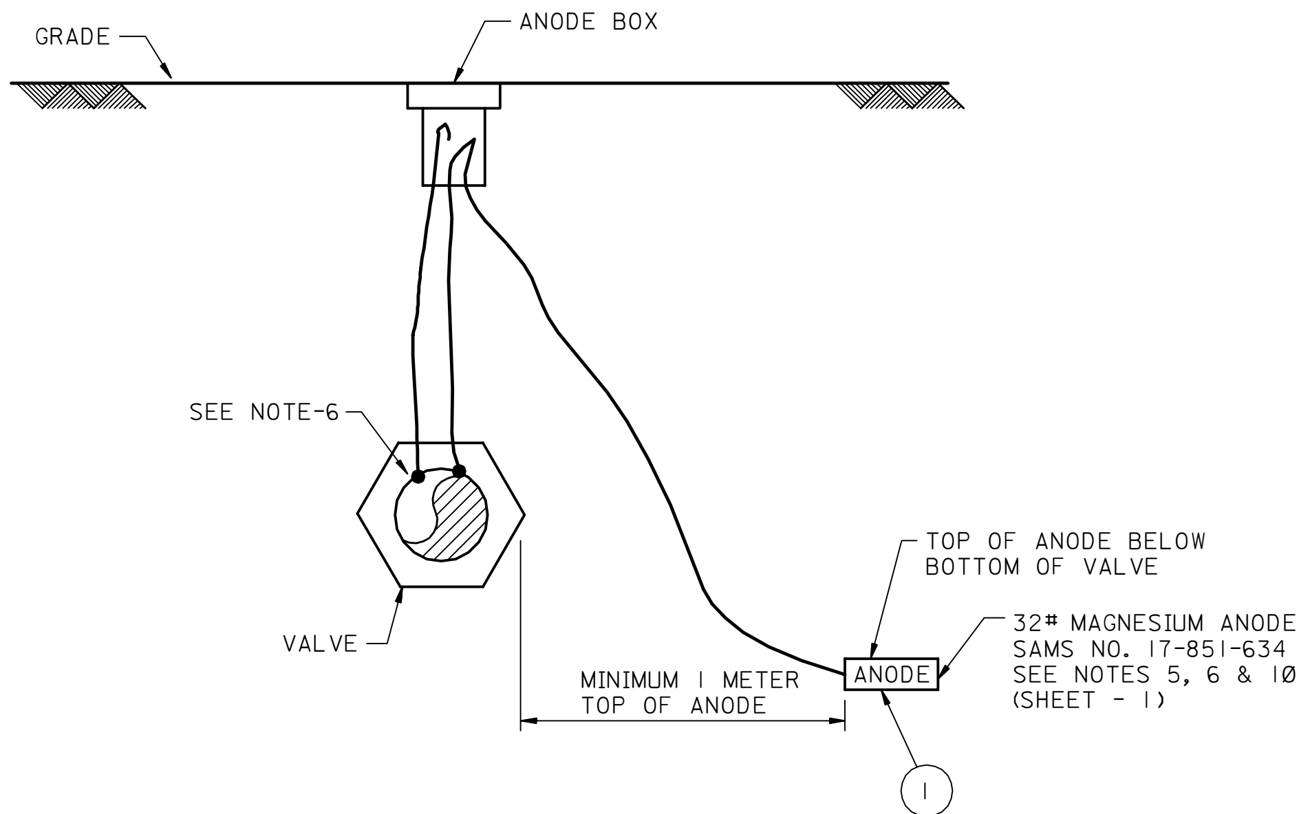
DETAIL-6
