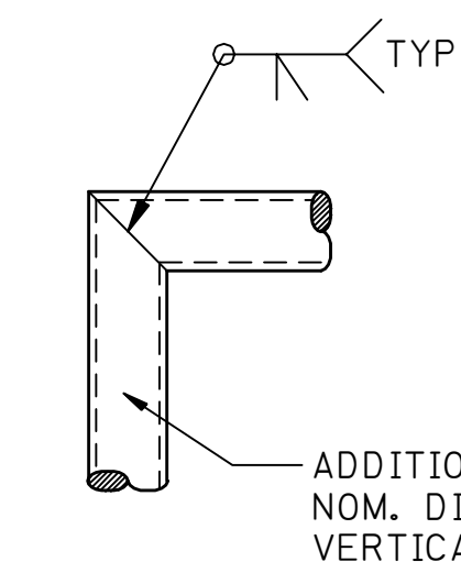
K VIEW - SCALE 1 : 5
