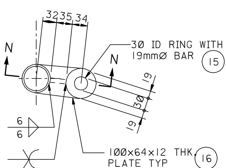
DETAIL SCALE 1 : 5
