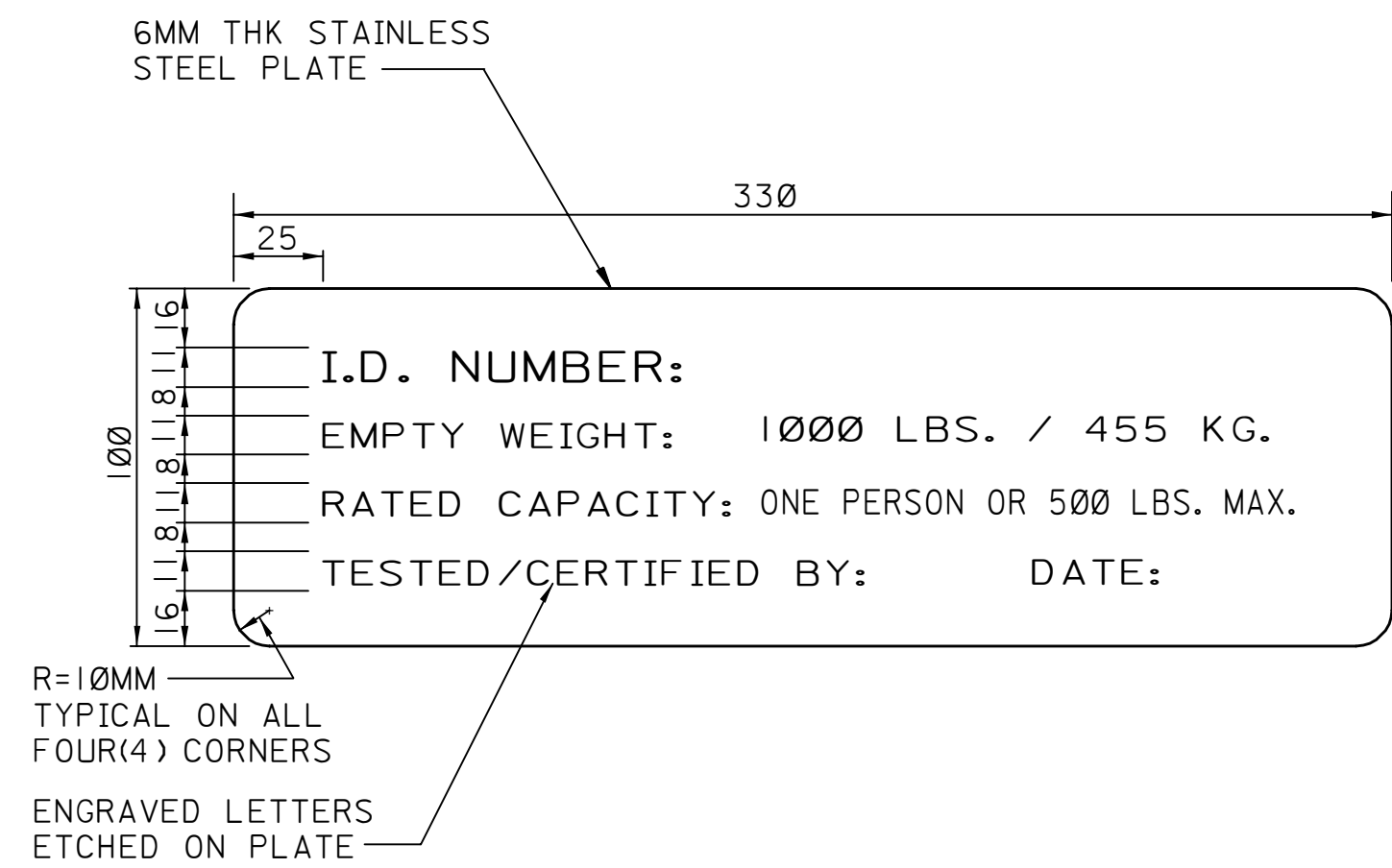
2 IDENTIFICATION PLATE DETAIL - NOT TO SCALE
