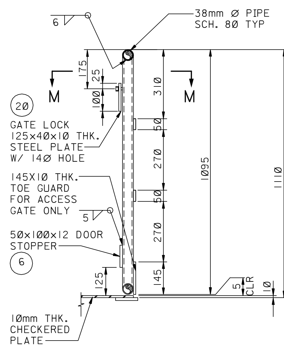
L SECTION @ GATE 145.2 SCALE 1 : 10
