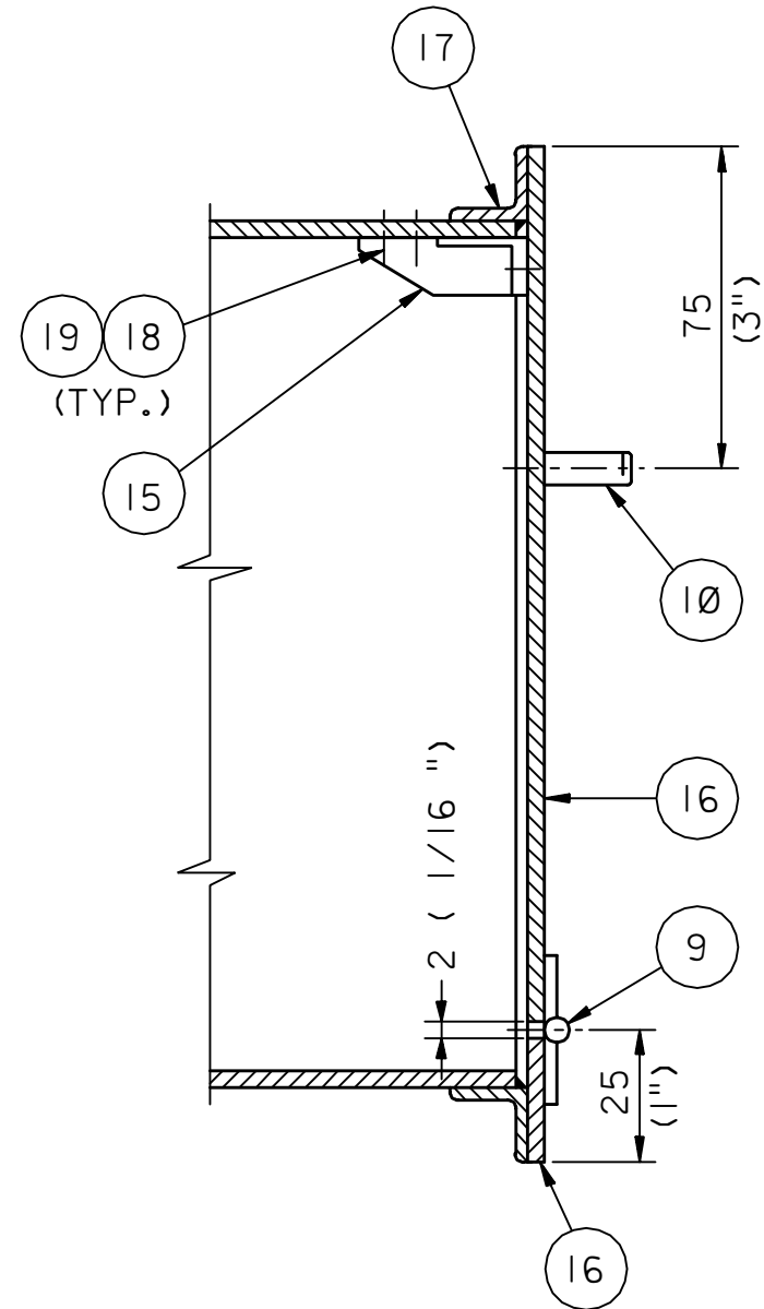
DETAIL-2
