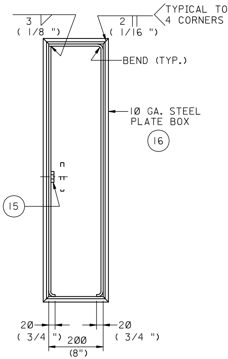
SECTION C-C
