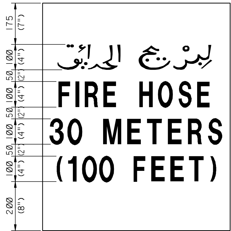
DETAIL-3
