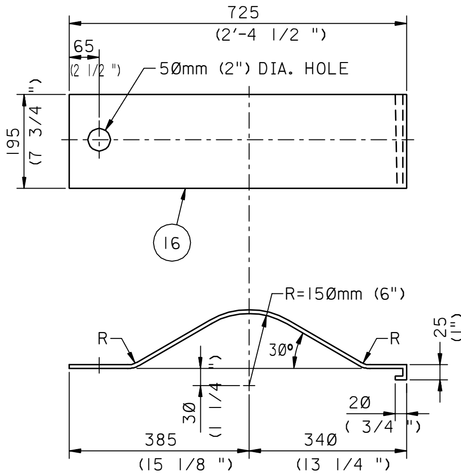
DETAIL-1
