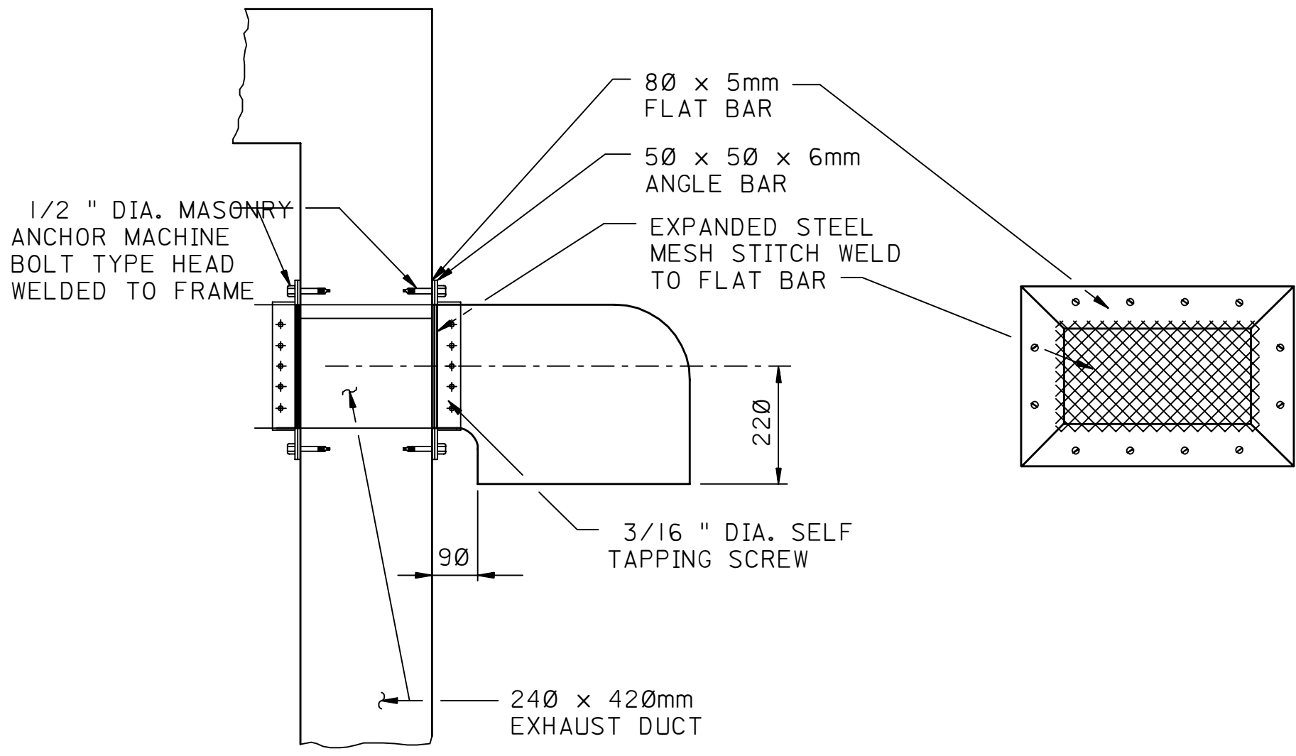
DETAIL 2 EXHAUST DUCT
