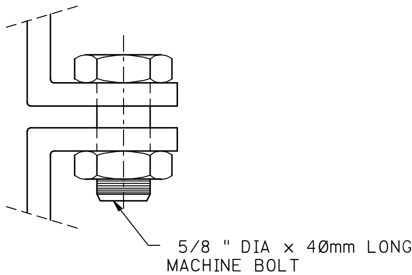
DETAL 5 MACHINE BOLT
