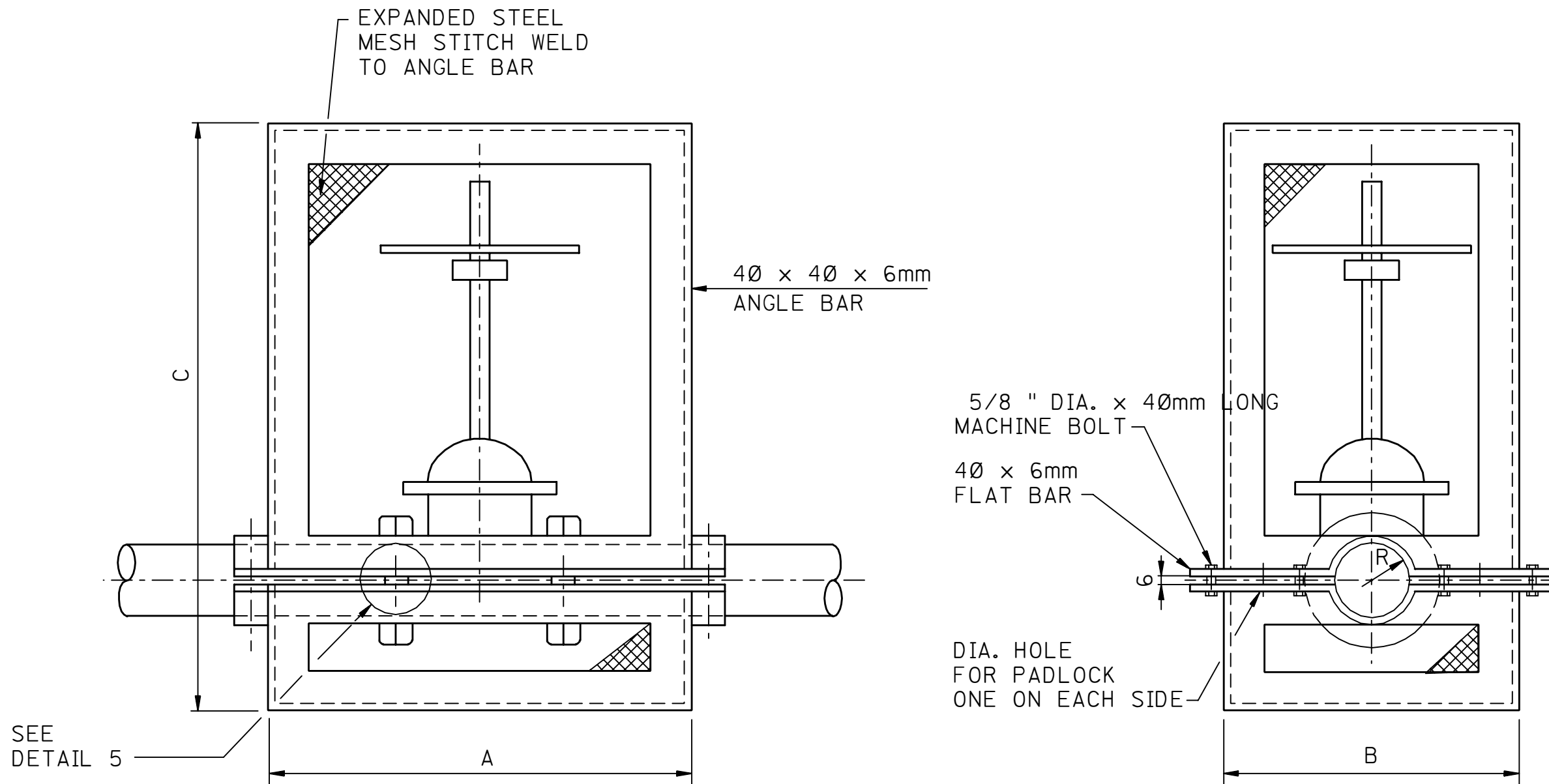
DETAIL 3 GENERAL OPENING
