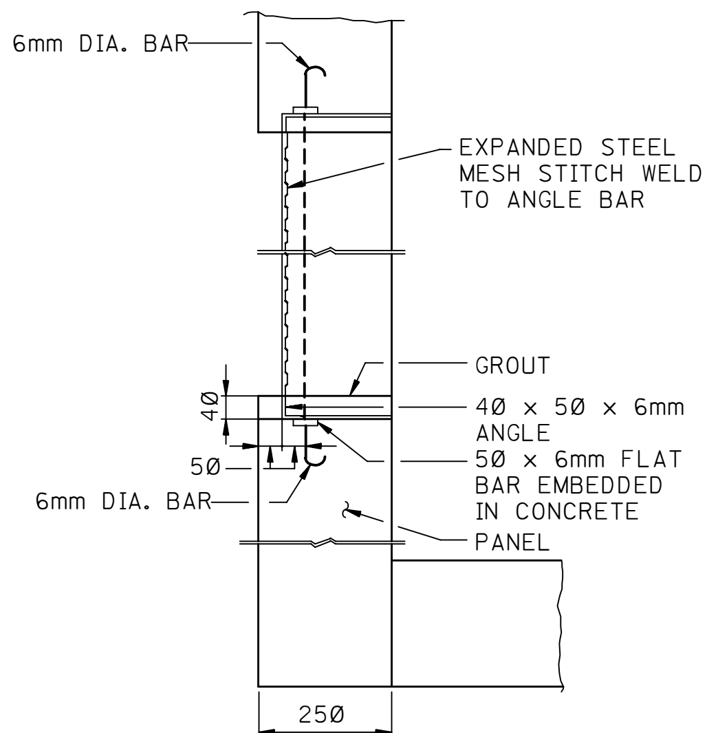
DETAIL 3 GENERAL OPENING
