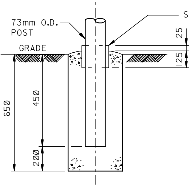
CORNER AND GATE POSTS
