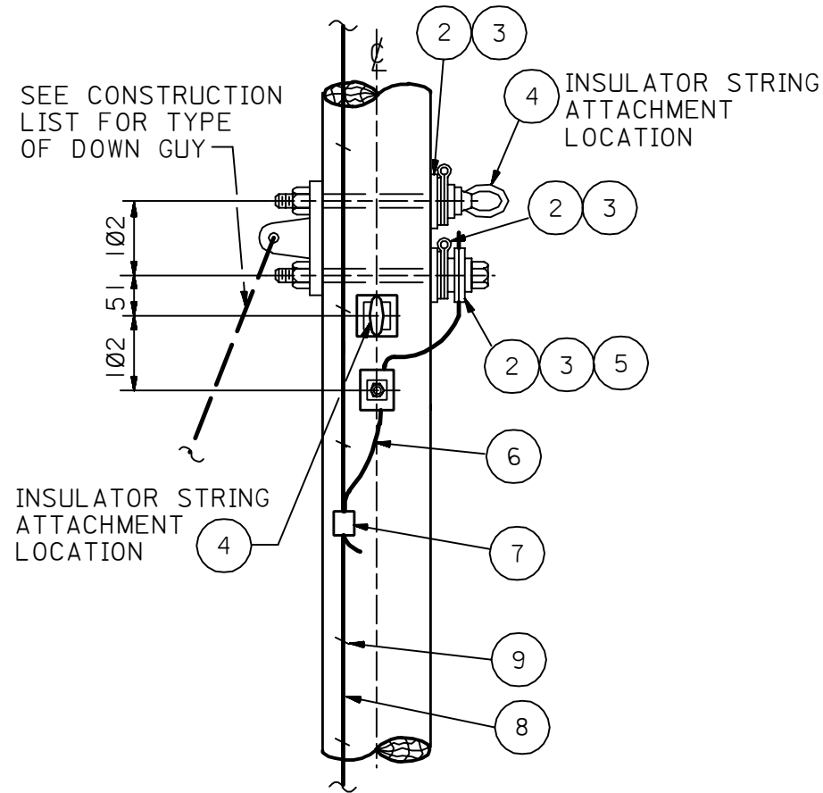
FIGURE-1 BONDING DETAIL AT GUYED PHASE POSITION
