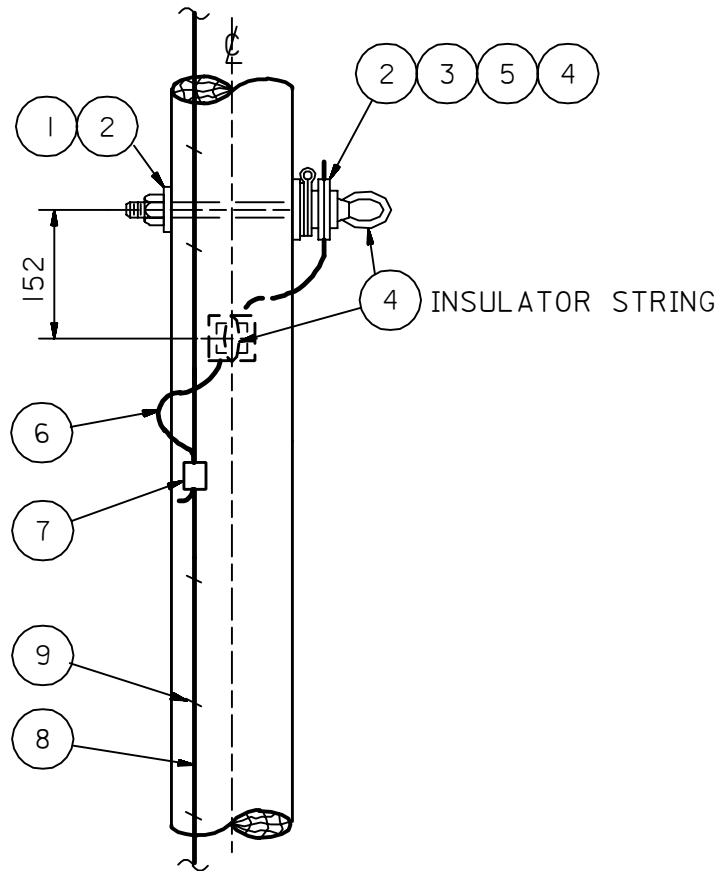
FIGURE-2 BONDING DETAIL AT UN-GUYED PHASE POSITION
