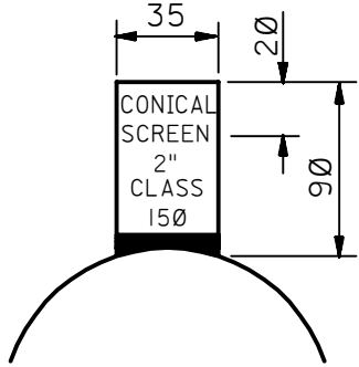
TYPICAL EXTENSION FOR IDENTIFICATION DETAIL-I
