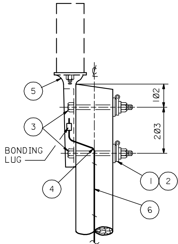
FIGURE-1 POLE TOP LINE POST INSULATOR INSTALLATION
