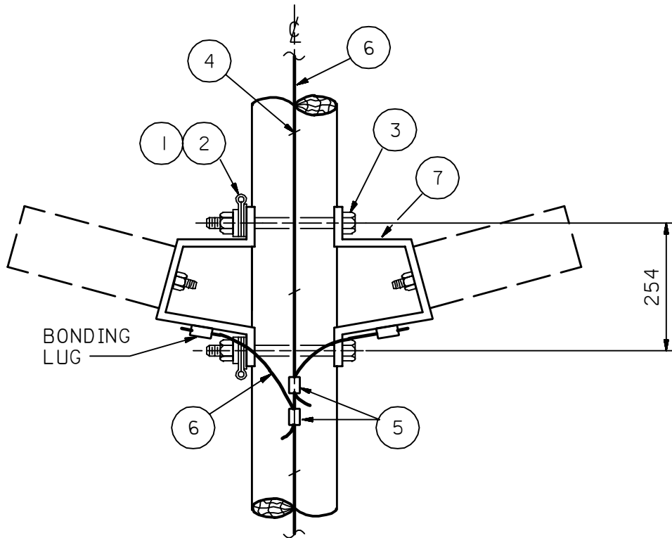
FIGURE-2 HORIZONTAL LINE POST INSULATOR INSTALLATION
