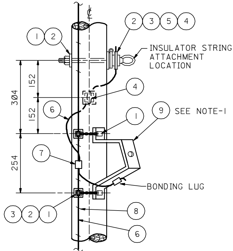
FIGURE-2 BONDING DETAIL AT UN-GUYED PHASE POSITION
