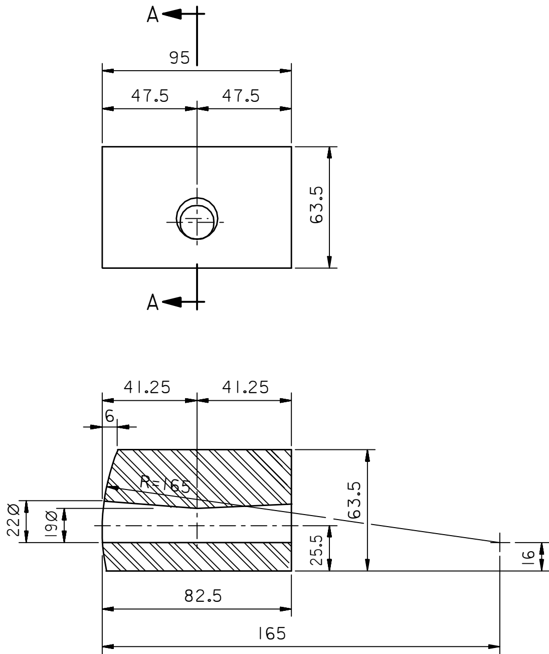
SECTION "A-A"
