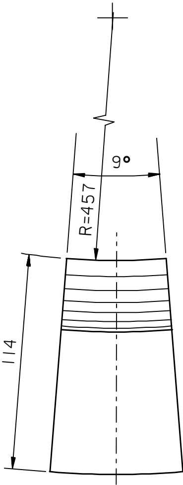
VIEW "A-A"
