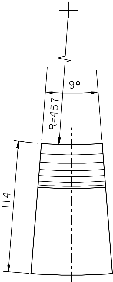
VIEW "A-A"
