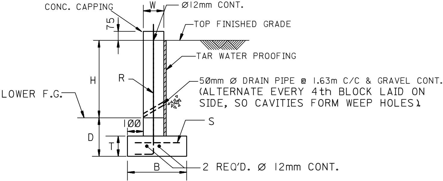
CONCRETE BLOCK RETAINING WALLS & PLANTING BOXES
