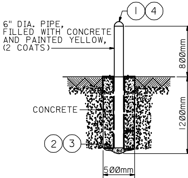
GUARD DETAIL
