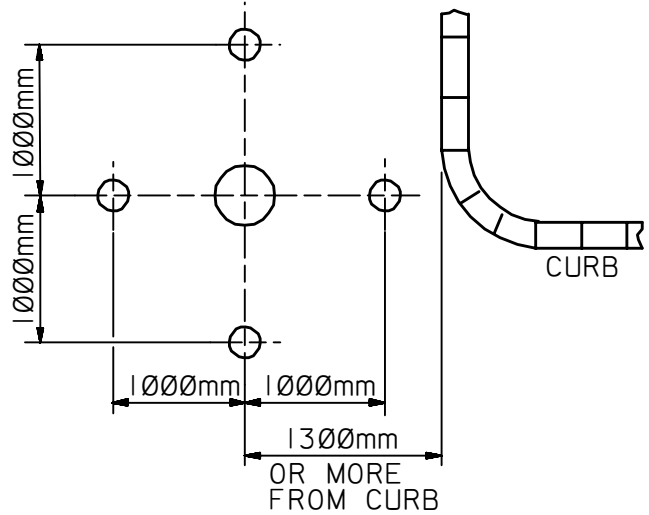
PLAN "B"
